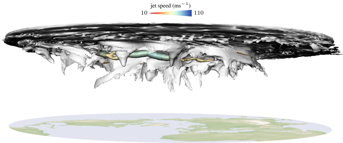
(c) Polar stereographic projection at 03.09.2016 18:00.
