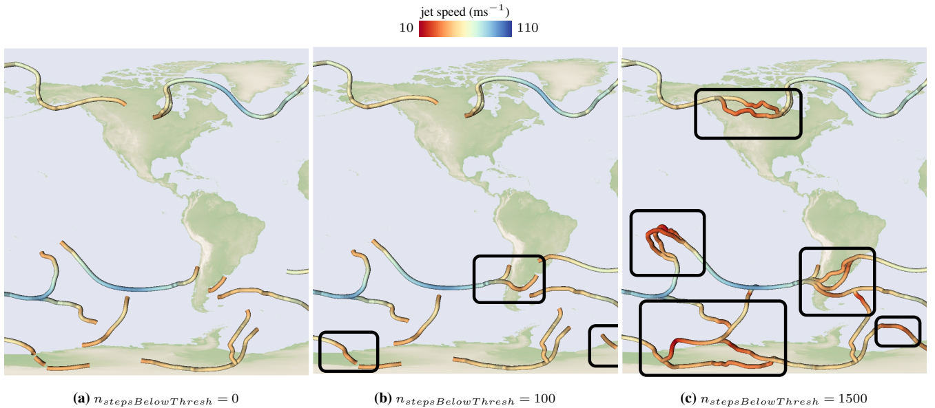
Figure 5. Increasing the number of prediction steps a jet core might remain below the wind magnitude threshold, results in longer connected jet corelines. Here, for 11.09.2016 15:00.
