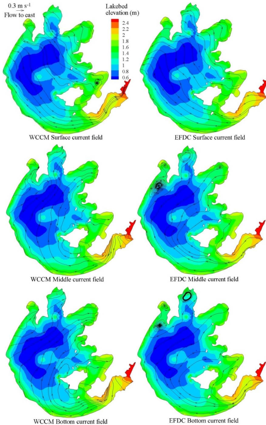
Figure B.3. Comparison of the flow fields and stream traces in the surface, middle, and bottom layers of Lake Taihu simulated by the WCCM and EFDC at 12:00 on August 10, 2015
