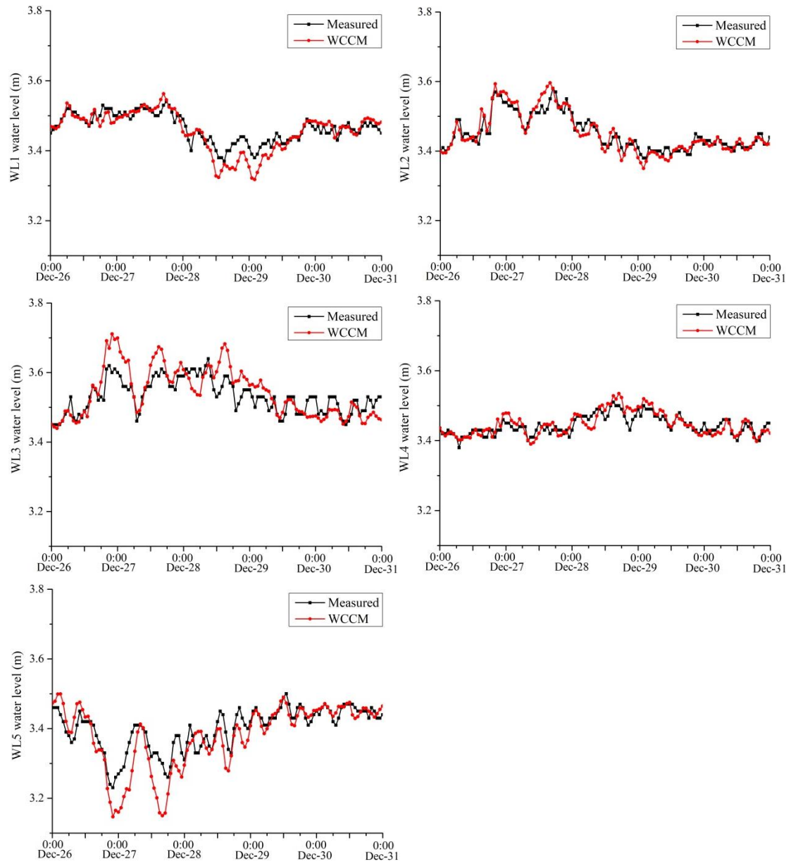
Figure 10. Comparison between the WCCM-simulated and measured water levels at the WL1–WL5 stations during the 2018 winter observation.
