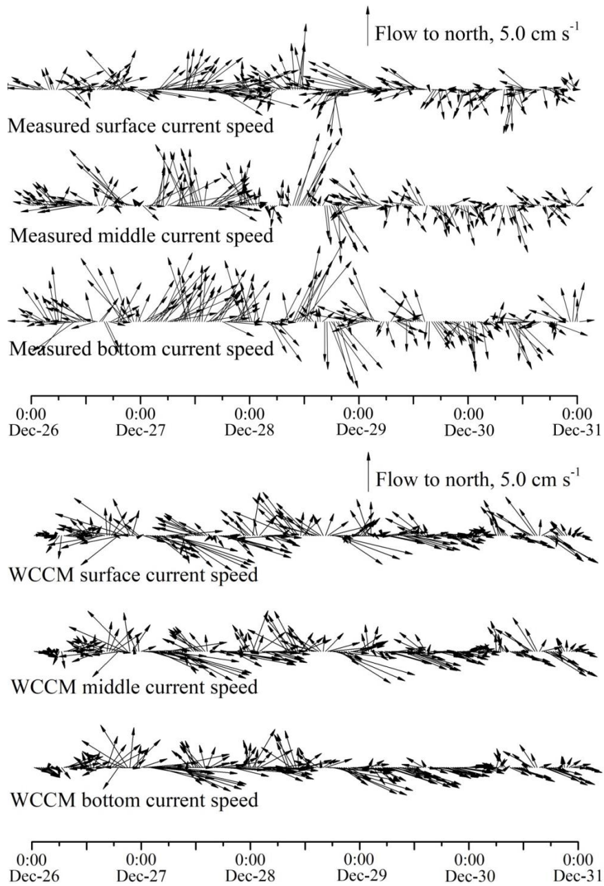
Figure 11. Comparison between the measured and WCCM-simulated surface, middle, or bottom current speeds at the LHWS during the 2018 winter observation.
