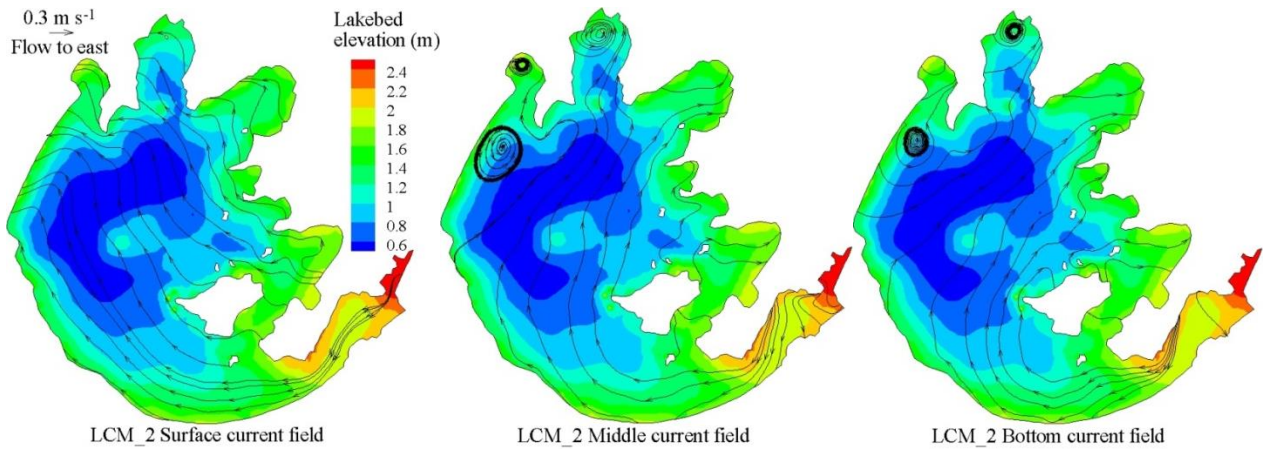
980 Figure B.5. Comparison of the LCM_2-simulated streamtraces of the surface, middle, and bottom current fields in Lake Taihu at 12:00 on August 10, 2015
