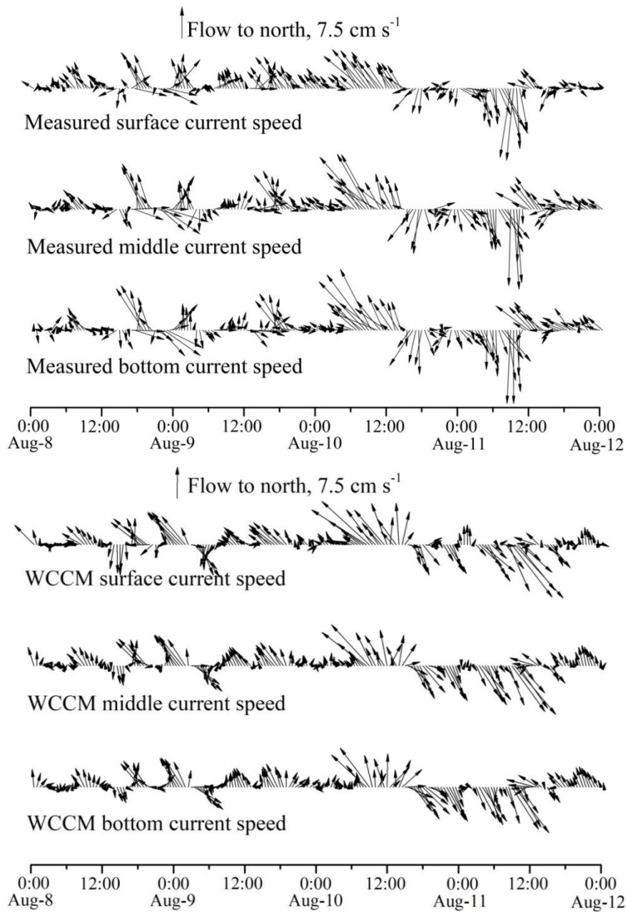
800 Figure 7. Comparison between the measured and WCCM-simulated current speeds in the lake surface, middle, and bottom water layer at the LHWS during the 2015 summer observation.
