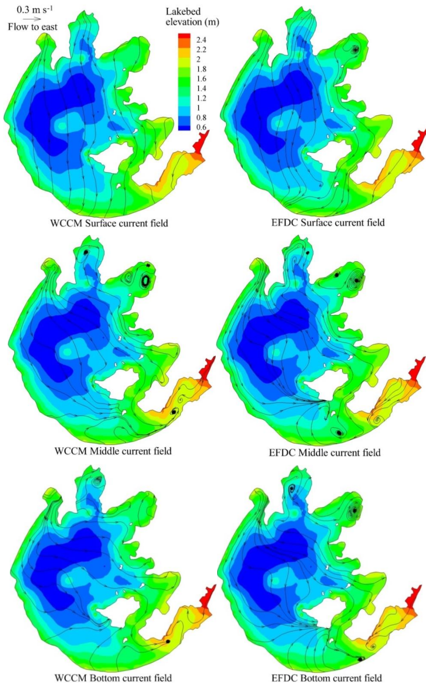
Figure B.4. Comparison of the flow fields and stream traces in the surface, middle, and bottom layers of Lake Taihu simulated by the WCCM and EFDC at 22:00 on December 26, 2018.
