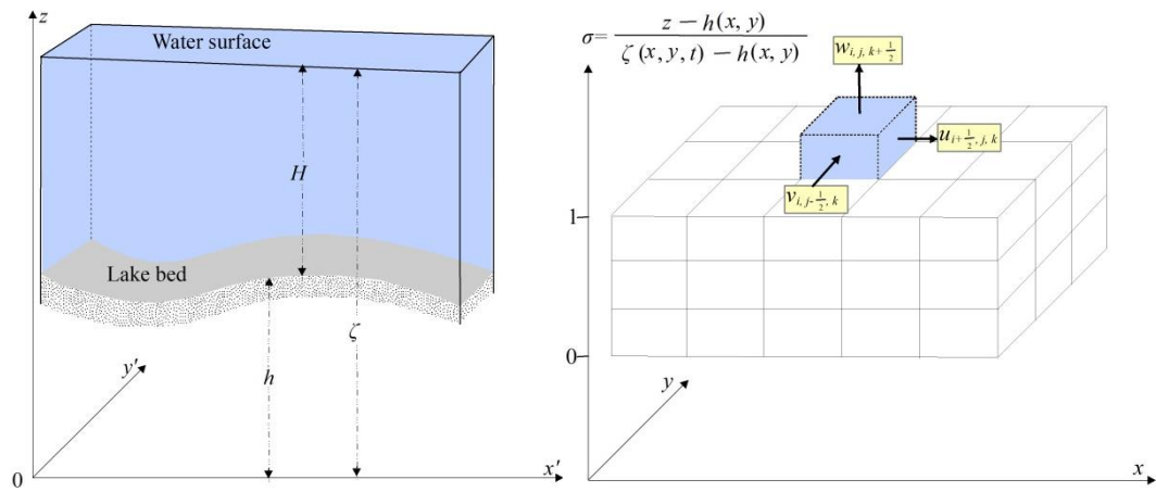
Figure 2. Lake bed elevation ( h ), water level ( \zeta ), and water depth ( H ) in the Cartesian coordinate system (left). The three components of lake current velocity in the i^{\text{th}} ( x -direction), j^{\text{th}} ( y -direction), and k^{\text{th}} ( \sigma -direction) grid of the mesh in the sigma ( \sigma ) coordinate system (right).
