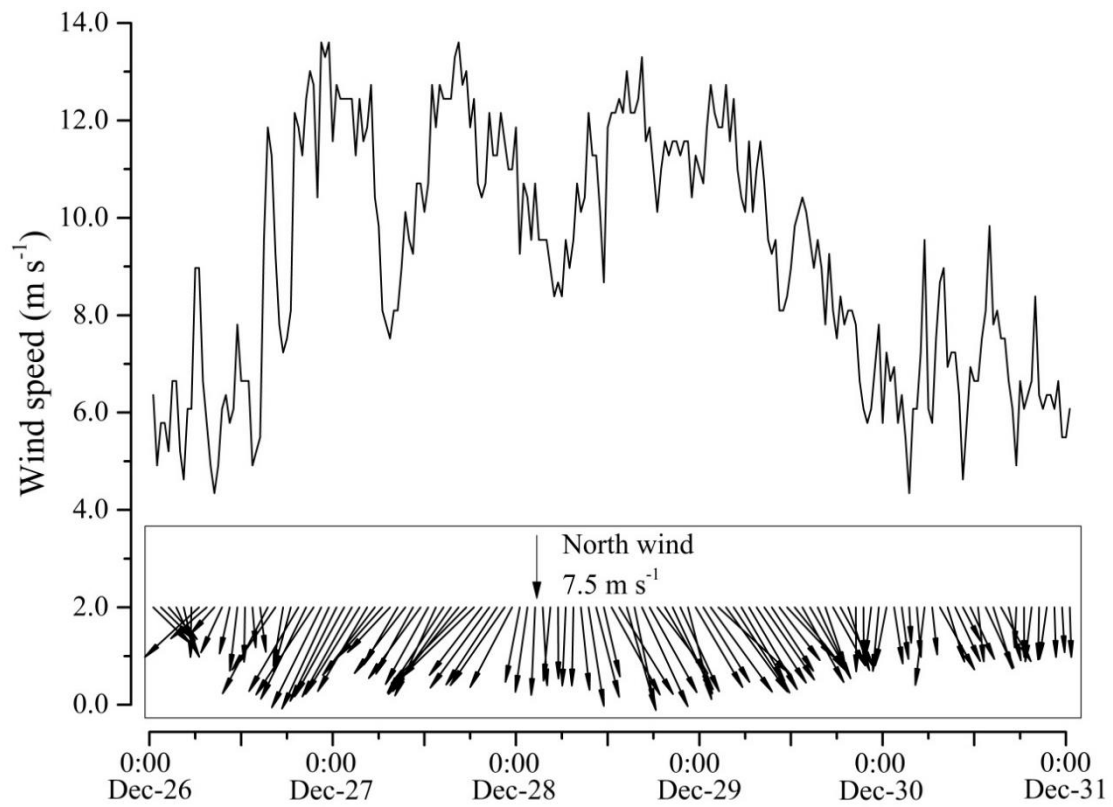
815 Figure 9. Variation of wind speed and direction at 10 m above the water surface at the LHWS during the 2018 winter observation.
