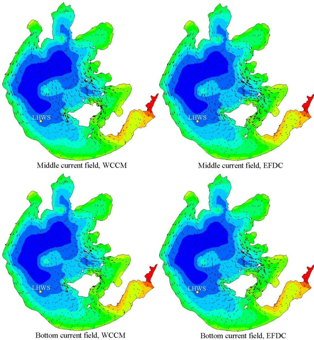
Figure 12. Comparison of the contour of the water level and surface, middle, and bottom current fields simulated by the WCCM 850 with those simulated by the EFDC at 22:00 on December 26, 2018.
