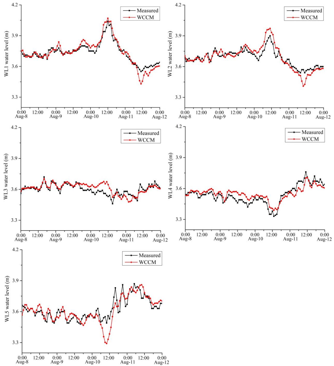
Figure 6. Comparison between the WCCM-simulated and measured water levels at the WL1–WL5 stations during the 2015 summer observation.
