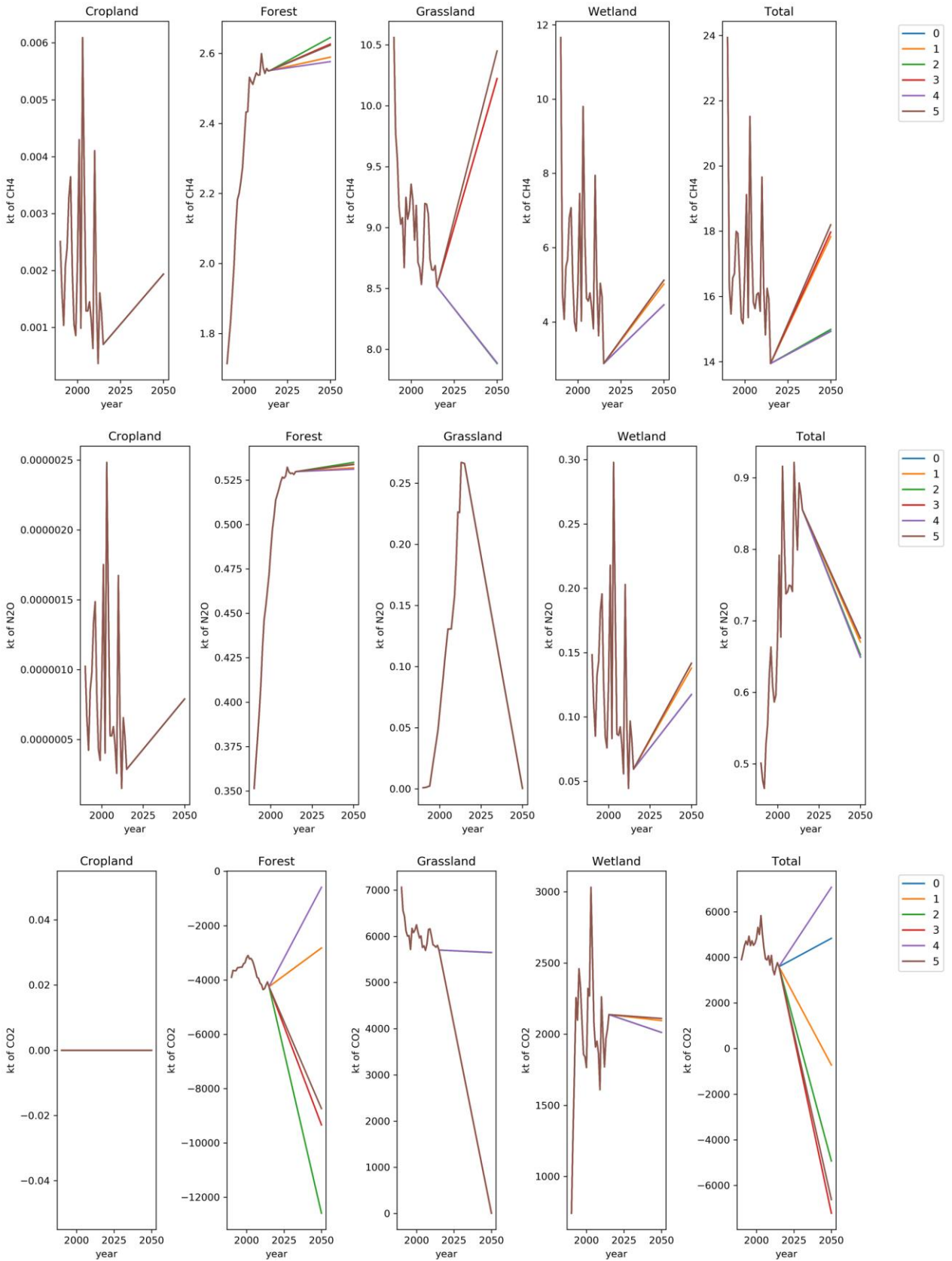
Figure 10. Scenario agricultural CH 4 , N 2 O CO 2 fluxes across cropland, forest, grassland and wetland land-uses
