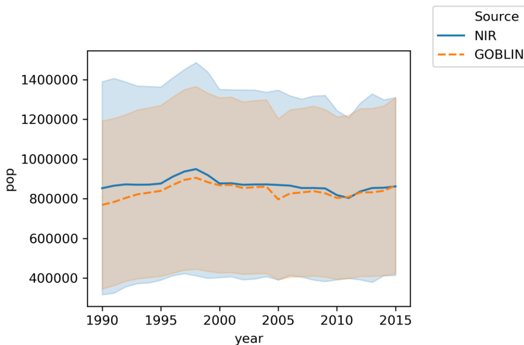
Figure 6. Average cattle livestock population (lines) and standard deviation among sub-groups over time (shaded areas) inputted to the national inventory report (NIR) and generated by the GOBLIN herd module from milking- and suckler-cow numbers, respectively.
