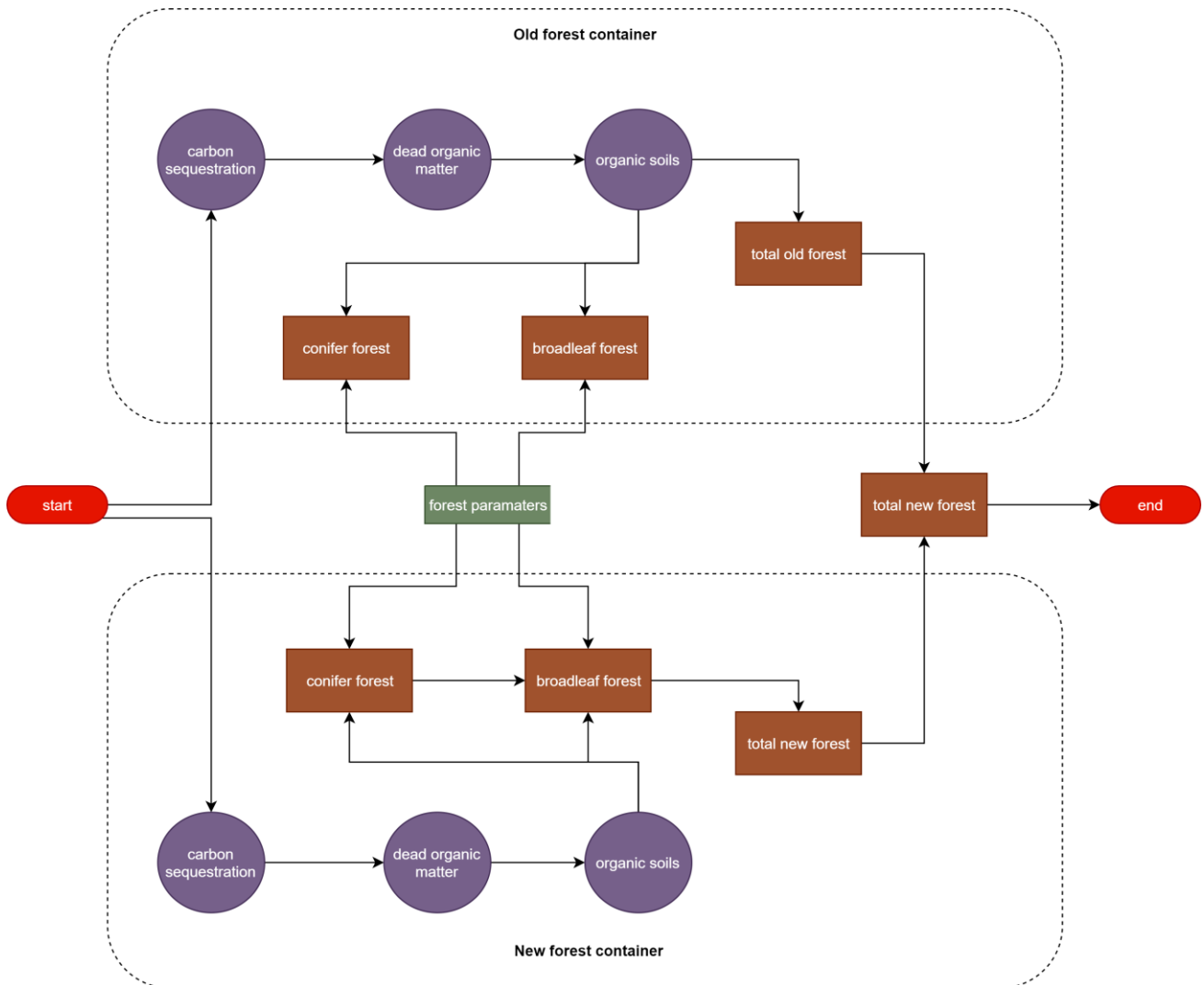
Figure 5. GOBLIN forest module calculation methodology. Arrows represent data flow. Modules are represented by brown rectangles, processes by purple circles, and open-ended green rectangles represent data stores.
