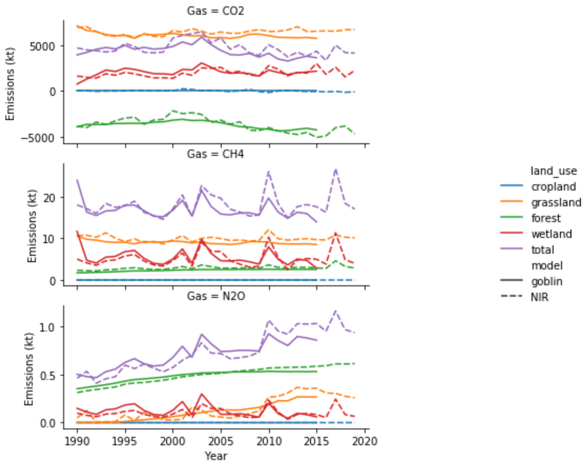
Figure 7. Comparison of land-use GHG fluxes computed by GOBLIN with those reported in national inventory reports , derived from the same activity data for 1990 to 2015
