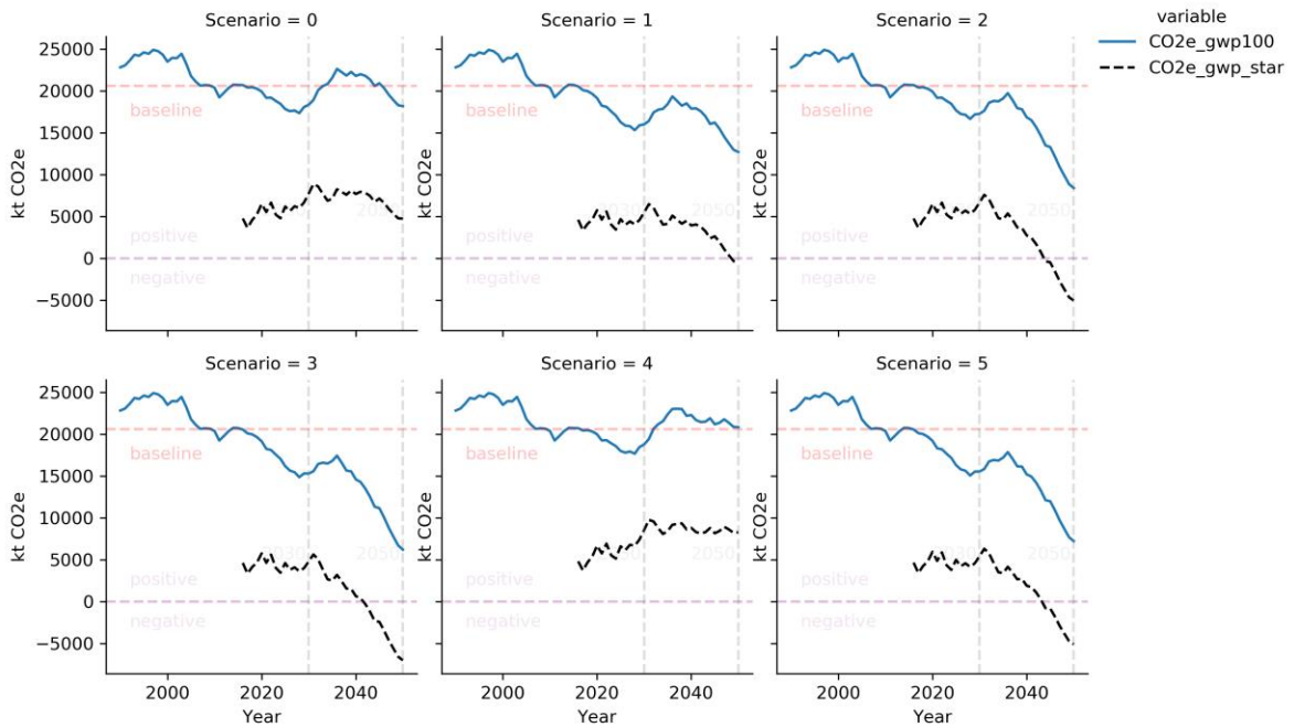
Figure 11. Net marginal GHG removals (accounted for as CO 2 e balance) from forestry between 1990 and 2050 across scenarios
