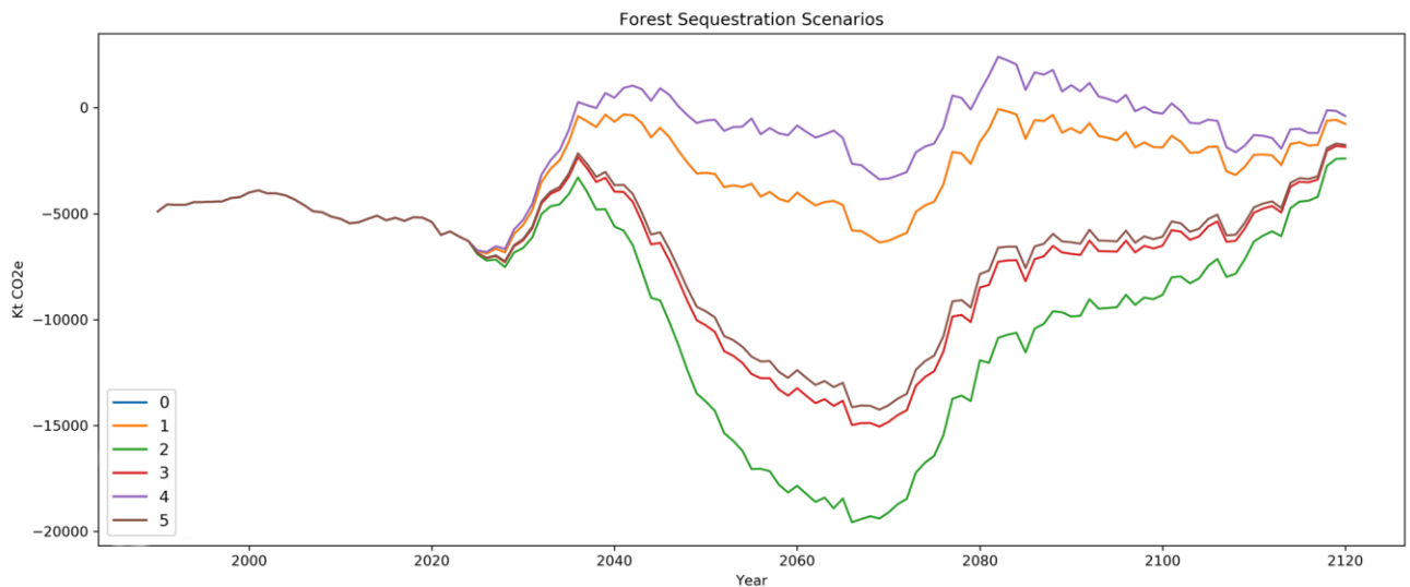
Figure 13. Net marginal GHG flux (accounted for as CO 2 e balance) from forestry between 1990 and 2120 with zero afforestation post 2050 and zero percent harvest rate
