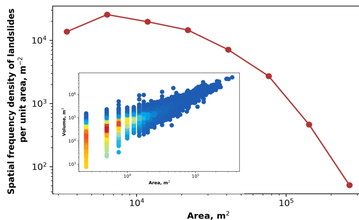
Figure 14. (a) Magnitude-frequency relationship of the landslides simulated with Landlab-HyLands (red dots) and illustrated in Fig. 13. (Inset) Scatter density plot showing the simulated Area-Volume relationship.
