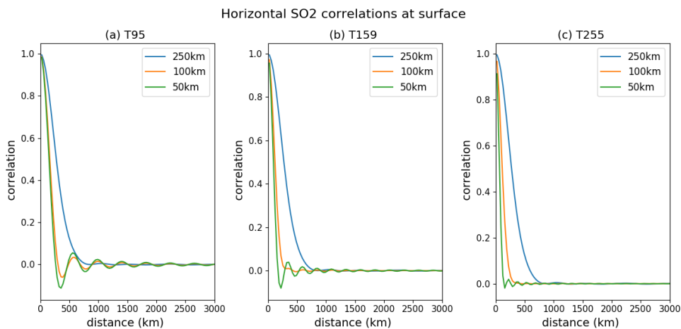
410 Figure 4: SO 2 background error horizontal surface correlations at different truncations: (a) TL95, (b) TL159 and (c) TL255 if the horizontal length scales are specified as Gaussian correlation function with length scales of 250 km (blue), 100 km (orange) and 50 km (green).
