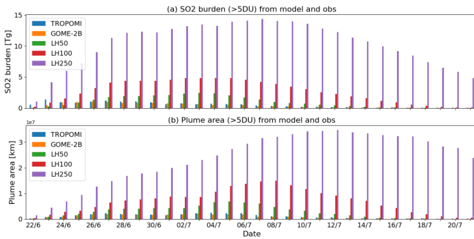
450 Figure 6: (a) SO 2 burden in Tg and (b) plume area in 1e 7 km 2 from TROPOMI, GOME-2B and three SO 2 LH experiments at 0z with horizontal background error length scales of 50 km (LH50), 100km (LH100) and 250 km (LH250) for the Raikoke eruption (22 June to 21 July 2019). The values are calculated by gridding the data on a 1°x1° grid and selecting the grid cells with TCSO 2 values greater than 5 DU in the area 30-90°N.
