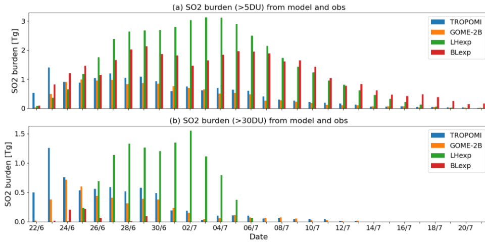
535 Figure 10: SO 2 burden in Tg from TROPOMI, GOME-2B, LHexp and BLexp TCSO 2 analysis at 0z for the Raikoke eruption (22 June to 21 July 2019). The values are calculated by gridding the data on a 1°x1° grid and selecting the grid cells with TCSO 2 values greater than (a) 5 DU and (b) 30 DU in the area 30-90°N.
