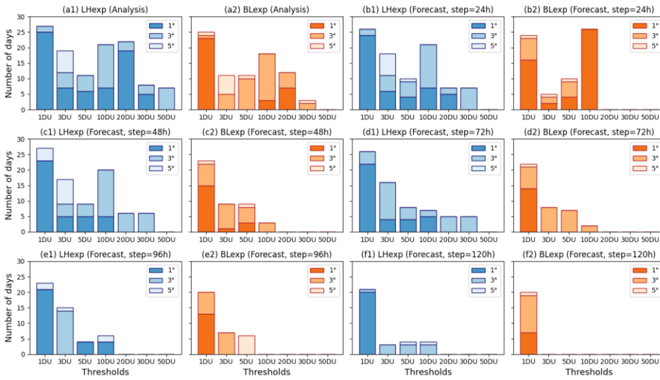
640 Figure 17: Number of days since the eruption on 22 June 2019 that the LHexp (blue) and BLexp (orange) (a) analyses and forecasts at steps (b) 24, (c) 48, (d) 72, (e) 96 and (f) 120-hours have some skill ( FSS>0.5 ) compared to NRT TROPOMI TCSO 2 data for neighbourhood sizes of 1°, 3° and 5° and thresholds of 1, 3, 5, 10, 20, 30, 50 DU.
