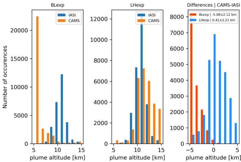
595 Figure 15: Comparison of plume altitude from IASI ULB LATMOS data with the altitude of maximum \text{SO}_2 concentration from the LHexp (middle panel) and BLexp (left panel) for the period 22-29 June 2019. The right panel shows a histogram of the differences of the plume altitudes (CAMS minus IASI) for LHexp (blue) and BLexp (red).
