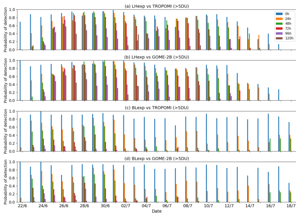
605 Figure 16: Probability of detection of LHexp against (a) NRT TROPOMI and (b) GOME-2B, as well as BLexp against (c) NRT TROPOMI and (d) GOME-2B for the period 22 June to 18 July 2021 for analysis at 0z (blue), 24-hour forecast (orange), 48-hour forecast (green), 72-hour forecast (red), 96-hour forecast (purple) and 120-hour forecast (brown).
