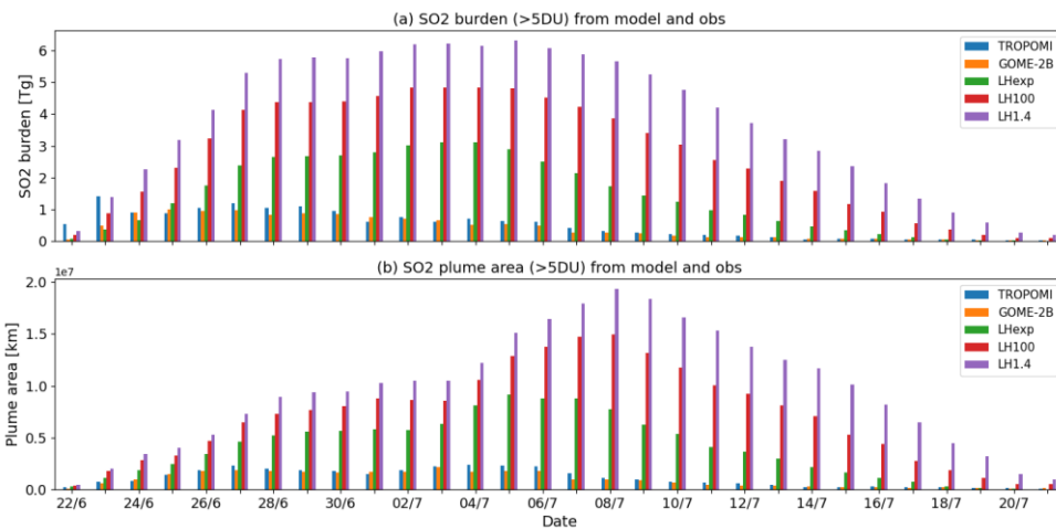
460 Figure 7: (a) SO 2 burden in Tg and (b) plume area in 10 7 km 2 from TROPOMI, GOME-2B and three SO 2 LH experiments at 0z with background error standard deviation values of 0.7e-7 (LHexp), 1e-7 (LH100) and 1.4e-7 kg/kg (LH1.4) for the Raikoke eruption (22 June to 21 July 2019). The values are calculated by gridding the data on a 1°x1° grid and selecting the grid cells with TCSO 2 values greater than 5 DU in the area 30-90°N.
