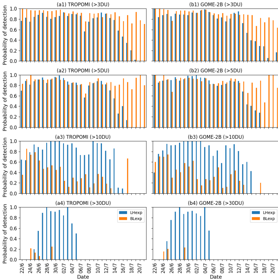
550 Figure 12: Timeseries of POD for TCSO 2 analysis fields (at 0z) against (a) NRT TROPOMI and (b) GOME-2B for TCSO 2 thresholds of (1) 3DU, (2) 5 DU, (3) 10 DU and (4) 30 DU (22 June to 21 July 2019). Values for LHexp are shown in blue, values for BLexp in orange.
