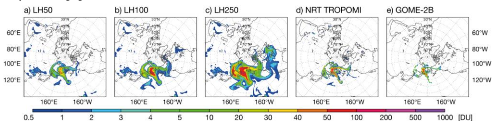
430 Figure 5: TCSO 2 analyses on 27 June 2019 at 0z obtained by assimilating SO 2 LH data using a background standard deviation profile of 10 -7 kg/kg and background errors with horizontal correlations of (a) 50 km, (b) 100 km and (c) 250 km. Also shown are (d) NRT TROPOMI and (e) GOME-2B TCSO 2 values.
