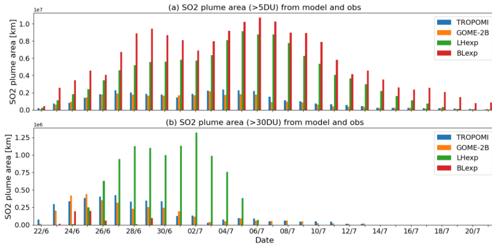
540 Figure 11: SO 2 plume area [km 2 ] from TROPOMI, GOME-2B, LHexp and BLexp TCSO 2 analysis at 0z for the Raikoke eruption (22 June to 21 July 2019). The values are calculated by gridding the data on a 1°x1° grid and selecting the grid cells with TCSO 2 values greater than (a) 5 DU and (b) 30 DU in the area 30-90°N.
