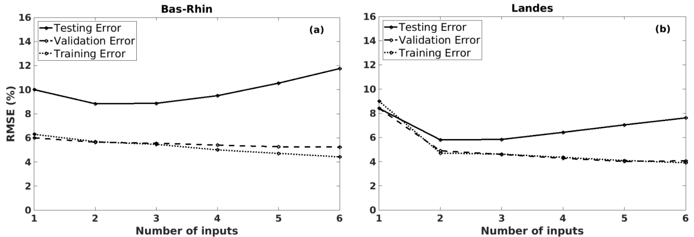
Figure 10. The training/validation/testing RMSE values of the predicted grain maize yield anomalies, using different LIN models (with 12 potential predictors) by increasing the number of inputs, in (a) Bas-Rhin and (b) Landes.
