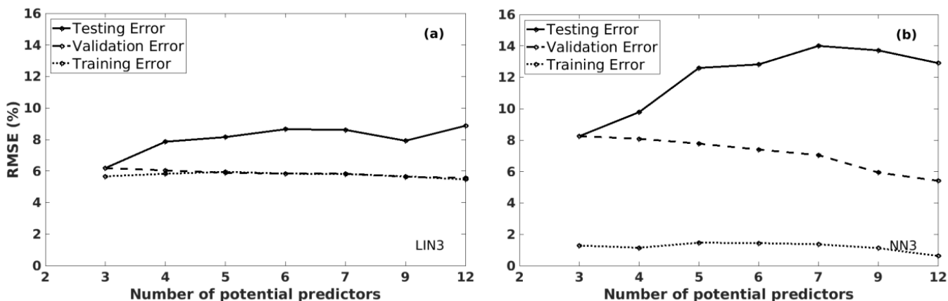
Figure 12. The training/validation/testing RMSE values of the predicted grain maize yield anomalies, using different models by increasing the number of potential predictors, in Bas-Rhin (France): (a) LIN3 and (b) NN3 (with n_{neuron} = 7 ) models.
