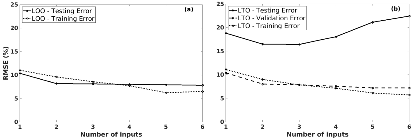
Figure 7. The training/validation/testing RMSE values of the predicted coffee yield anomalies, using different LIN models (with 18 potential predictors) by increasing the number of inputs, in Cu M'gar (Dak Lak, Vietnam): (a) is induced from LOO procedure, (b) is from LTO procedure.
