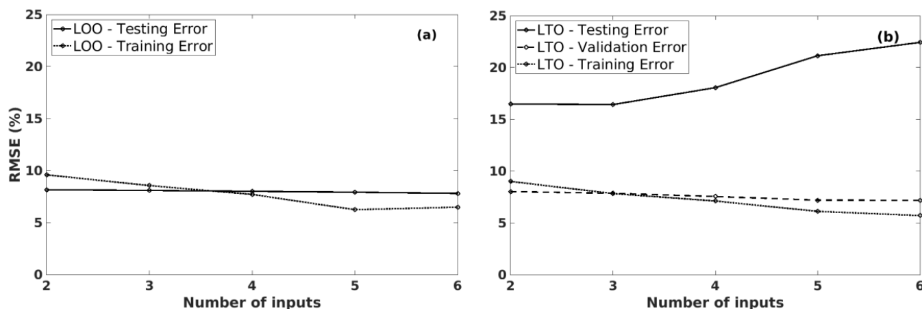
Figure 6. The training/validation/testing RMSE values of the predicted coffee yield anomalies, using different LIN models (with 18 potential predictors) by increasing the number of inputs, in Cu M'gar (Dak Lak, Vietnam): (a) is induced from LOO procedure, (b) is from LTO procedure.
