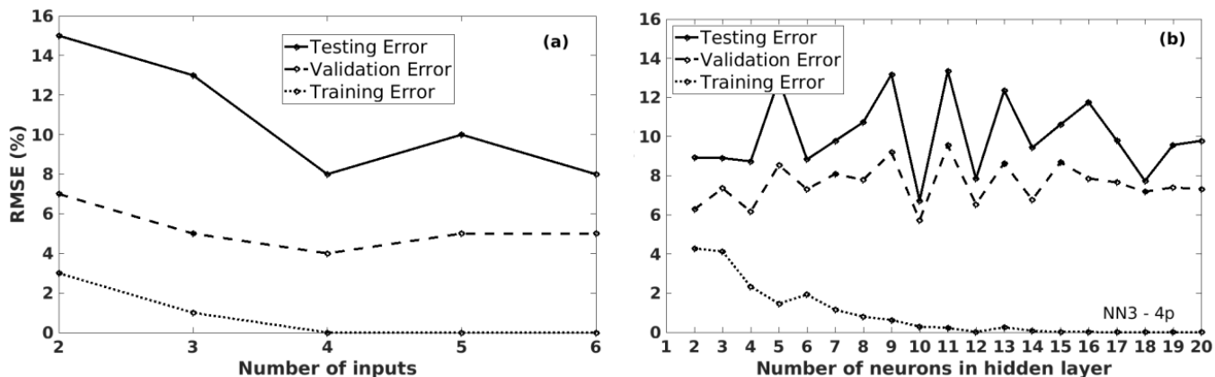
Figure 11. The training/validation/testing RMSE values of the predicted grain maize yield anomalies, using different NN models with various choices, in Bas-Rhin (France): (a) NN models (with n_{pre} = 12 and n_{neuron} = 7 ) by increasing the number of inputs, (b) NN3 models (with n_{pre} = 4 ) by increasing the number of neurons in the hidden layer.
