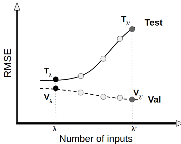
Figure 5. Schematic illustration of validation and testing RMSE values of predicted yield anomalies for an increasing number of inputs, obtained from the LTO procedure. For a fixed complexity level, i.e., n_{input} = \lambda , two RMSE values are obtained: V_\lambda for validation and T_\lambda for testing datasets. (The cases of underfitting are excluded in this illustration.)
