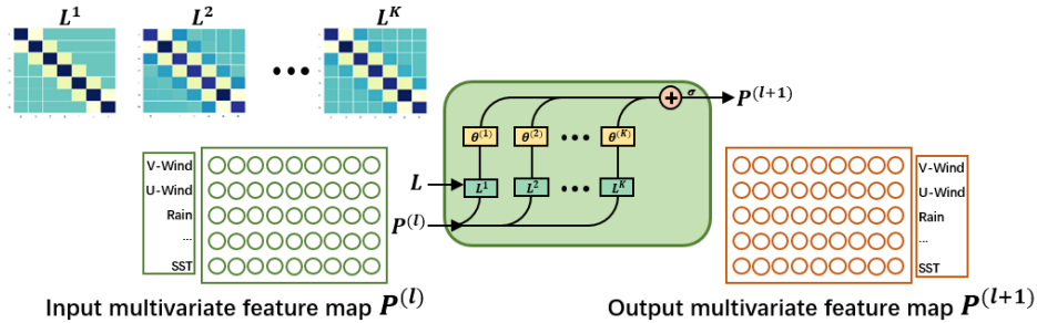
290 Figure 7: K -order graph convolution layer. K is the truncated order and L^k represents the interactions between k -order neighbours. and each row in p^{(l)} and p^{(l+1)} represents features of different physical variables, and their positions are not changed during forward propagation.
