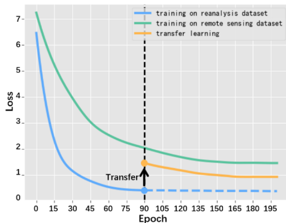
450 Figure 11: The loss changes when training with only reanalysis dataset (blue line), with only remote sensing dataset (green line) and transfer learning on these two datasets in order (black arrow and yellow line after 90 epochs).
