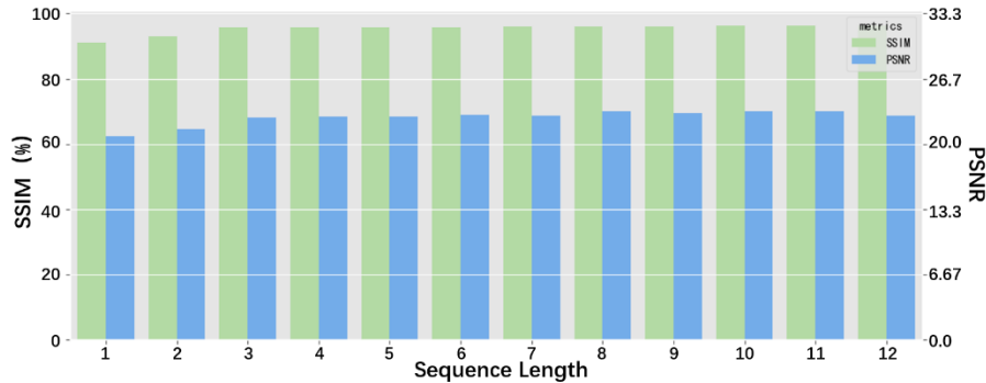
430 Figure 10: The performances of the ENSO-ASC when the input sequence length increases under IMS forecast strategy.
