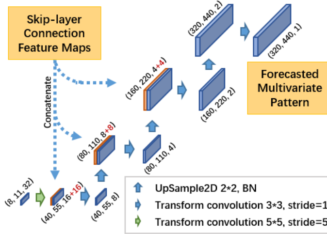
335 Figure 9: A detailed structure for decoder, skip-layer connections (the red channel cascaded to the feature maps) from encoder for helping end-to-end learning to restore the forecasted patterns at different spatial scales.
