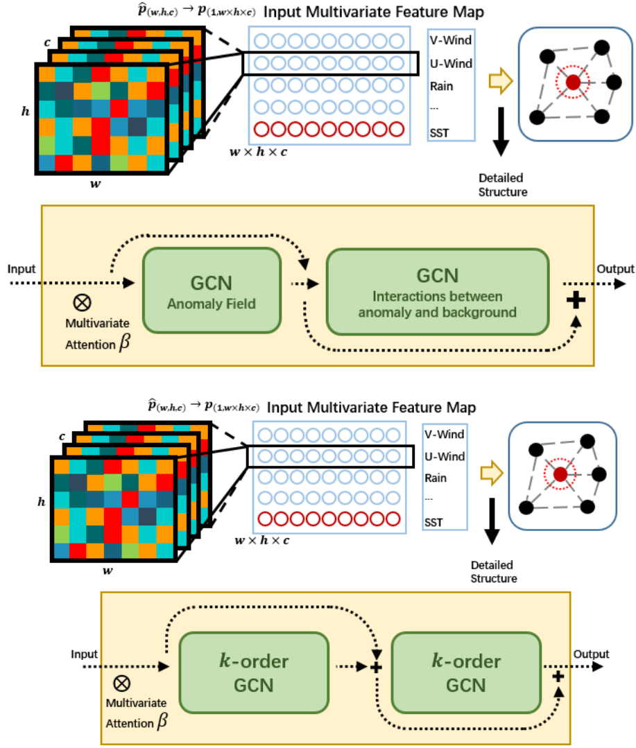
Figure 8: A detailed structure for multivariate air-sea coupler between encoder and decoder: Pre-processes for input (upper row), and dual-layer structure for simulating interactions between anomalous and background fields residual learning (lower row). There is also a multivariate attention component-weight in the coupler.
