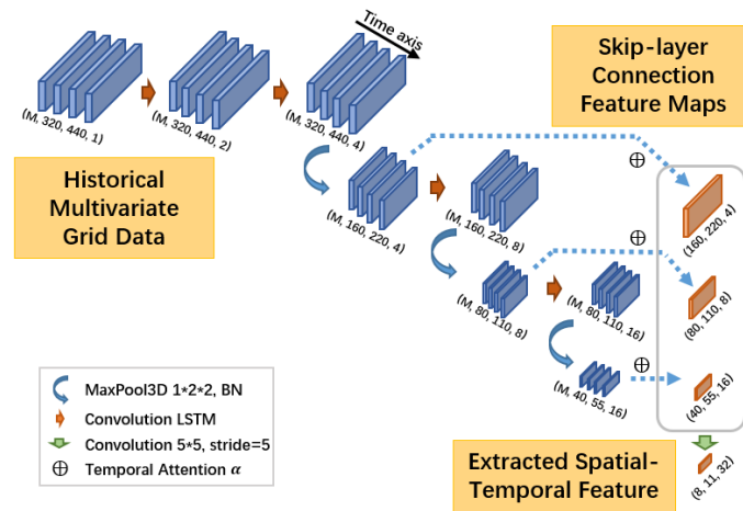
Figure 5: A detailed structure for encoder: Stacked ConvLSTM encoder for extracting spatial-temporal features simultaneously. There is also temporal attention component-weight for skip-layer connections in the grey box.
