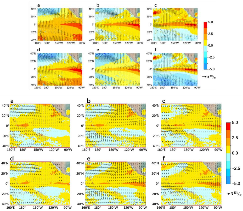
Figure 17: The growth phase of SST and wind anomalies in 2015/2016 super Niño event from 2015.4 to 2015.6. a-c are the forecast results of the ENSO-ASC and d-f are real-world observations.
