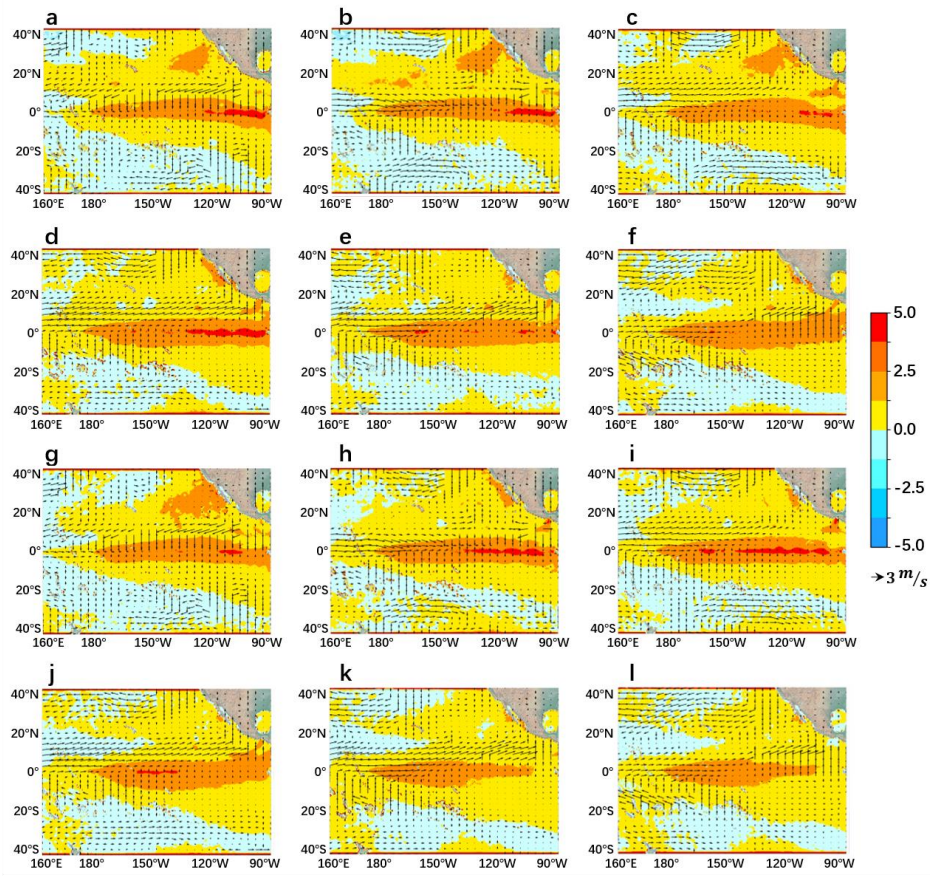
Figure 1848: The peak phase of SST and wind anomalies in 2015/2016 super Niño event from 2015.9 to 2016.2. a-f are the forecast results of the ENSO-ASC and g-l are real-world observations.
