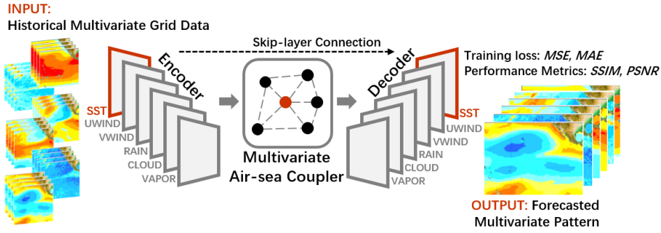
Figure 3: The structure of ENSO-ASC. There are 6 encoders for the chosen variables to extract spatial-temporal information and a multivariate air-sea coupler to simulate interactions. After interactions, we design 6 decoders to restore the major variable SST and other variables. The training loss and performance metrics are also displayed.
