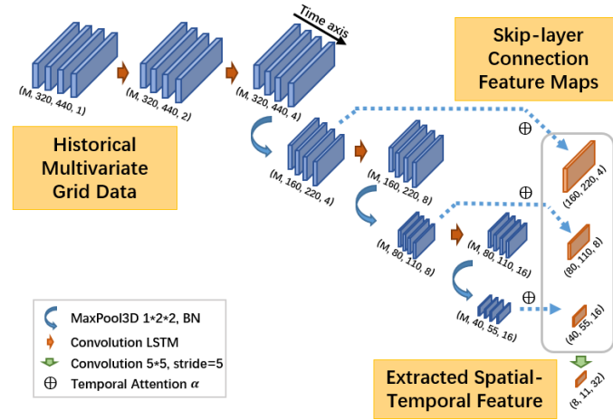
Figure 5: A detailed structure for encoder: Stacked ConvLSTM encoder for extracting spatial-temporal features simultaneously. There is also temporal attention component-weight for skip-layer connections in the grey box.
