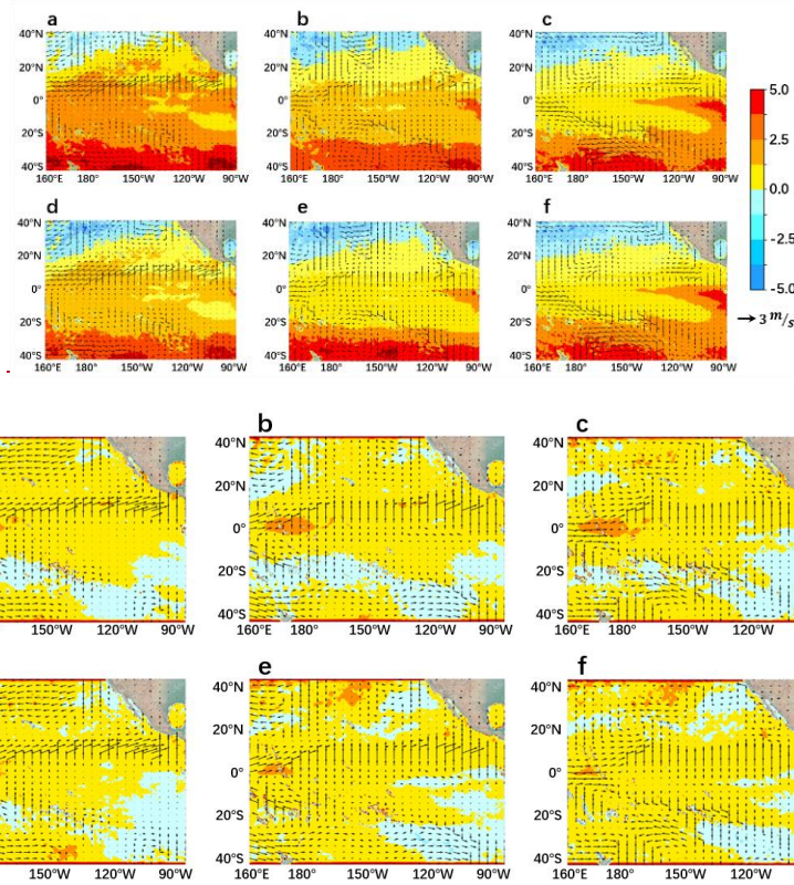
Figure 20: The same with Fig. 17 but for the neural SST and wind anomalies evolutions in 2020.1 to 2020.3.
