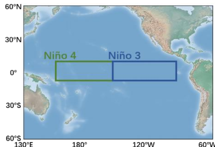
Figure 1: Most concerned regions in ENSO events. The blue rectangle covers the Niño3 region ( 5^{\circ}\text{N} - 5^{\circ}\text{S} , 150^{\circ}\text{W} - 90^{\circ}\text{W} ), and the green rectangle covers the Niño4 region ( 5^{\circ}\text{N} - 5^{\circ}\text{S} , 160^{\circ}\text{E} - 150^{\circ}\text{W} ).
