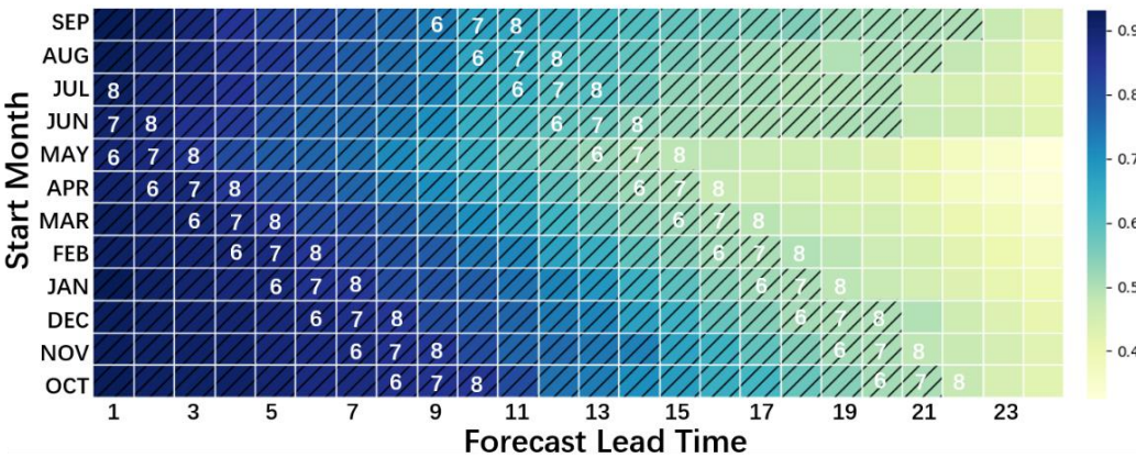
650 Figure 15: The correlation skill heat map between the forecast results of the ENSO-ASC and real-world observations on Niño3.4 index with different forecast start months over the validation period. The hatching cells represent the correlations over-exceed 0.5, and the white numbers on the cells mean the forecast-calendar months.
