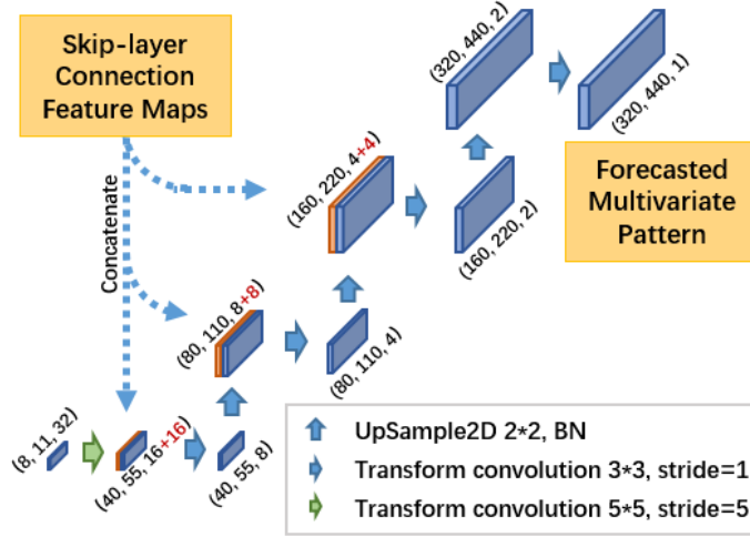
Figure 9: A detailed structure for decoder, skip-layer connections (the red channel cascaded to the feature maps) from encoder for helping end-to-end learning to restore the forecasted patterns at different spatial scales.
