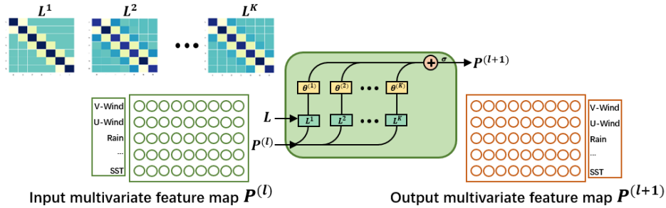
Figure 7: K -order gGraph convolution layer. K is the truncated order and L^k represents the interactions between k -order neighbours. Each row in P^{(l)} and P^{(l+1)} represents features of different physical variables, and their positions are not changed during forward propagation.
