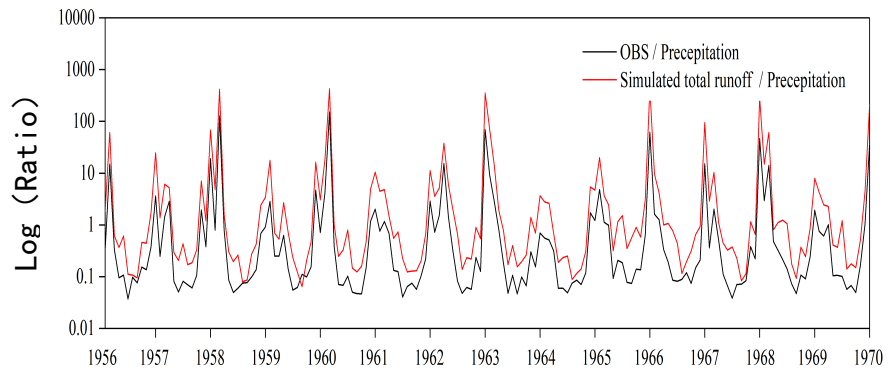
Figure S2. The ratios of the observed (dark line) and simulated (red line) runoff (default model) to observed precipitation for the WRB over the period of 1956-1969 based on the default options of CLM.
