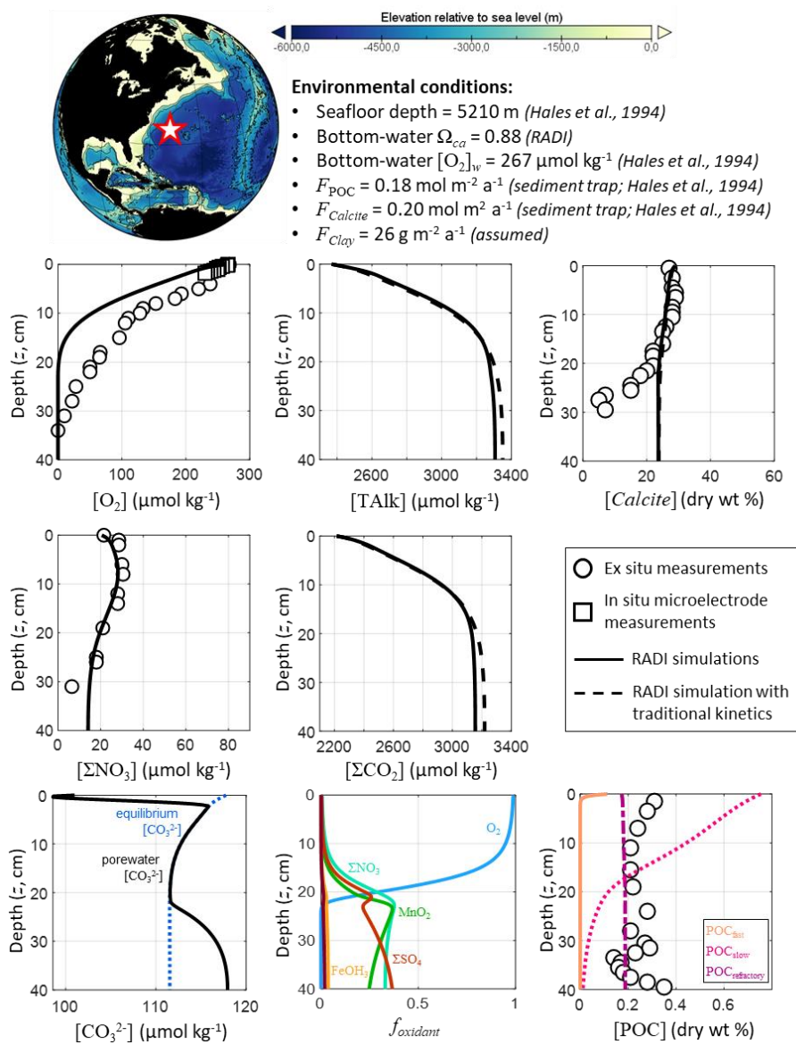
Figure 4. Comparison of RADI with measurements from the North-western Atlantic station #9 described in ( Hales et al., 1994 ). The lower panels represent (left) the computed CO_3^{2-} concentrations in porewaters (solid black line) and at equilibrium with respect to calcite (dashed blue line), and (center) the fractions of organic matter degraded by a given oxidant.
