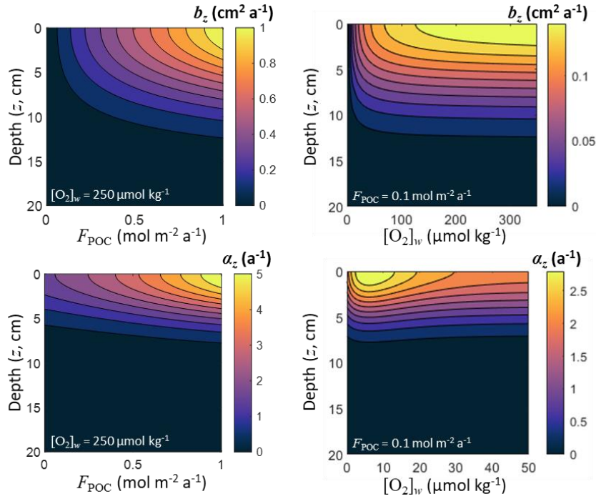
485 Figure 3. Bioturbation mixing rate b_z and irrigation coefficients \alpha_z as a function of sediment depth z , organic carbon deposition flux F_{\text{POC}} , and dissolved oxygen concentration in the bottom waters [\text{O}_2]_w .
