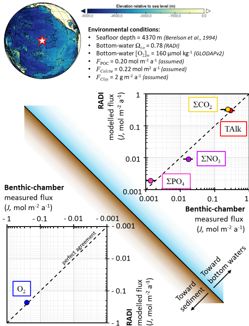
Figure 6. Comparison of fluxes computed from RADI with benthic-chamber measurements from the station #W-2 described in Hammond et al. (1996). Error bars are included for all measured fluxes but not always visible.
