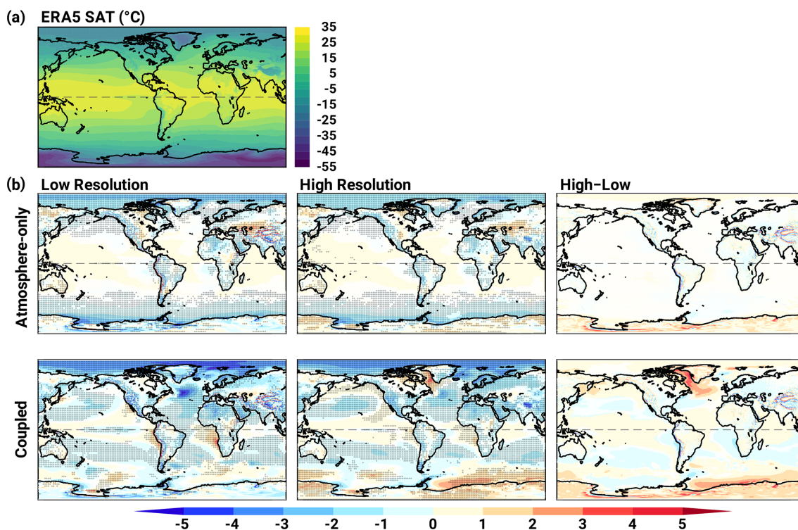
Figure 1. (a) ERA5 near-surface (2 m) air temperature (SAT; in °C). (b) Left and middle: multi-model ensemble mean bias in (2 m) SAT CE2 (in °C) in the atmosphere-only (top) and coupled (bottom) simulations at low (left) and high (middle) resolutions. Biases are with respect to ERA5 (shown in a). Stippling masks where at least four out of the five models agree on the anomaly sign. Right: difference between the two resolutions. In all panels non-significant anomalies at the 5 % level (based on a two-tailed Student's t test) are masked white. The Equator is a dashed line in all the panels.
