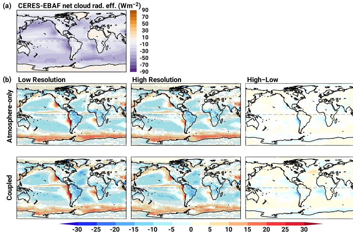
Figure 5. (a) CERES-EBAF net cloud radiative effect (in \text{W m}^{-2} ). (b) Multi-model ensemble mean bias in net cloud radiative effect (in \text{W m}^{-2} ) with respect to CERES-EBAF at low and high resolution (left and middle) and differences between the two resolutions (right), as in Fig. 1.
