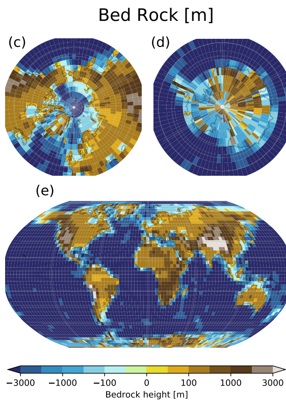
Figure 1. Initial ice thickness (a,b) and bed rock (c-e) in GREB-ISM. Ice thickness less than 10 m is not shown.
