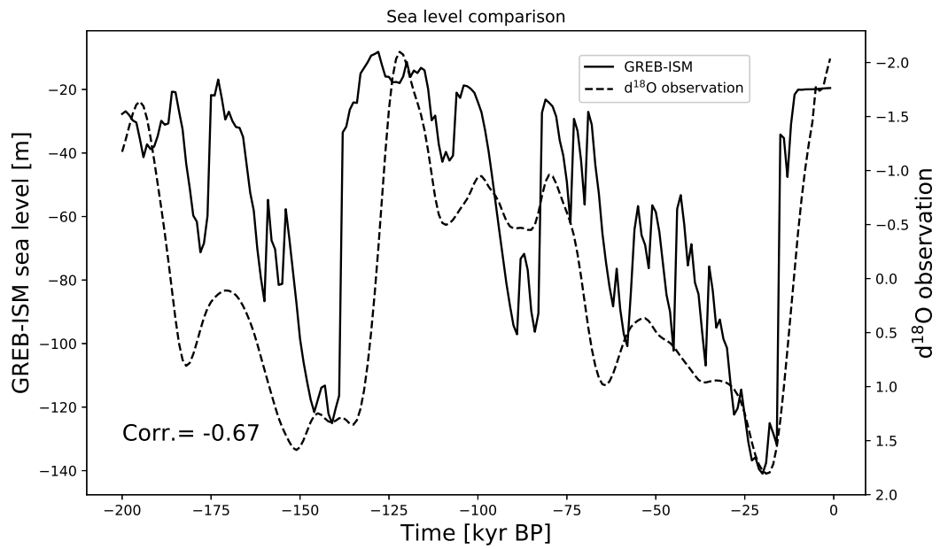
Figure 10. Time series of simulated sea level (left axis; units: m ) from the stand-alone transition experiment and d 18 O proxy data (right axis, the axis has been inverted to have a better comparison ).
