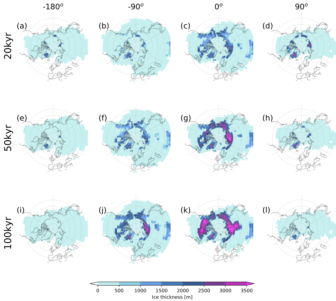
Figure 16. Ice thickness (unit: m) distribution in four phases within for the forcing period periods of 20 kyr (upper), 50 kyr (middle) and 100 kyr (lower) from the last cycle of the simulations shortwave oscillation experiment . The headings mark the corresponding -180^\circ , -90^\circ , 0^\circ and 90^\circ phase of the solar forcing phases are marked in the headings.
