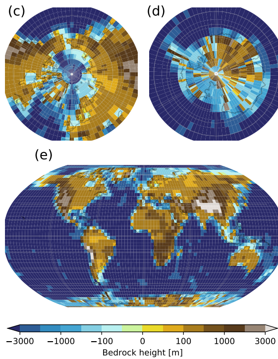
Figure 1. Topography-Initial ice thickness (a,b) and bed rock (c-e) in GREB-ISM. Ice thickness less than 10 m is not shown.
