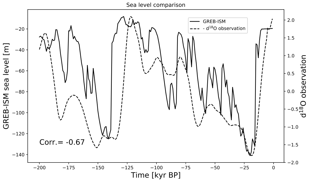
Figure 10. Time series of simulated sea level (left axis; units: m ) from the GREB-ISM stand-alone transition experiment and d 18 O observation proxy data (right axis).
