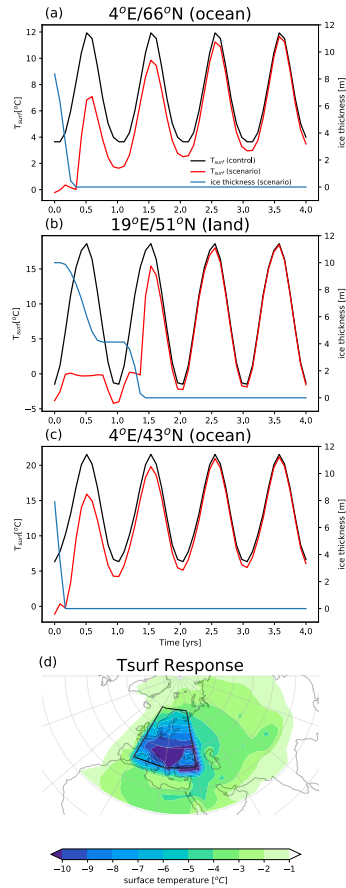
Figure 4. GREB-ISM surface temperature and ice thickness response to adding a 10 m ice sheet in surface temperature (units: °C) and ice thickness experiment (units: m). (a), (b) and (c) are the temperature (units: °C) and ice thickness (units: m) evolution in at three different sites locations. The black, red and blue curve represent control run surface temperature (without adding 10 m ice), scenario run surface temperature (with adding 10 m ice) and scenario run ice thickness. (d) shows the temperature difference (units: °C) between scenario and control at the end of the first simulation year after adding 10m. The black outlined region in (d) mark the area in which the initial 10 m ice thickness anomalies sheet is added.
