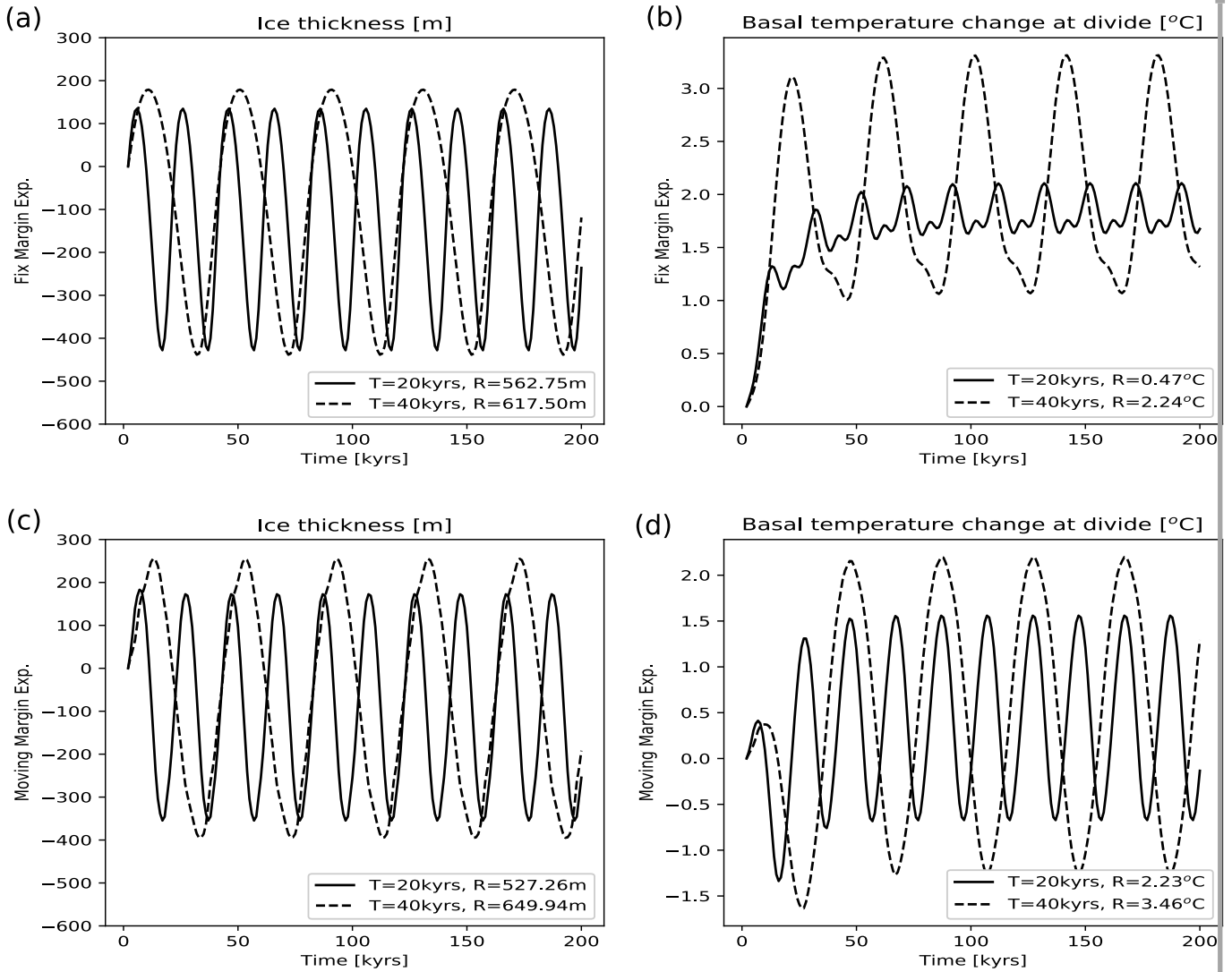
Figure 6. Time evolution of ice thickness (a, c, unit: m ) and homologous basal temperature (b, d, unit: K ) in the EISMINT I fixed (a, b) and moving margin experiments with GREB-ISM (c, d) margin experiments with GREB-ISM with 20/40 kyr period forcing. R marks the range (maximum minus minimum in the last 50 kyr) of the simulated variables.
