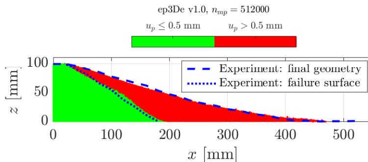
Figure 6. Final geometry of the granular collapse for three-dimensional configuration of our GPU-based explicit GIMPM implementation ep3De v1.0. The green region (i.e., the intact region) is defined by the L_2 -norm of the material point displacement u_p = \|\mathbf{u}_p\|_2 \leq 0.5 mm, whereas the red region (i.e., the deformed region) is defined by u_p = \|\mathbf{u}_p\|_2 > 0.5 mm. The experiment of Bui et al. (2008) is indicated by the blue dashed line (i.e., the free surface) and the blue dotted line (i.e., the failure surface).
