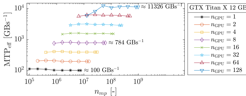
Figure 18. MTP_{\text{eff}} sum across the GPUs involved.
