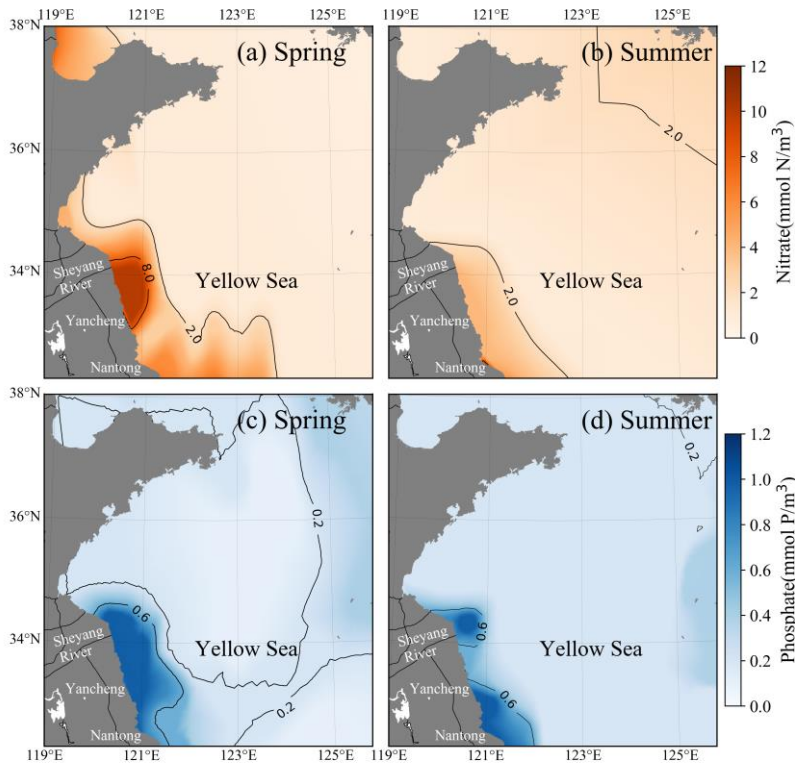
315 Figure. 7. Seasonal-averaged surface distributions of nitrate (upper) and phosphate (lower) in YS during spring (left), summer (right).
