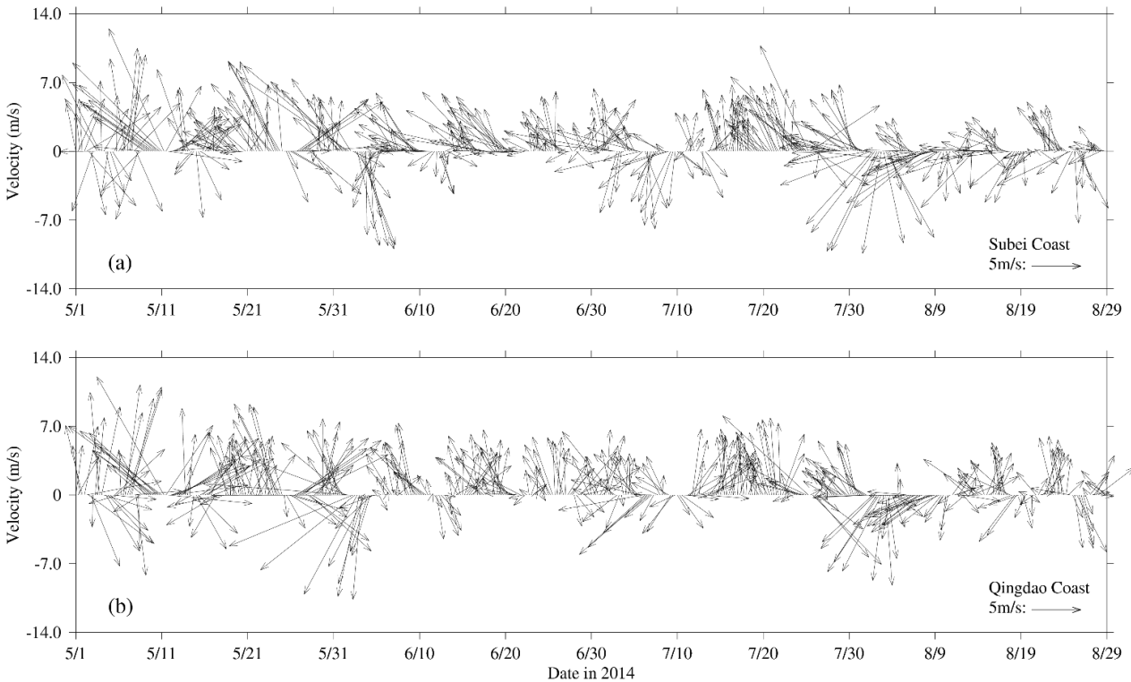
Figure. 4. Wind vectors at 10-m-height near Subei coast (a) and Qingdao coast (b) at a time interval of 6-hrs from May to August 2014.
