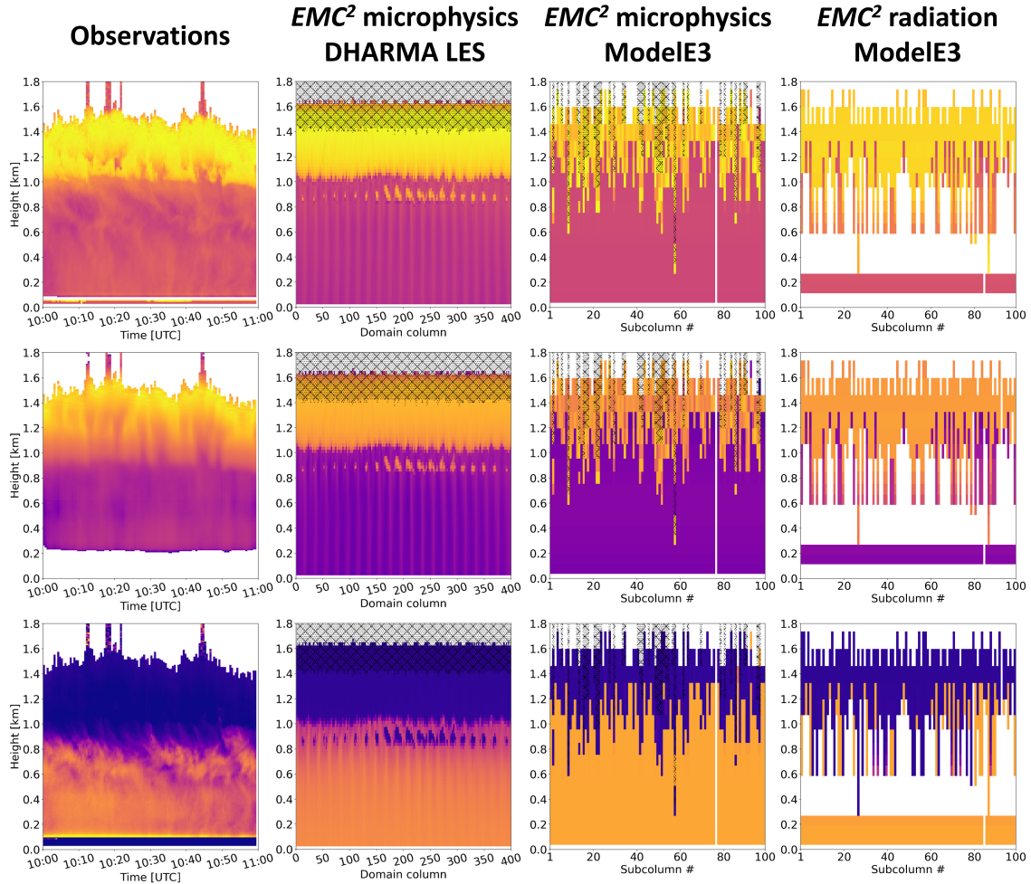
Figure 4. Observed and simulated HSRL particulate backscatter cross-section ( \beta_{ptot} ; top row), particulate extinction cross-section ( \alpha_{ptot} ; middle row), and linear depolarization ratio (LDR; bottom row) using the DHARMA LES output and ModelE3 configuration Tun3 SCM output. The columns show (from left to right) the observations from McMurdo Station between 10:00-11:00 UTC, DHARMA LES three-dimensional output (horizontal dimensions stacked onto a single domain column dimension) processed using EMC 2 microphysics with the subcolumn generator turned off ( N_s = 1 ), ModelE3 EMC 2 output using the microphysics approach, and EMC 2 output using the radiation approach. The DHARMA LES output corresponds to 10:00 UTC (arrival of cloud field at McMurdo Station; see sect. 3.2), while ModelE3's EMC 2 panels depict the SCM output for 05:00 UTC (see text) processed with EMC 2 using 100 subcolumns. A mask denoting full lidar signal attenuation generated using a total accumulated optical thickness ( \tau_{tot} ) condition of \tau_{tot} > 4 is plotted over the simulated data (hatched areas).
