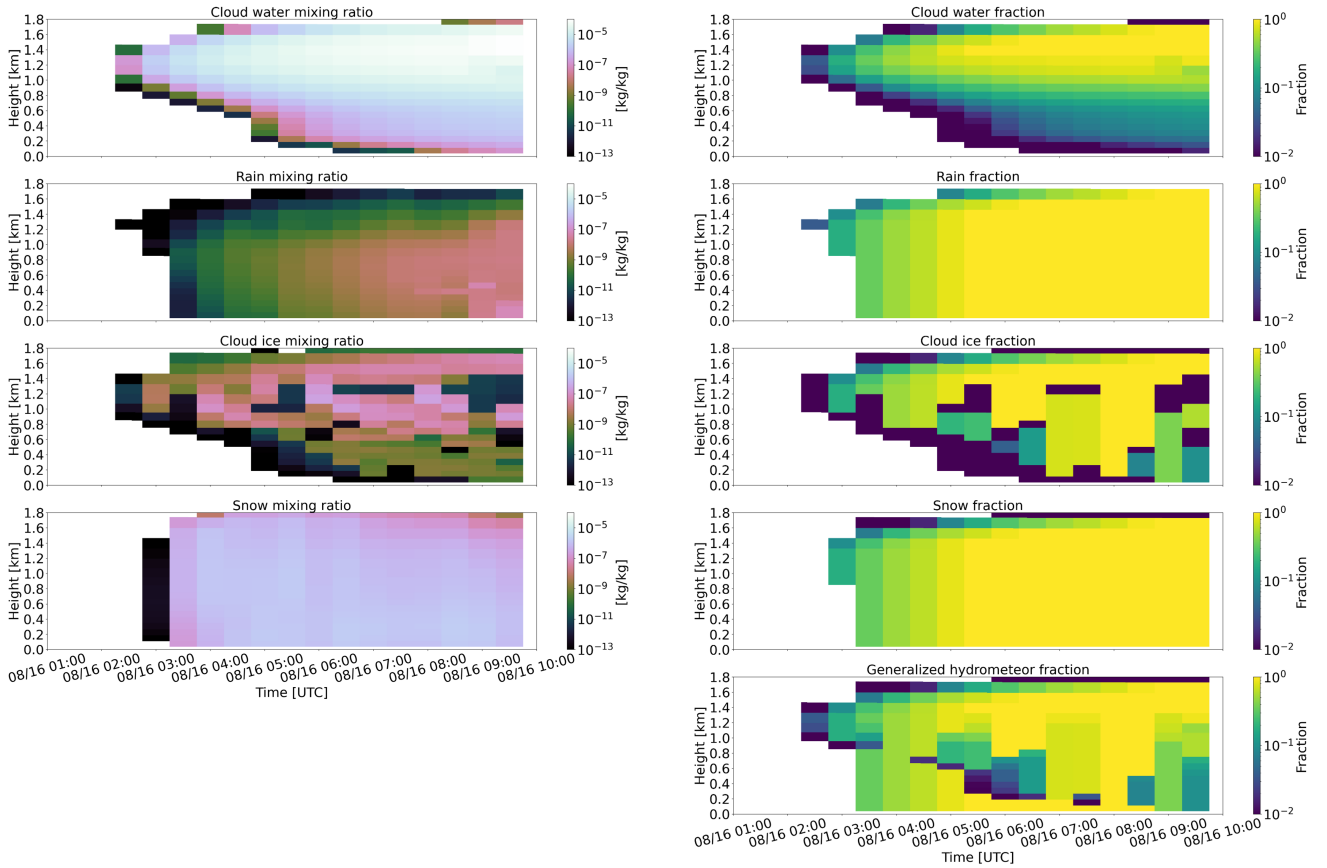
Figure 3. ModelE3 configuration Tun3 single column model (SCM) output for the Antarctic cloud case study (August 16, 2016) showing mixing ratio (left) and hydrometeor fraction (right) time-height curtain plots of (from top to bottom) cloud water, rain, cloud ice, and snow. The generalized hydrometeor fraction used in the radiation approach (see sect. 2) is depicted in the bottom right panel.
