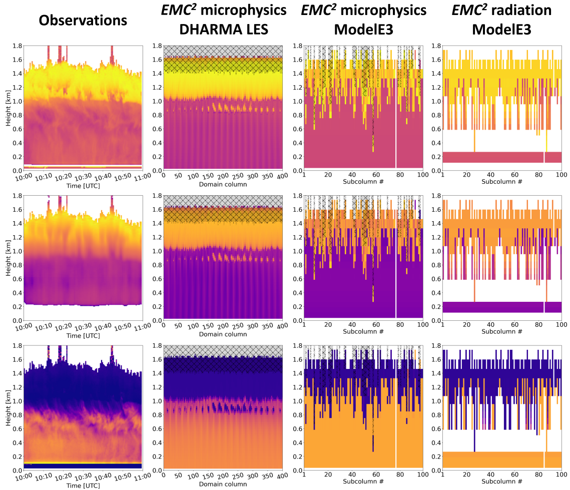
Figure 4. Observed and simulated HSRL particulate backscatter cross-section ( \beta_{p_{tot}} ; top row), particulate extinction cross-section ( \alpha_{p_{tot}} ; middle row), and linear depolarization ratio (LDR; bottom row) using the DHARMA LES output and ModelE3 configuration Tun3 SCM output. The columns show (from left to right) the observations from McMurdo Station between 10:00-11:00 UTC, DHARMA LES three-dimensional output ( horizontal dimensions stacked onto a single domain column dimension ) processed using EMC 2 microphysics ( without with the subcolumn generator turned off ( N_s = 1 ) ), ModelE3 EMC 2 output using the microphysics approach, and EMC 2 output using the radiation approach, and EMC 2 output using the empirical approach with the microphysics cloud fractions for the subcolumn generator (see sect. 2.2) . The DHARMA LES output corresponds to 10:00 UTC (arrival of cloud field at McMurdo Station; see sect. 3.2), while ModelE3's EMC 2 panels depict the SCM output for 05:00 UTC (see text) processed with EMC 2 using 100 subcolumns. A mask denoting full lidar signal attenuation mask of \tau_{tot} > 4 ( \tau_{tot} is the generated using a total accumulated optical thickness ( \mathcal{T}_{tot} ) condition of \mathcal{T}_{tot} > 4 is applied to the plotted over the simulated data (hatched areas).
