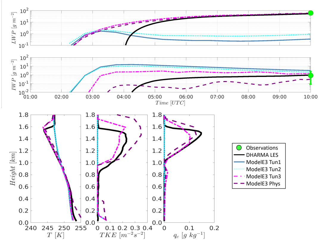
Figure B1. Time series showing (top) liquid water path (LWP) and (middle) ice water path (IWP) in each case study simulation using the DHARMA LES (baseline simulation in Silber et al., 2019a), and the four ModelE3 configurations (Tun1, Tun2, Tun3, and Phys). The Eulerian retrievals shown for 10:00 UTC (error bars denote uncertainty) correspond to the time at which the Lagrangian simulated domain approaches McMurdo Station (see sect. 3.2). (Bottom, from left to right) Temperature, turbulent kinetic energy, and cloud water mixing ratio profiles at the end of the SCM and DHARMA LES simulations.
