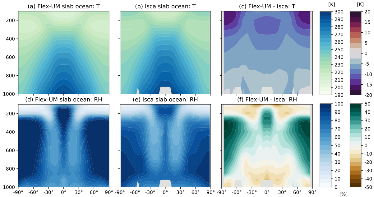
Figure 2. Slab ocean aquaplanet model climatologies for Flex-UM (left) and Isca (middle) for temperature ( T in K , top panel) and relative humidity ( RH as a %, bottom panel) on their native model grids. The differences between the models (Flex-UM - Isca) is plotted in the right panels and are interpolated onto the Flex-UM grid. Grey masking near the surface in the middle and right plots occur where the Isca surface pressure is less than the interpolated model level.
