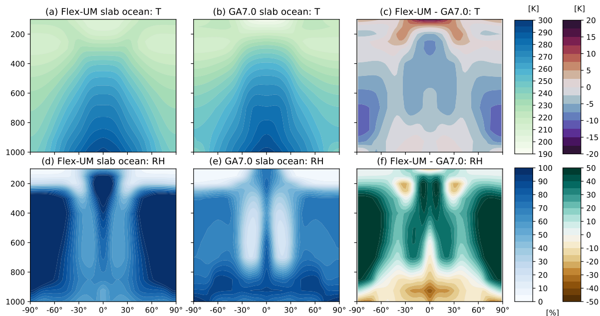
Figure 8. Slab ocean aquaplanet model climatologies for Flex-UM (left) and GA7.0 (middle) for temperature ( T in K , top panel) and relative humidity ( RH as a %, bottom panel) on their native model grids. The differences between the models (Flex-UM - GA7.0) is plotted in the right panels and are interpolated onto the Flex-UM grid. Subplots (a) and (d) are identical to Fig. 2 (a) and (d) but are shown here for ease of comparison.
