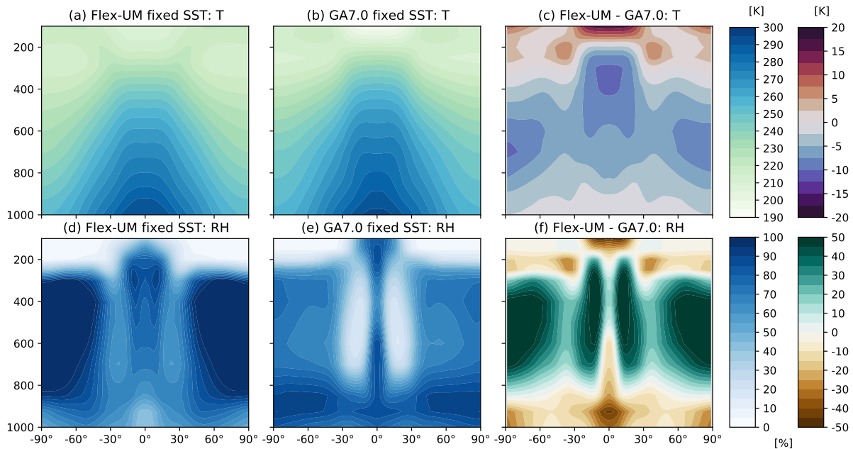
Figure 5. Fixed-SST aquaplanet model climatologies for Flex-UM (left) and GA7.0 (middle) for temperature ( T in K , top panel) and relative humidity ( RH as a %, bottom panel) on their native model grids. The differences between the models (Flex-UM - GA7.0) is plotted in the right panels and are interpolated onto the Flex-UM grid.
