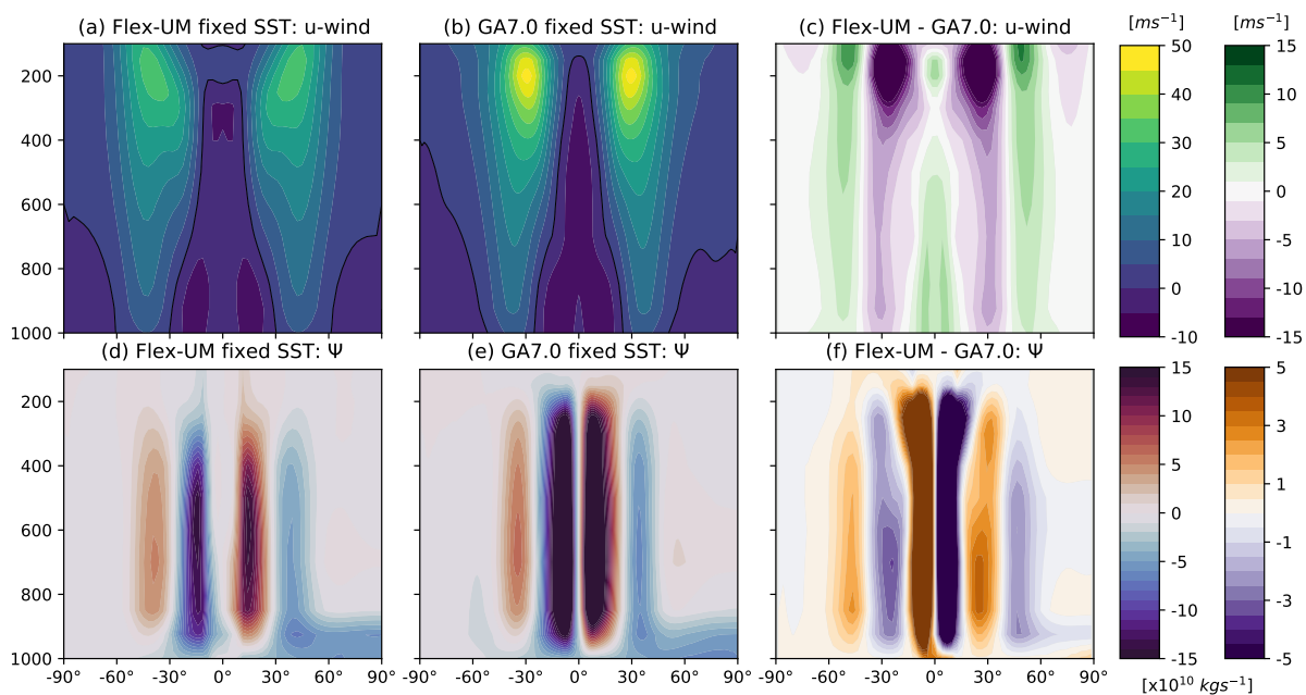
Figure 6. As in Fig. 5 but for zonal-mean zonal wind ( u in ms^{-1} , top panel) and mass stream function ( \Psi in \times 10^{10} kgs^{-1} , bottom panel).
