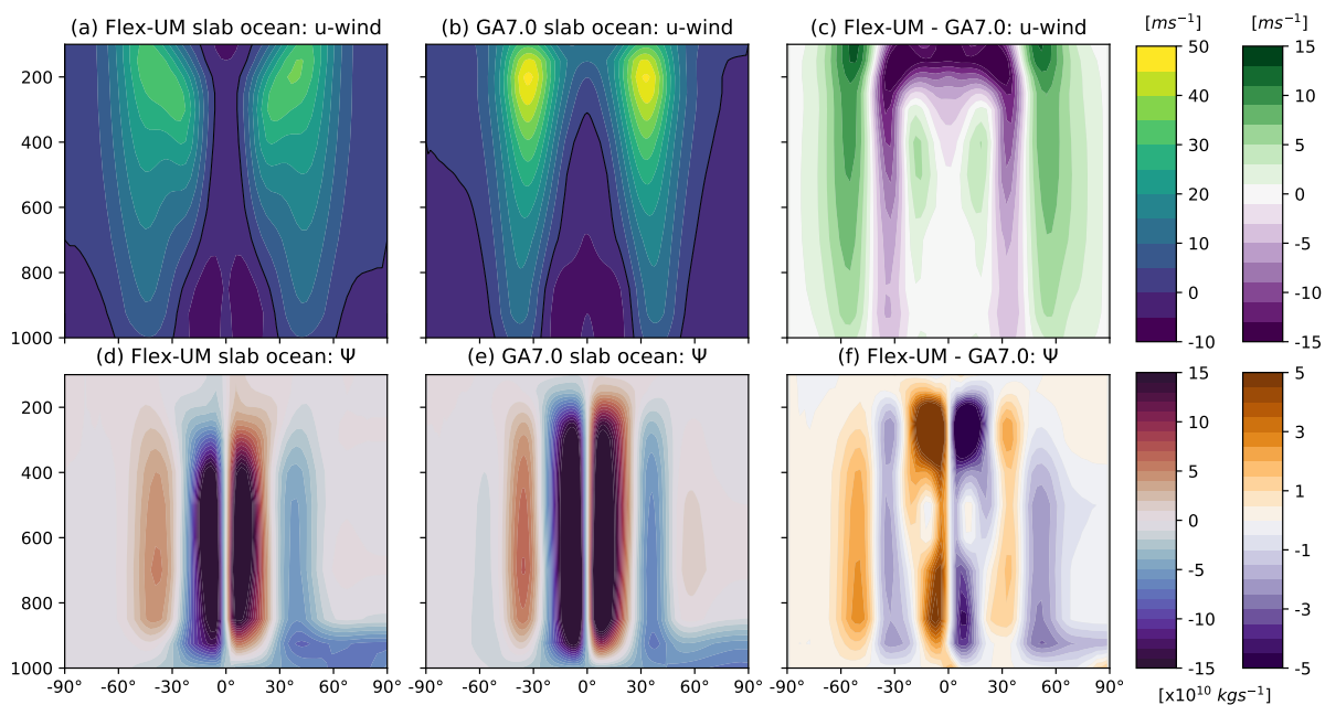
Figure 9. As in Fig. 8 but for zonal-mean zonal wind ( u in ms^{-1} , top panel) and mass stream function ( \Psi in \times 10^{10} kgs^{-1} , bottom panel).
