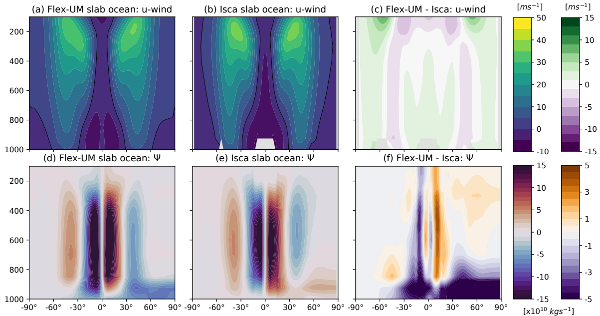
Figure 3. As in Fig. 2 but for zonal-mean zonal wind ( u in ms^{-1} , top panel) and mass stream function ( \Psi in \times 10^{10} kgs^{-1} , bottom panel).
