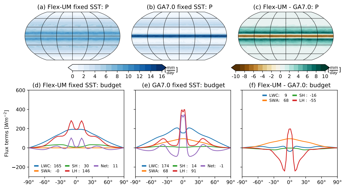
Figure 7. As in Fig. 5 but for precipitation ( P in mm\ day^{-1} , top panel) and the atmospheric energy budget ( Wm^{-2} , bottom panel).
