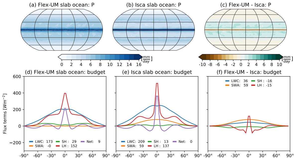
Figure 4. As in Fig. 2 but for precipitation ( P in mm\ day^{-1} , top panel) and the atmospheric energy budget ( Wm^{-2} , bottom panel).
