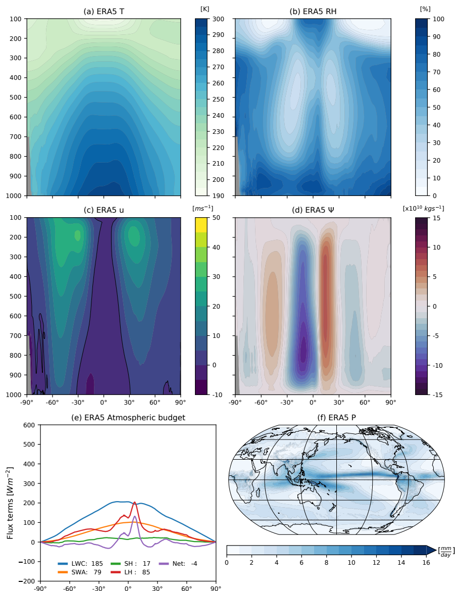
Figure 1. ERA5 reanalysis climatologies for: (a) zonal-mean temperature ( T in K ), (b) zonal-mean relative humidity ( RH as a %), (c) zonal-mean zonal wind ( u in ms^{-1} ), (d) meridional mass stream function ( \Psi in \times 10^{10} kgs^{-1} ), (e) atmospheric energy budget (see Equ. 1 in Wm^{-2} ), and (f) precipitation ( P in mmday^{-1} ). Grey contouring in the SH in subplots (a-d) is data masked where the surface pressure is less than the plotted contour level. The black contour in subplot (c) is the zero wind contour. The legend plotted in subplot (e) are the area weighted global averages.
