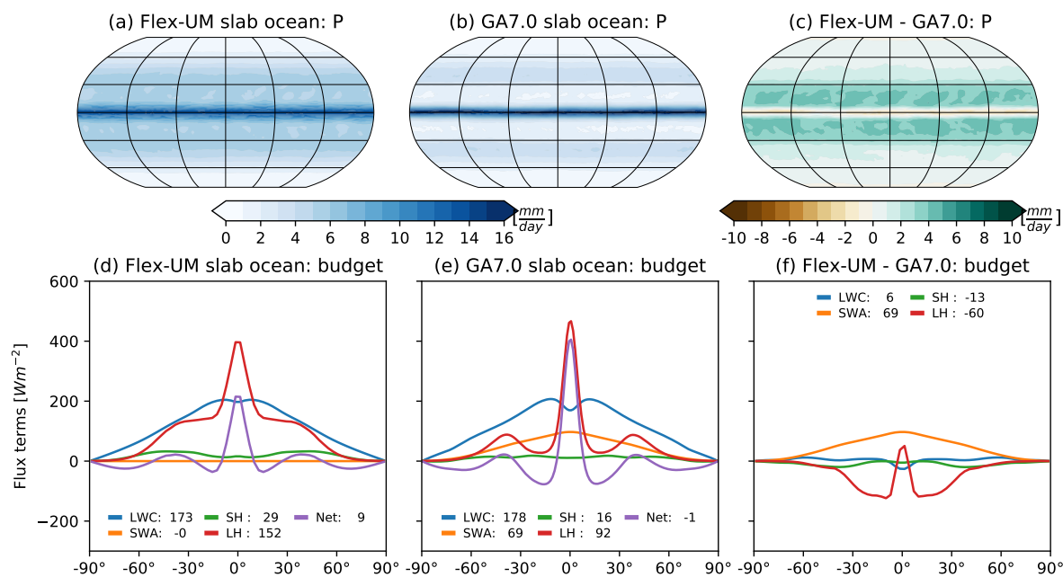
Figure 10. As in Fig. 8 but for precipitation ( P in mmday^{-1} , top panel) and the atmospheric energy budget ( Wm^{-2} , bottom panel).
