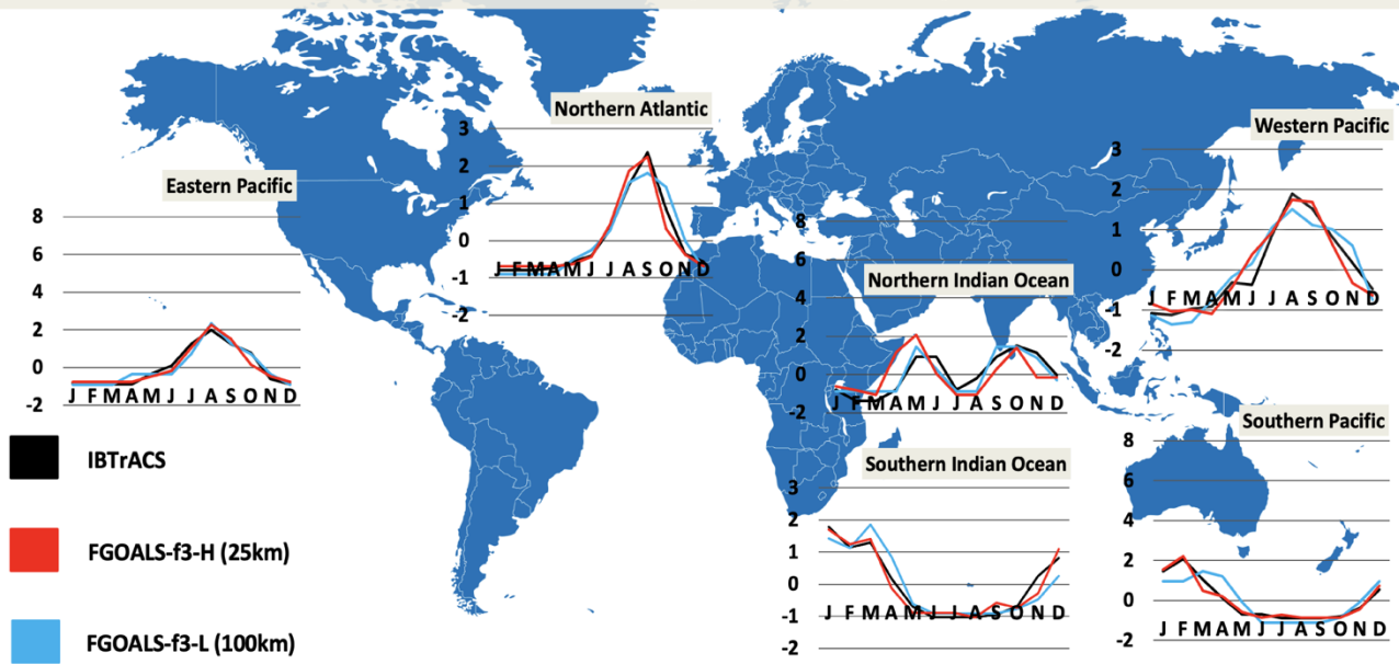
800 Figure S1. Seasonal cycle of tropical cyclones with zero-mean normalization in the western Pacific, southern Pacific, northern Indian, northern Atlantic, southern Indian, and eastern Pacific oceans (units: number of cyclones) during the time period 1991–2014.
