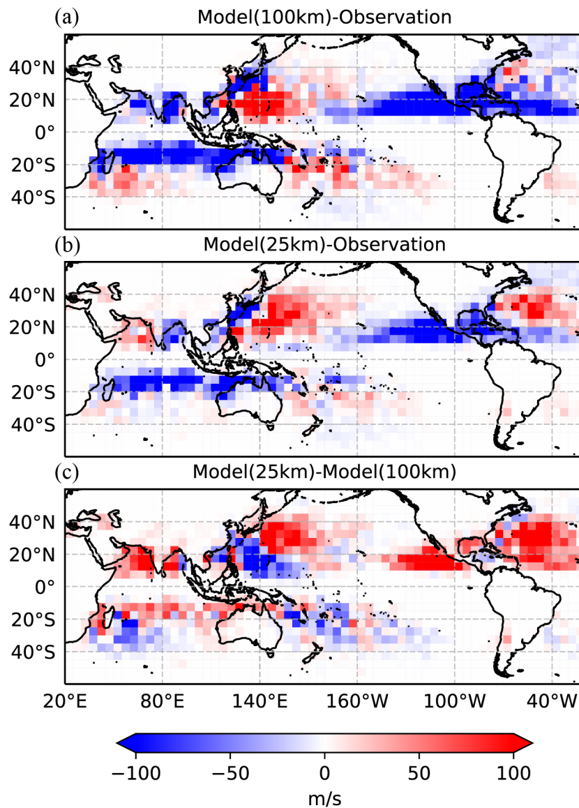
Figure 3. Global maximum sustained wind anomalies of the tropical cyclones (units: \text{m s}^{-1} ). The track density is analyzed in ( 5^\circ \times 5^\circ ) equidistance grid boxes at 6-h intervals. (a) Maximum sustained wind anomalies between FGOALS-f3-L and IBTrACS; (b) maximum sustained wind anomalies between FGOALS-f3-H and IBTrACS; and (c) maximum sustained wind anomalies between FGOALS-f3-H and FGOALS-f3-L.
