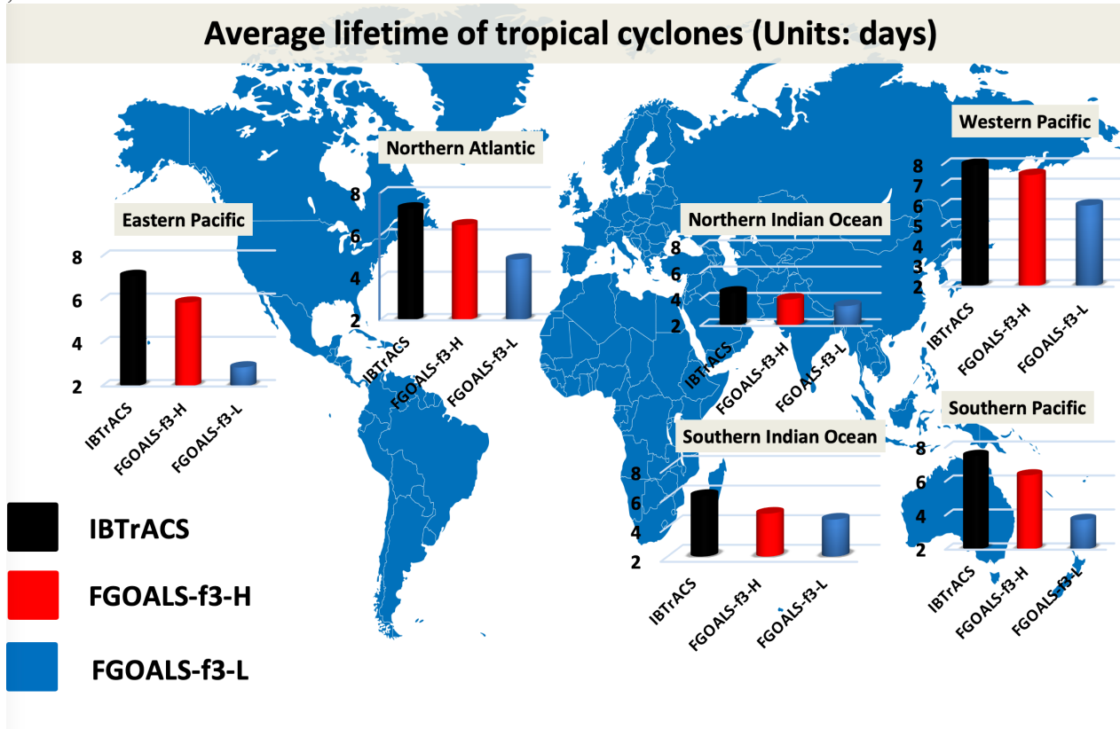
Figure 5. Climatological lifetime of tropical cyclones in the western Pacific, southern Pacific, northern Indian, northern Atlantic, eastern Pacific oceans, and southern Indian oceans (units: days) during the time period 1991–2014.
