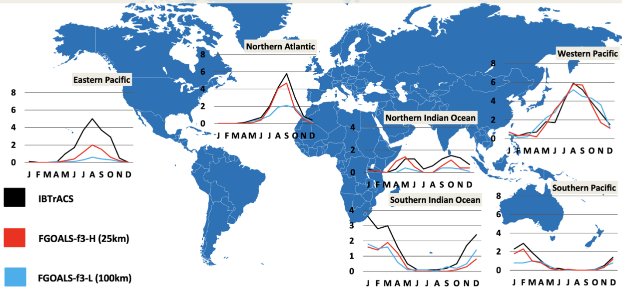
Figure 6. Seasonal cycle of tropical cyclones in the western Pacific, southern Pacific, northern Indian, northern Atlantic, eastern Pacific, and southern Indian oceans (units: number of cyclones) during the time period 1991–2014.
