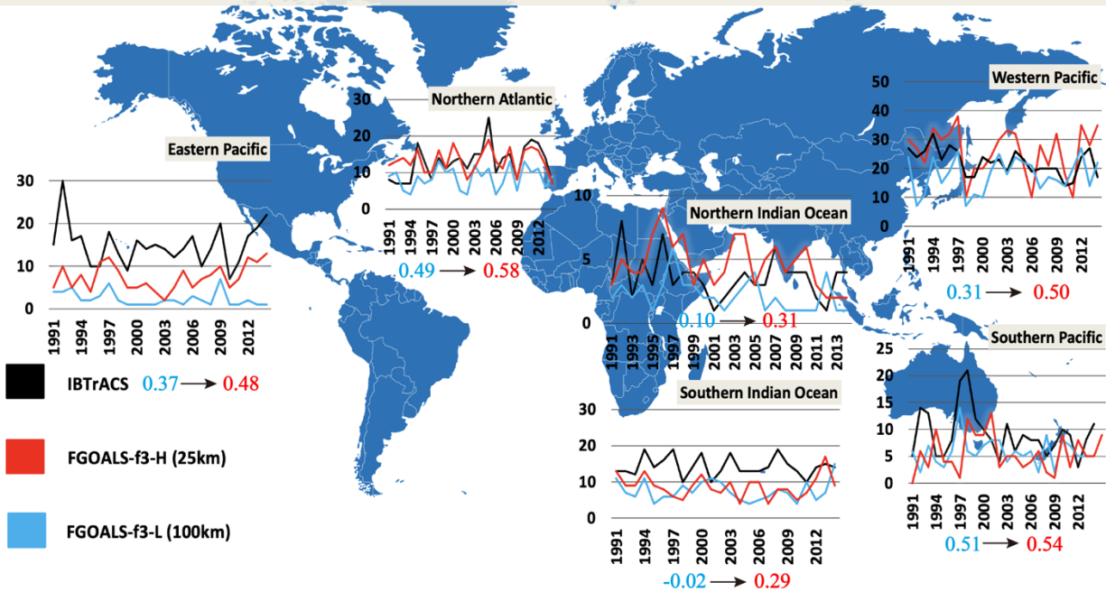
Figure 7. Interannual variability of tropical cyclones in the western Pacific, southern Pacific, northern Indian, northern Atlantic, eastern Pacific, and southern Indian oceans (units: number of cyclones) during the time period 1991–2014. The numbers under the line charts are the correlation coefficients between IBTrACS and FGOALS-f3.
