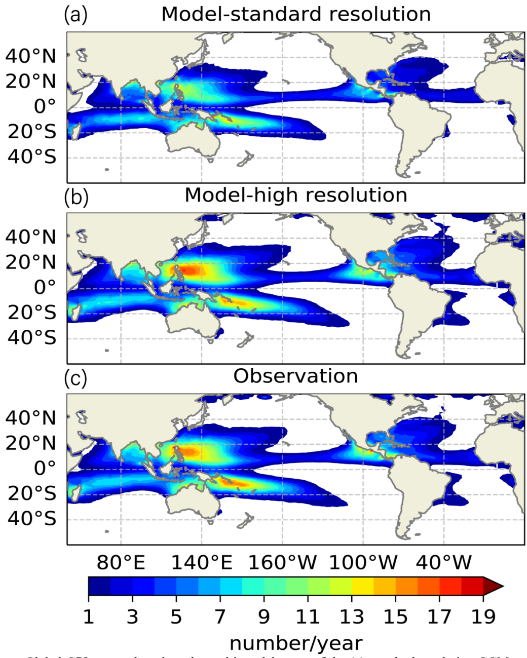
795 Figure 13. Global GPI pattern based on the multi-model mean of the (a) standard-resolution GCMs and (b) high-resolution GCMs and (c) ERA-Interim dataset.
