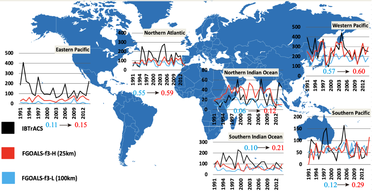
Figure 8. ACE of tropical cyclones (units: 10^4 kt) in the western Pacific, southern Pacific, northern Indian, northern Atlantic, eastern Pacific, and southern Indian oceans (units: number of cyclones) during the time period 1991–2014.
