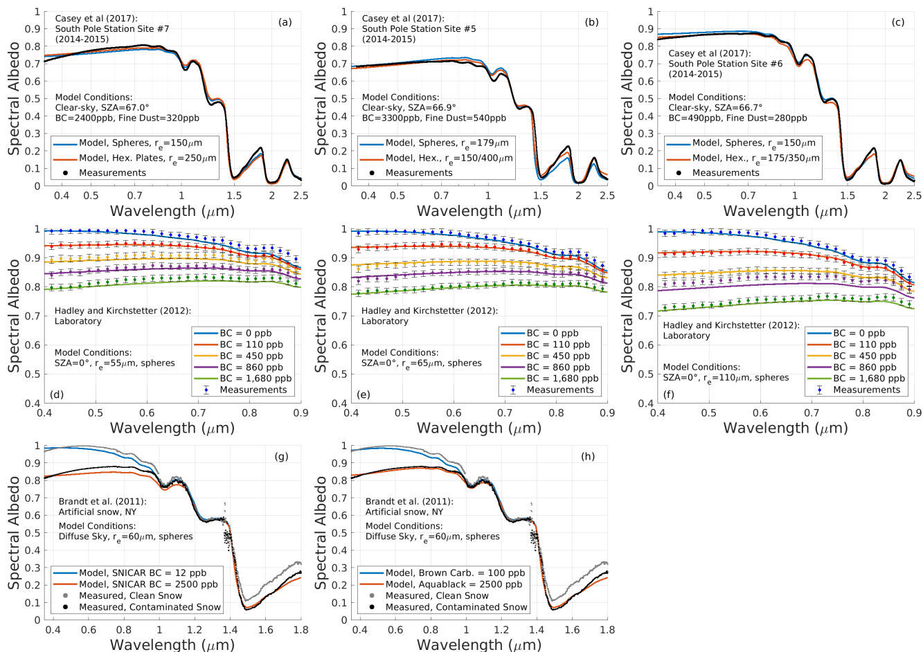
Figure 10. Comparison of modeled spectral snow albedo with measurements from Casey et al. (2017) (a–c), Hadley and Kirchstetter (2012) (d–f), and Brandt et al. (2011) (g–h) of snow contaminated primarily with black carbon. The environmental conditions and model parameters for each setting are listed on the figures and described in the text.
