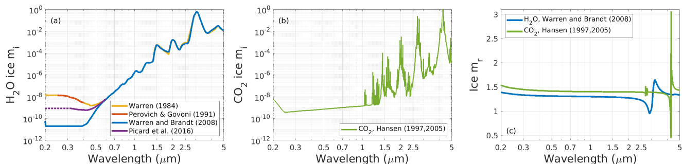
Figure 2. Ice complex refractive index data used in SNICAR-ADv3, including imaginary components ( m_i ) of H 2 O ice (a), imaginary components ( m_i ) of CO 2 ice (b), and real components ( m_r ) of both types of ice (c).
