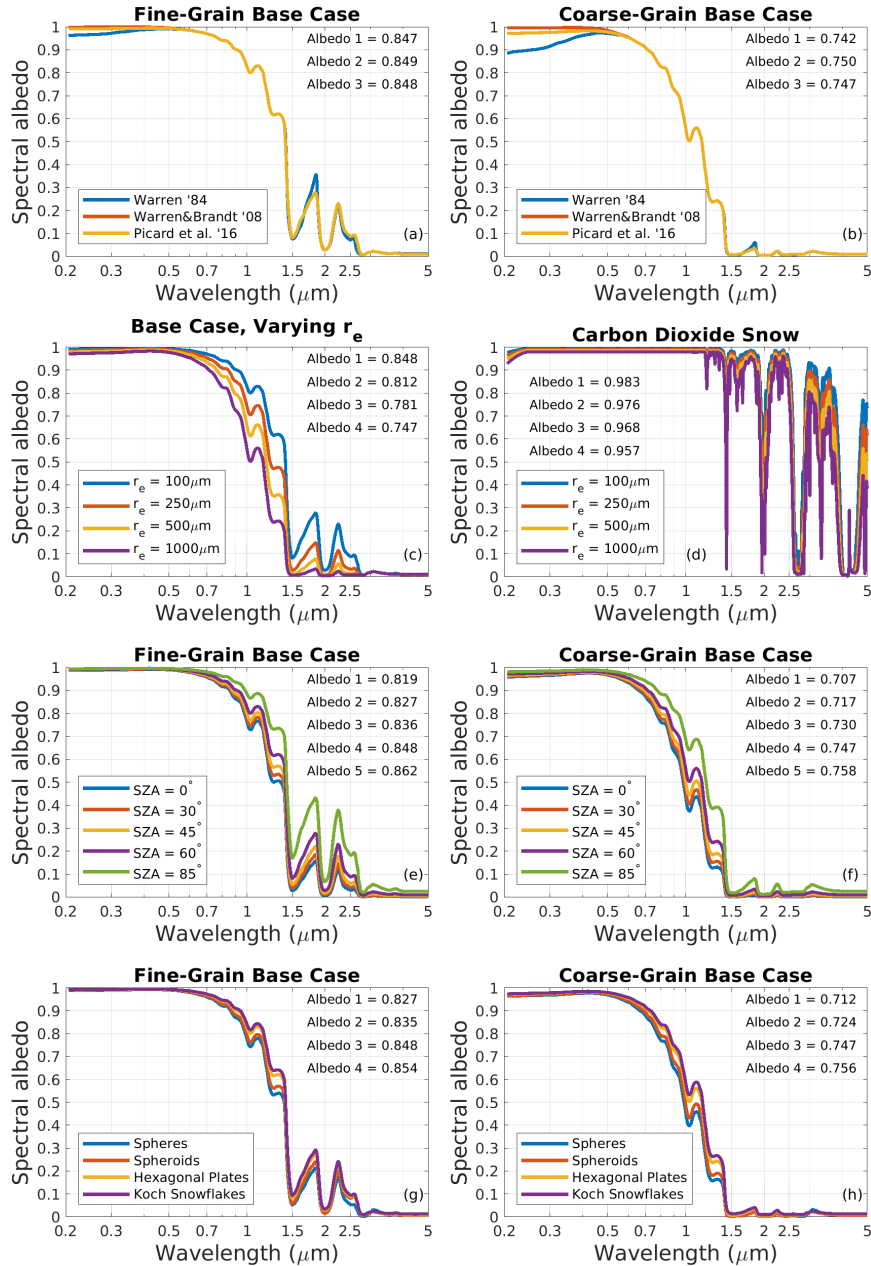
Figure 4. Albedo variations of optically semi-infinite, impurity-free snow in SNICAR-ADV3. Variations are shown for different ice refractive index datasets (a,b,d), ice particle effective grain size (c,d), solar zenith angle (e,f), and ice particle shape (g,h). Except for the parameter being varied, all snowpack properties are those of the fine-grain ( r_e = 100\mu\text{m} ) or coarse-grain ( r_e = 1000\mu\text{m} ) base case defined in Table 3. Solar broadband albedos for each curve are also printed on the figures, with order corresponding to that of the legend.
