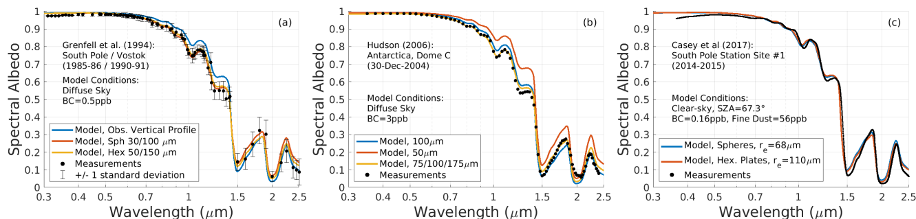
Figure 9. Comparison of modeled spectral snow albedo with measurements from Grenfell et al. (1994) (a), Hudson et al. (2006) (b), and Casey et al. (2017) (c) of very clean snow from Antarctica . The environmental conditions and model parameters for each setting are listed on the figures and described in the text.
