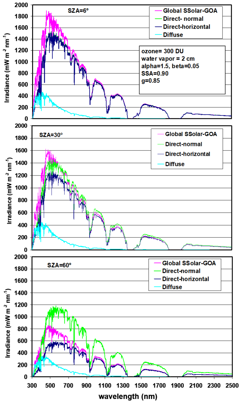
Figure 2: Global, direct normal, direct-horizontal, and diffuse spectral solar irradiances simulated at sea surface level according to the input parameters shown in the figure for SZAs of 6°, 30°, 60°, respectively (from top to bottom).
