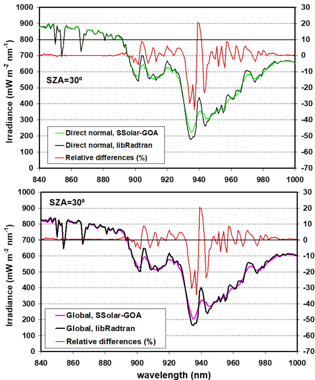
Figure 4: Comparison between libRadtran and SSolar-GOA models in the region of the 940 nm absorption band of water vapour for direct normal (top) and global (bottom) solar irradiances at SZA=30°.
