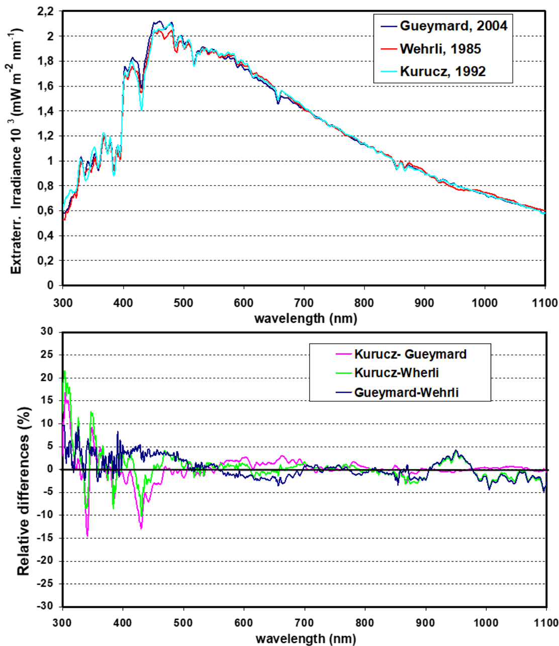
Figure 10: Comparison between the extraterrestrial solar irradiance spectra given by Gueymard, Wehrli, and Kurucz (see references) convoluted with a spectral triangular slit function of FWHM of 11 nm.
