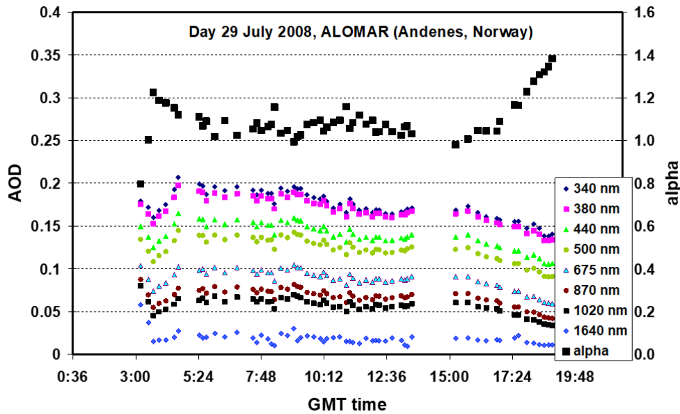
730 Figure 12: Time evolution of AOD at different wavelengths and alpha parameter on 29 July 2008 at Andenes (Andøya, Norway).
