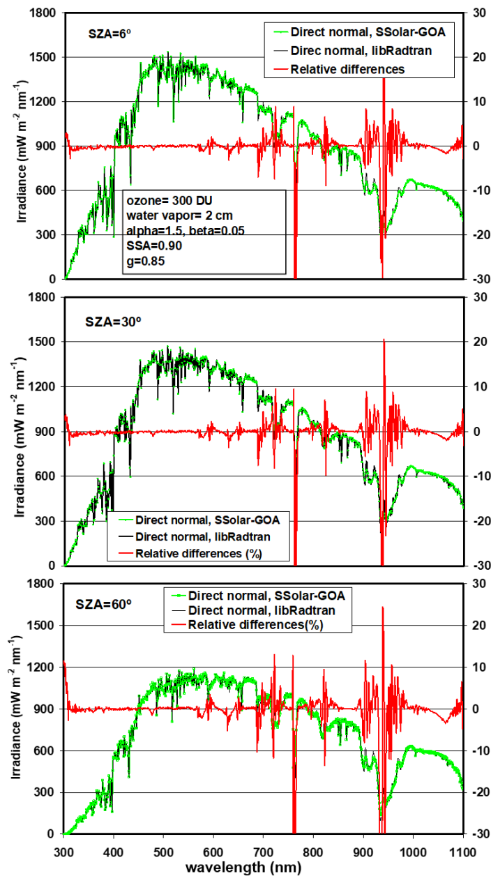
Figure 3: Comparison between libRadtran and SSolar-GOA models for direct normal irradiance at SZA= 6°, 30°, and 60° respectively (from top to bottom), with input parameters shown at the top of the figure. Right Y axis indicates the relative differences in % in all figures (libRadtran minus SSolar-GOA/libRadtran).
