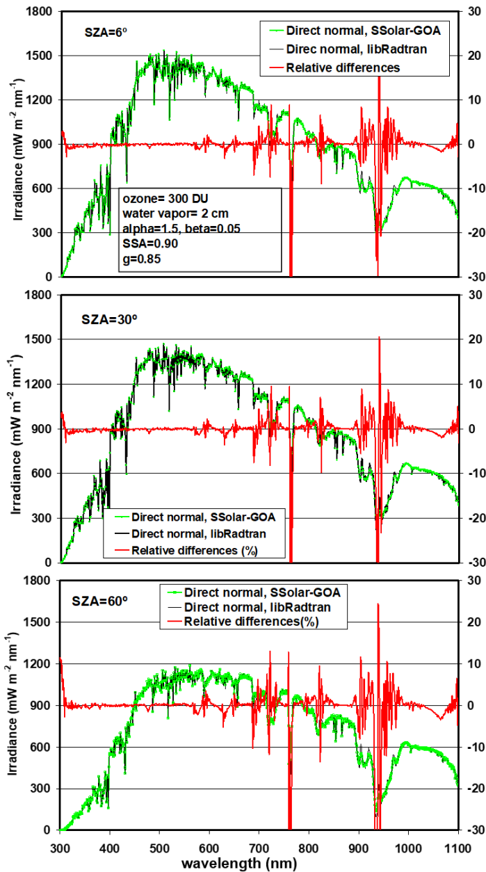
Figure_32: Comparison between libRadtran and SSolar-GOA models for direct normal irradiance at SZA= 6°, 30°, and 60° respectively (from top to bottom), with input parameters shown at the top of the figure. Right Y axis indicates the relative differences in % in all figures (libRadtran minus SSolar-GOA/libRadtran).
