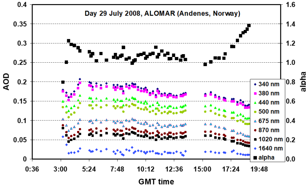
765 Figure 11 Figure 12 : Time evolution of AOD at different wavelengths and alpha parameter on 29 July 2008 at Andenes (Andøya, Norway).
