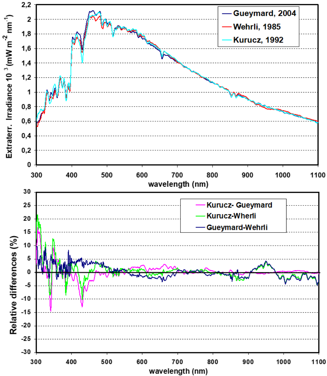
[730] Figure-Figure 109 : Comparison between the extraterrestrial solar irradiance spectra given by Gueymard, Wehrli, and Kurucz (see references) convoluted with a spectral triangular slit function of FWHM of 11 nm.
