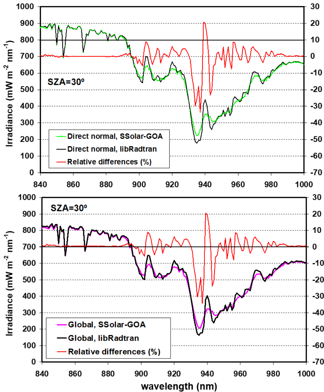
Figure 43: Comparison between libRadtran and SSolar-GOA models in the region of the 940 nm absorption band of water vapour for direct normal (top) and global (bottom) solar irradiances at SZA=30°.
