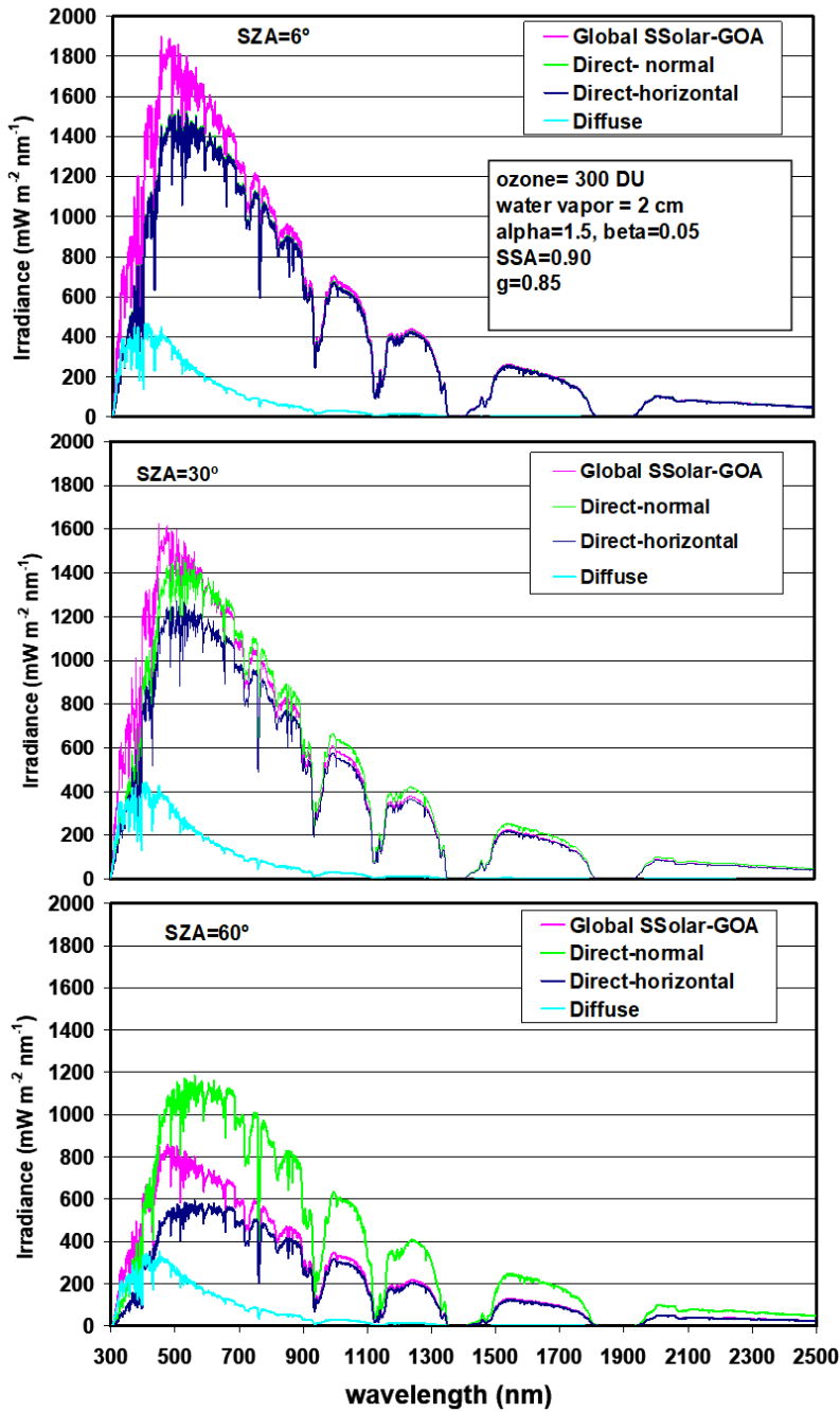
Figure -24: Global, direct normal, direct-horizontal, and diffuse spectral solar irradiances simulated at sea surface level according to the input parameters shown in the figure for SZAs of 6°, 30°, 60°, respectively (from top to bottom).
