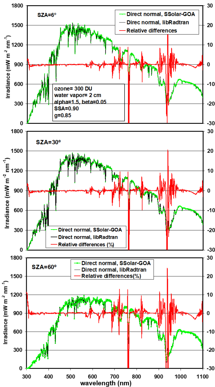
Figure 2: Comparison between the libRadtran and SSolar-GOA models for direct normal irradiance at SZA= 6°, 30°, and 60° respectively (from top to bottom), with input parameters shown at the top of the figure. Right Y axis indicates the relative differences in % in all figures (libRadtran minus SSolar-GOA/libRadtran).
