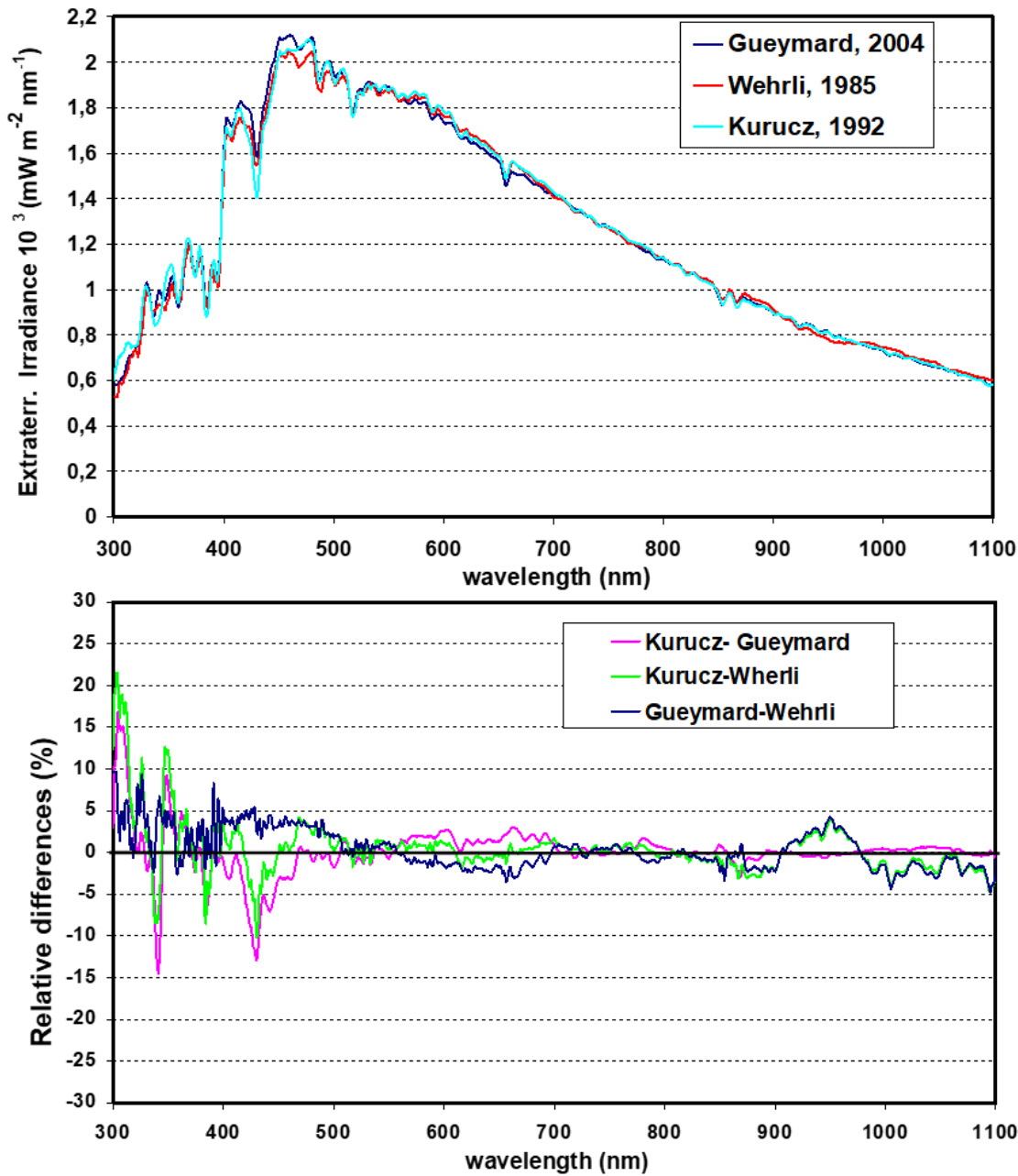
Figure 9: Comparison between the extraterrestrial solar irradiance spectra given by Gueymard, Wehrli, and Kurucz (see references) convoluted with a spectral triangular slit function of FWHM of 110 nm.
