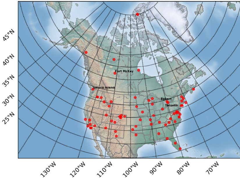
470 Figure 4: North American AERONET Sites. AOD data from these stations are used in this study.
