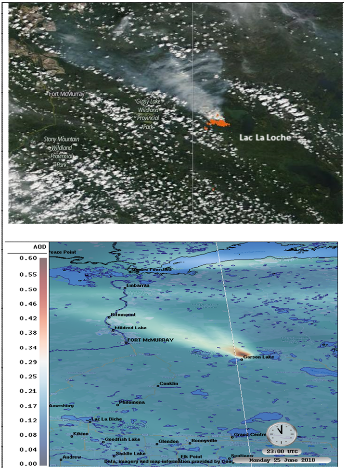
Figure 13: : Lac La Loche forest fire on June 25, 2018. Top : Overlay layer: MODIS-Terra thermal anomalies (day and night), over MODIS Terra true color corrected reflectance (Image from: https://worldview.earthdata.nasa.gov ). Bottom: GEM-MACH AOD at 580 nm at 23:00 UTC.
