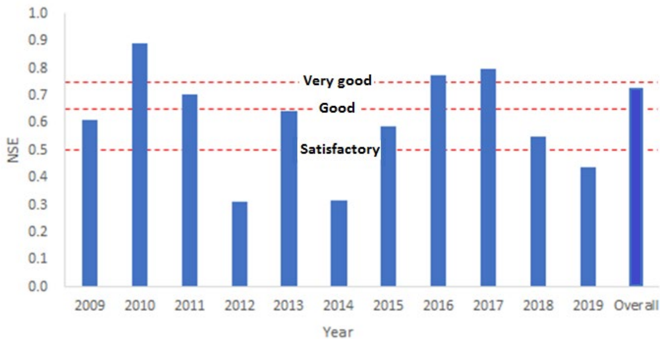
Figure 5. NSE score of modelling daily flow in the lower basin using TOPMODEL summarised by year.
