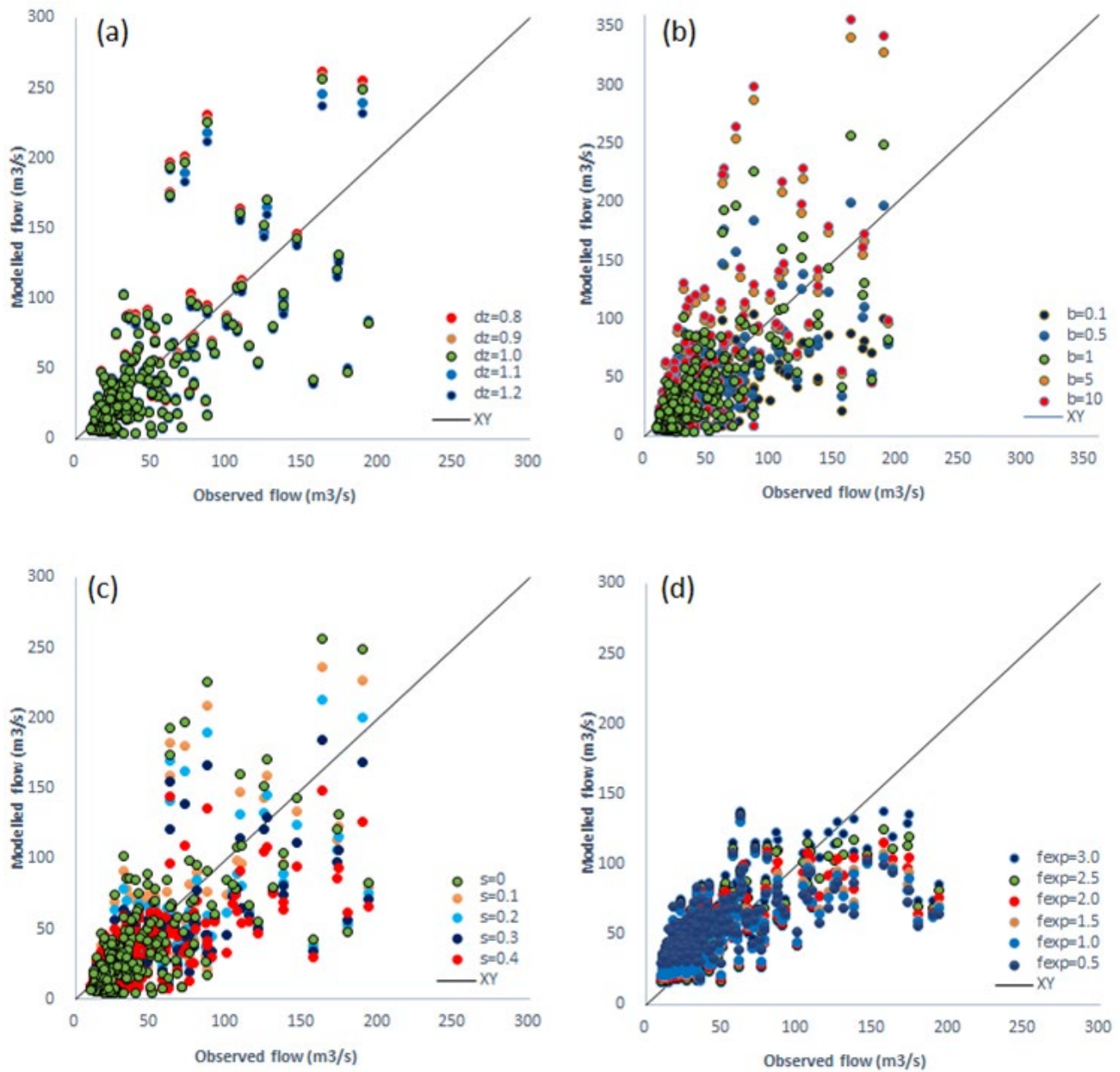
275 Figure 2. Sensitivity analysis of daily mean flow in the lower basin with a) soil depth b) shape factor c) threshold of minimum soil water content, using PDM, d) decay parameters, using TOPMODEL.
