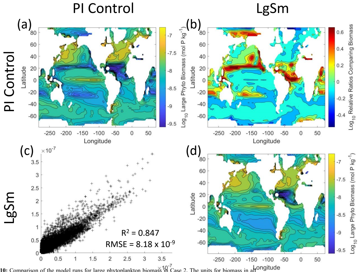
Figure 10: Comparison of the model runs for large phytoplankton biomass in Case 2. The units for biomass in all subplots are mol P kg -1 . The subplots show point-by-point scatter plots comparing the model runs against one another (c), yearly averaged log 10 biomass plots for each model run (a and d), and the log 10 relative ratios comparing the yearly averaged contour plots of the model runs (b). The x-axis and y-axis of the scatter plots (c) correspond to the horizontal/vertical model run labels, respectively (e.g., box (c) shows PI Control on the x-axis and LgSm on the y-axis). The yearly averaged log 10 contour plots (a and d) correspond to the matching horizontal/vertical model run labels (e.g., box (a) shows the yearly averaged log 10 biomass of PI Control). The log 10 relative ratios (b) were calculated as the model run listed on the horizontal axis divided by the model run listed on the vertical axis (e.g., box (b) shows LgSm divided PI Control).
