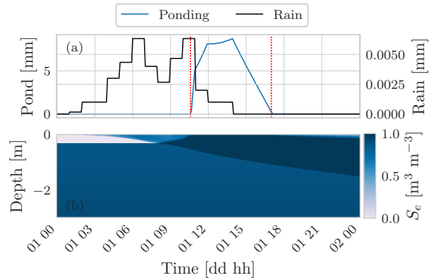
Figure C11. Panel (a) shows the rainfall and the water ponding at the soil surface. Initially rainfall can infiltrate into the soil and no water builds up at the soil surface. As the uppermost layer of the soil saturates water starts ponding at the soil surface. The dotted red lines indicate the times at which the boundary condition at the soil surface should be switched. Panel (b) shows the time evolution of the saturation degree within the soil.
