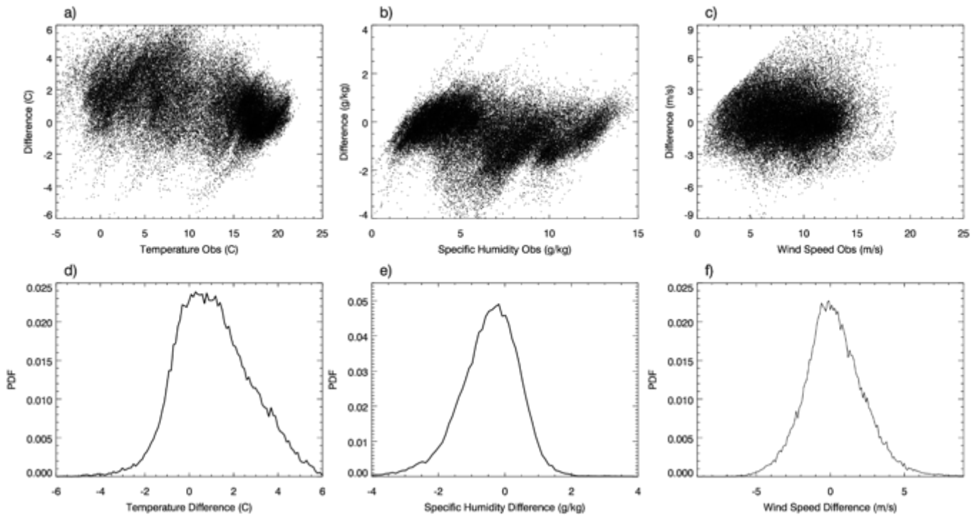
780 Figure 5. Scatter plot for GPM-retrieved observation vs. the departure between the observation and the model background for a) 2-m temperature [°C], b) 2-m specific humidity [g kg -1 ], and c) 10-m horizontal wind speed [m s -1 ] from all available data during the data assimilation time windows for the two case studies. Probability density function (PDF) of the d) 2-m temperature departure, b) 2-m specific humidity departure, and c) 10-m horizontal wind speed departure with bin width of 0.1.
