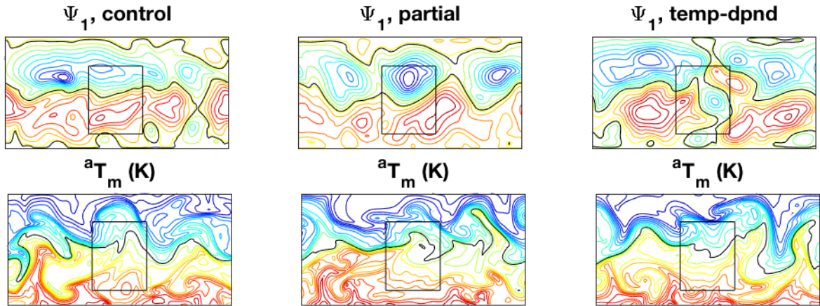
Figure 3: Atmospheric snapshots from the three simulations. Top: lower-layer streamfunction; bottom row: a.m.l. temperature perturbation, CI=2 K. Black curves show zero contour.
