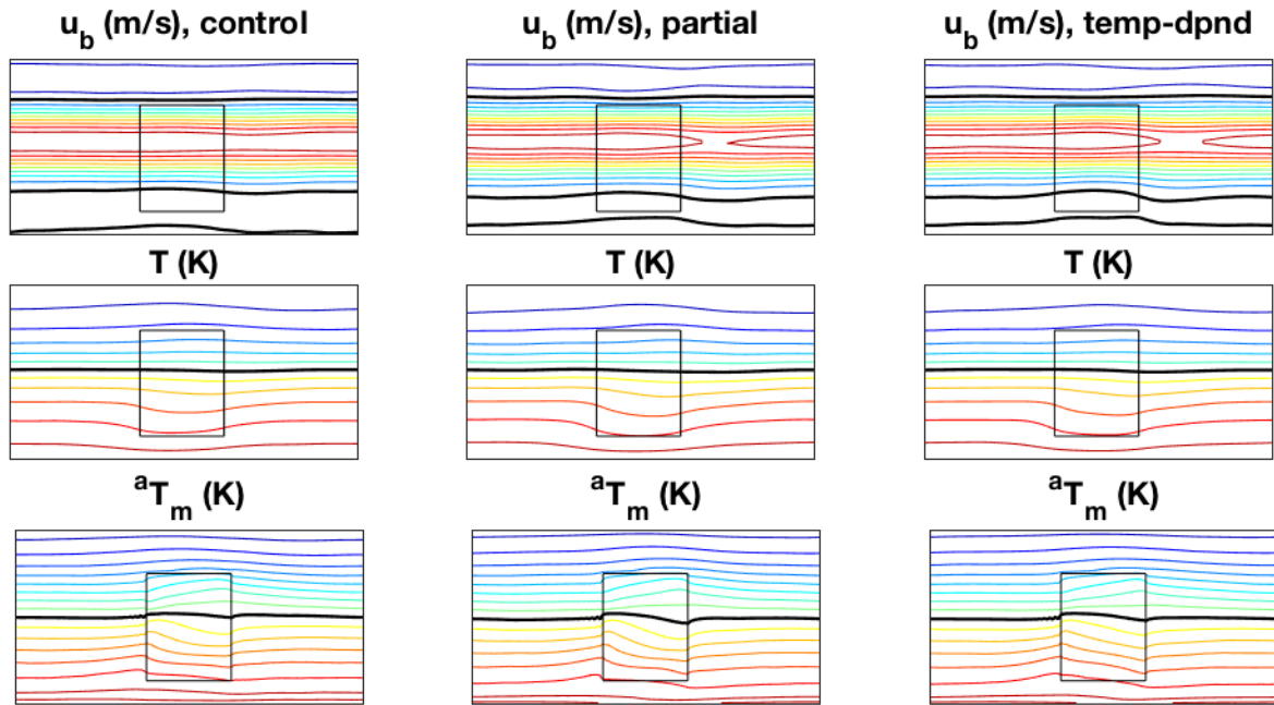
835 Figure 2: Atmospheric mean state (continued). Top: barotropic zonal wind, CI=2 m s -1 ; middle row: interior temperature perturbation according to Eq. (12), CI=2 K; bottom: a.m.l. temperature, CI=2 K.
