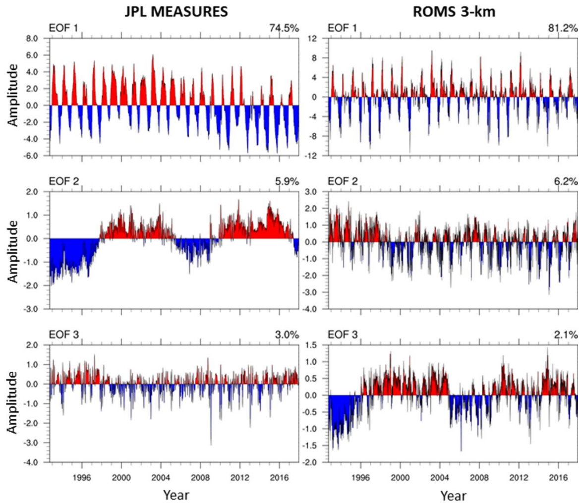
990 Figure 3. Time series of the amplitudes associated with the main three normalized spatial EOF components derived during the 1993-2017 period from the SSHA from the JPL MEASURES gridded product (left panels) and the SSH results of the AdriSC ROMS 3-km model (right panels).
