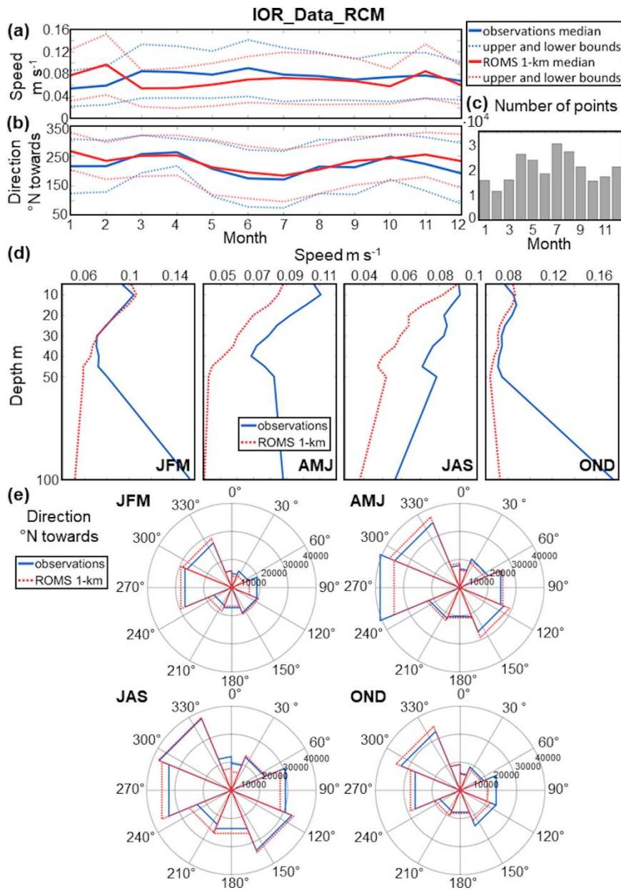
Figure 14. IOR_Data_RCM dataset. Monthly climatology of AdriSC 1-km and in situ (a) median speed, (b) median direction and their variabilities (i.e. upper and lower bounds defined as \pm \text{MAD} ) as well as (c) number of observations per month. Seasonal variations of the (d) speed of AdriSC ROMS 1-km model and observations depending on the depth. Seasonal rose plots of the (e) direction for RCM observations and the AdriSC ROMS 1-km model.
