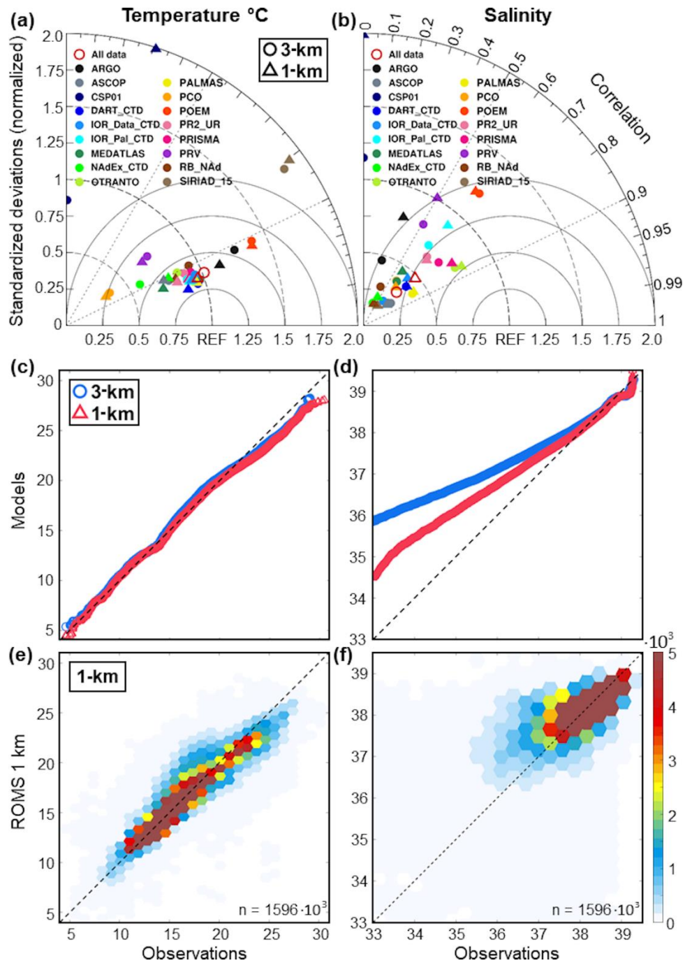
1000 Figure 6. Evaluation of the AdriSC ROMS 3-km and 1-km temperature (left panels) and salinity (right panels) results against observations from 17 different datasets with (a, b) Taylor diagrams and (c, d) quantile–quantile plots as well as, only for the 1-km model, (e, f) scatter plots showing the density (number of occurrences) with hexagonal bins and total number of points n .
