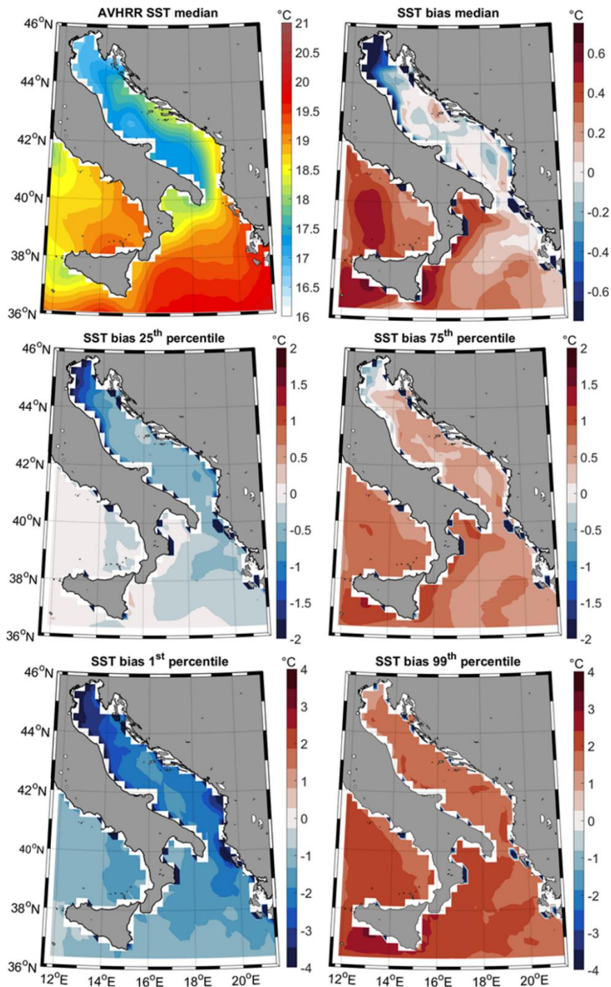
995 Figure 4. Median of the AVHRR daily sea-surface temperature product (top left panel) as well as median (top right panel) and 25 th (centre left panel), 75 th (centre right panel), 1 st (bottom left panel), 99 th (bottom right panel) percentiles of the daily sea-surface temperature biases between AdriSC ROMS 3-km model results and AVHRR product during the 1987-2017 period.
