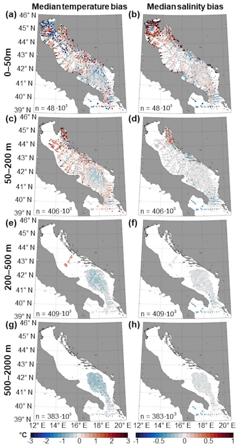
1005 Figure 7. Median of the temperature (left panels) and salinity (right panels) biases between AdriSC ROMS 1-km model results and CTD observations for depth ranges: (a, b) 0-50 m, (c, d) 50-200 m, (e, f) 200-500 m, (g, h) 500-2000 m, with the total number of points n (bottom left corner).
