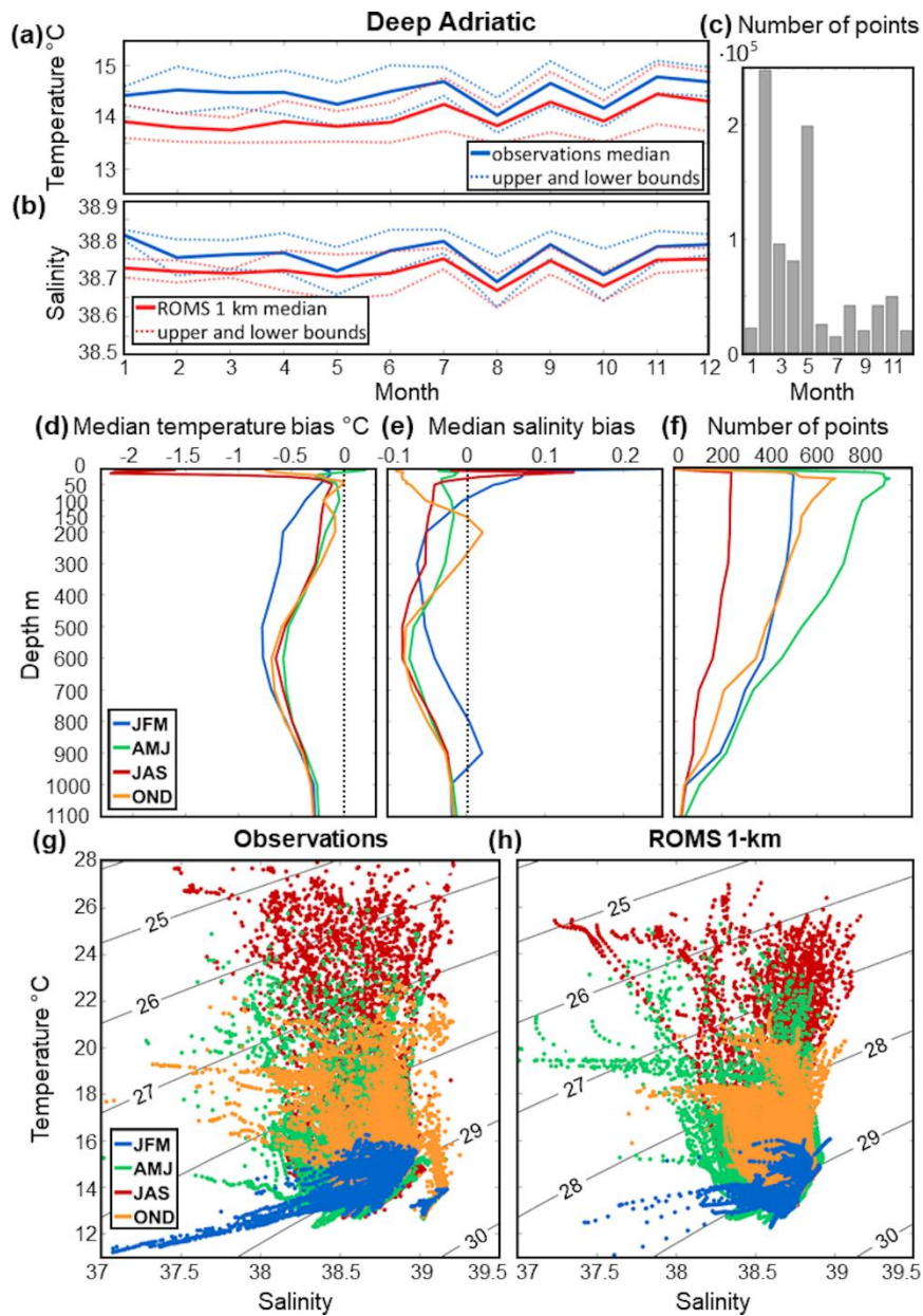
1020 Figure 10. Deep Adriatic subdomain. Monthly climatology of AdriSC 1-km and in situ (a) median temperature, (b) median salinity and their variabilities (i.e. upper and lower bounds defined as \pm MAD) as well as (c) number of observations per month. Seasonal variations of the (d) temperature and (e) salinity biases between the AdriSC ROMS 1-km model and observations depending on the depth as well as (f) number of observations per depth. Seasonal T-S diagrams for (g) the CTD observations and (h) the AdriSC ROMS 1-km model with PDA isolines.
