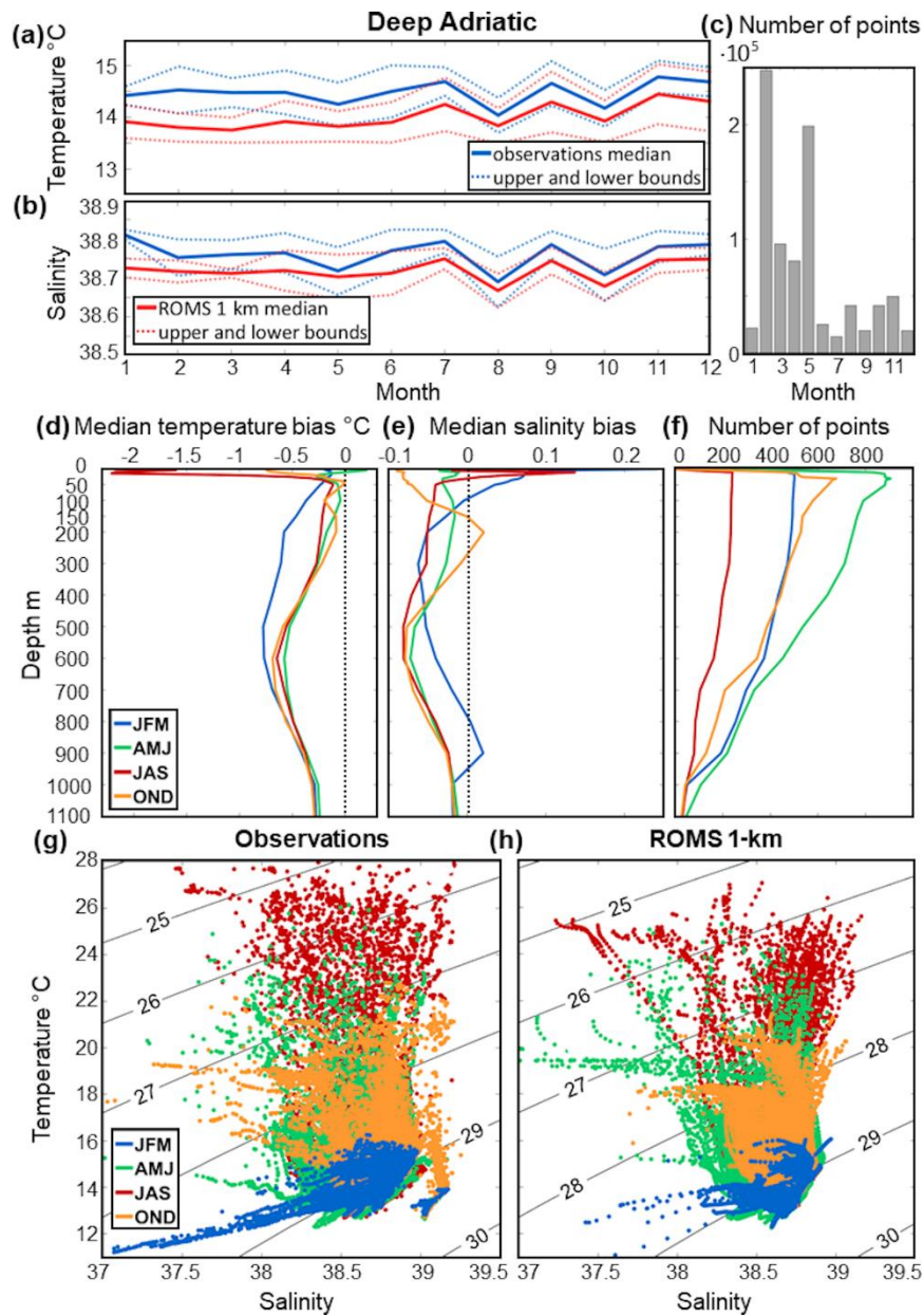
1030 Figure 10. Deep Adriatic subdomain. Monthly climatology of AdriSC 1-km and in situ (a) median temperature, (b) median salinity and their variabilities (i.e. upper and lower bounds defined as \pm MAD) as well as (c) number of observations per month. Seasonal variations of the (d) temperature and (e) salinity biases between the AdriSC ROMS 1-km model and observations depending on the depth as well as (f) number of observations per depth. Seasonal T-S diagrams for (g) the CTD observations and (h) the AdriSC ROMS 1-km model with PDA isolines.
