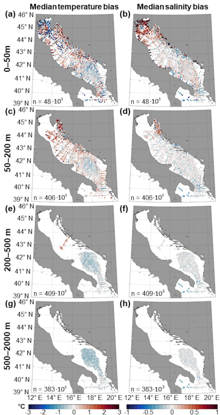
1015 Figure 7. Median of the temperature (left panels) and salinity (right panels) biases between AdriSC ROMS 1-km model results and CTD observations for depth ranges: (a, b) 0-50 m, (c, d) 50-200 m, (e, f) 200-500 m, (g, h) 500-2000 m, with the total number of points n (bottom left corner).
