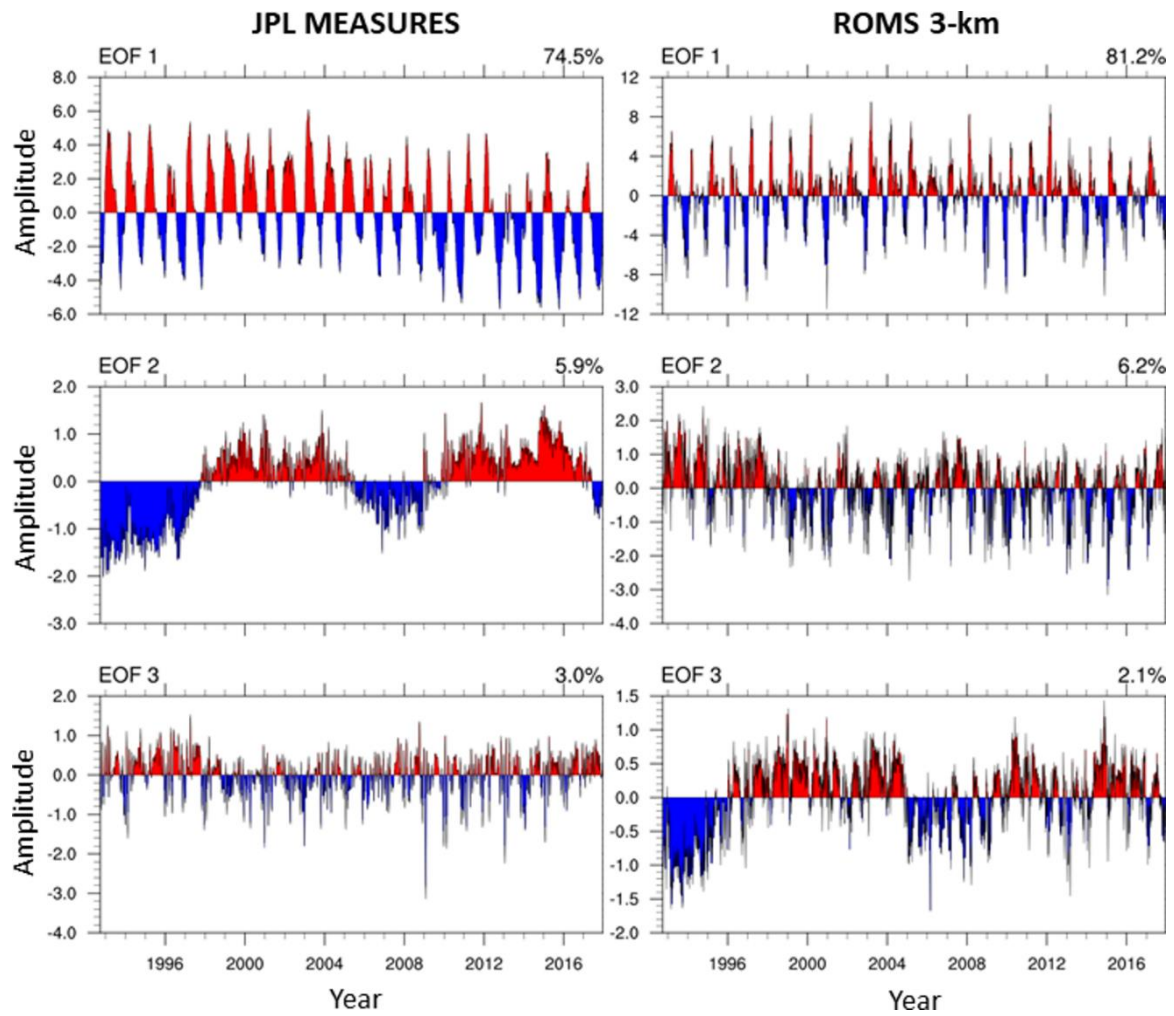
1000 Figure 3. Time series of the amplitudes associated with the main three normalized spatial EOF components derived during the 1993-2017 period from the SSHA from the JPL MEASURES gridded product (left panels) and the SSH results of the AdriSC ROMS 3-km model (right panels).
