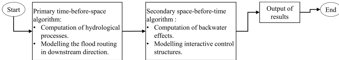
660 Figure 9: Structure of the implemented primary and secondary algorithm in the source code of Kalypso-NA (4.0). The enhancement of the primary algorithm is published in (Hellmers and Fröhle, 2017). The new (secondary) algorithm is explained in section 4.3.
