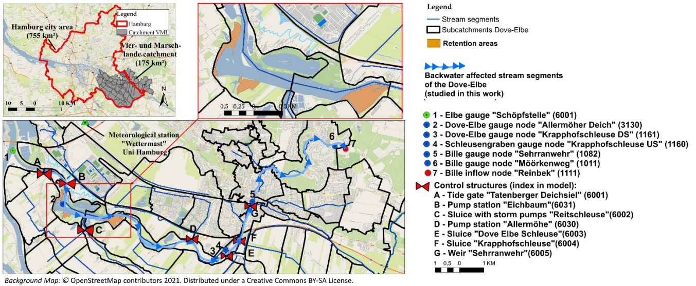
665 Figure 10: Map of the application study area ‘Vier- und Marschlande’ (175 km 2 ): subcatchments, gauging stations (1 to 7), studied backwater affected streams of the Dove-Elbe, three retention areas in the main stream and control structures (A to G).
