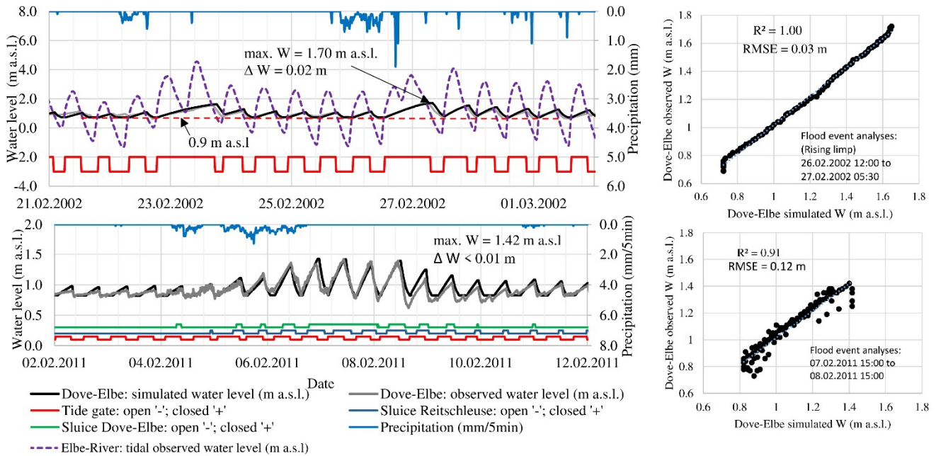
670 Figure 11: Closure and opening state of the control structures as well as simulated and observed water levels at the downstream gauge ‘Allermöher Deich’ for the event February 2002 and February 2011. The tide gate remained closed two times during the storm events in February 2002. Meaning, the Elbe River water level during low tide period did not fall below the required minimal water level of 0.9 m a.s.l. The simulated and observed water levels depict a difference of 0.02 m to 0.01 m in a stream with a water table fluctuation of about 1 m. The RMSE for the flood event analysis shows a deviation of up to 0.12 m.
