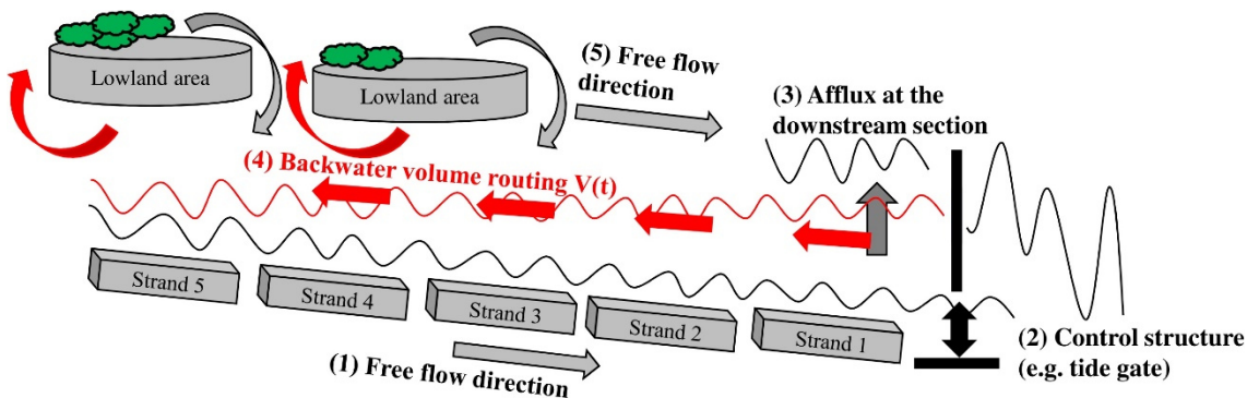
625 Figure 2: Scheme of five computation steps in the developed concept to compute backwater effects with a hydrological approach: (1) free flood routing computation downstream, (2) control structure simulation, (3) afflux computation, (4) backwater volume routing computation in upstream direction including adjacent lowland areas (as well as retention areas) and (5) free flood routing computation after opening the barrier.
