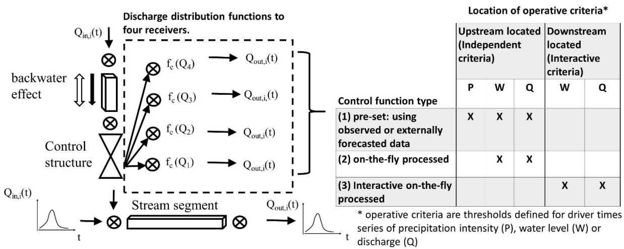
Figure 4: Scheme of a control structure with discharge distribution functions to four receivers and the three control function types depending on operative criteria.
