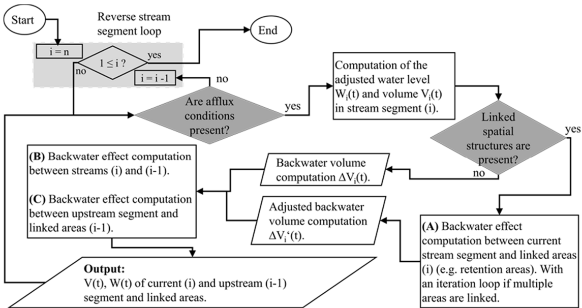
655 Figure 8: Computation of the upstream directed backwater effect over stream segments and adjacent lowland areas (e.g. retention areas). Illustrated details of the second calculation routine (b) of the algorithm in Fig. 5.
