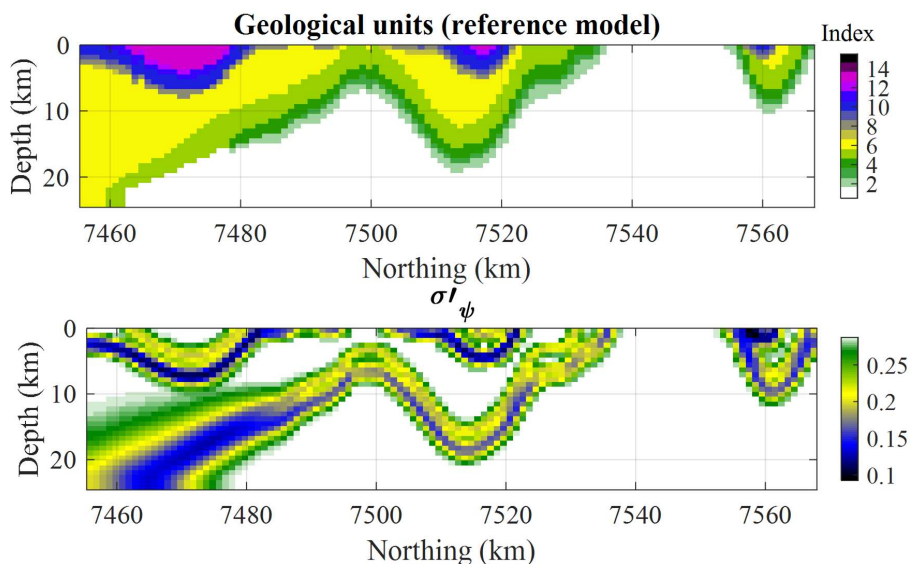
440 Figure 6. Two-dimensional slice extracted from the 3D model along the profile: geological reference model (top), the \sigma_\psi metric (bottom). Here, the geological uncertainty metric considered is the standard deviation of the probability of the different lithologies as per equation 18.
