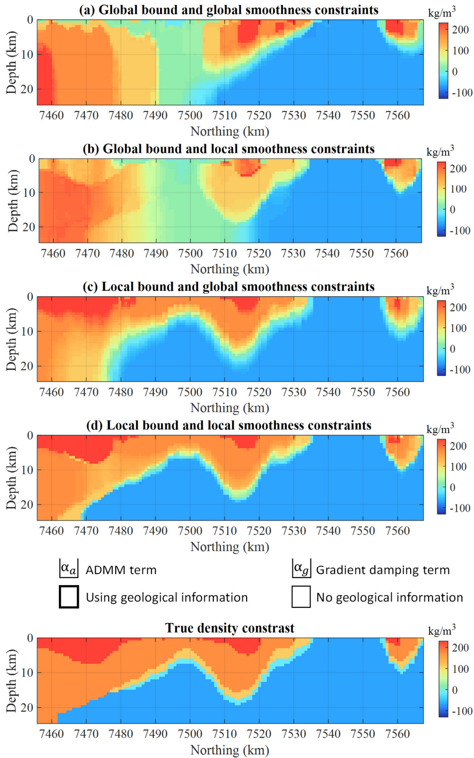
Figure 16. Results from gravity inversion using: (a) global ADMM clustering and homogenous smoothness constraints, (b) global ADMM clustering and geologically-derived smoothness constraints, (c), ADMM clustering and geologically-derived smoothness constraints, and (d) geologically-derived ADMM clustering and geologically-derived smoothness constraints. For visual comparison, the true model is reminded at the bottom of the Figure.
