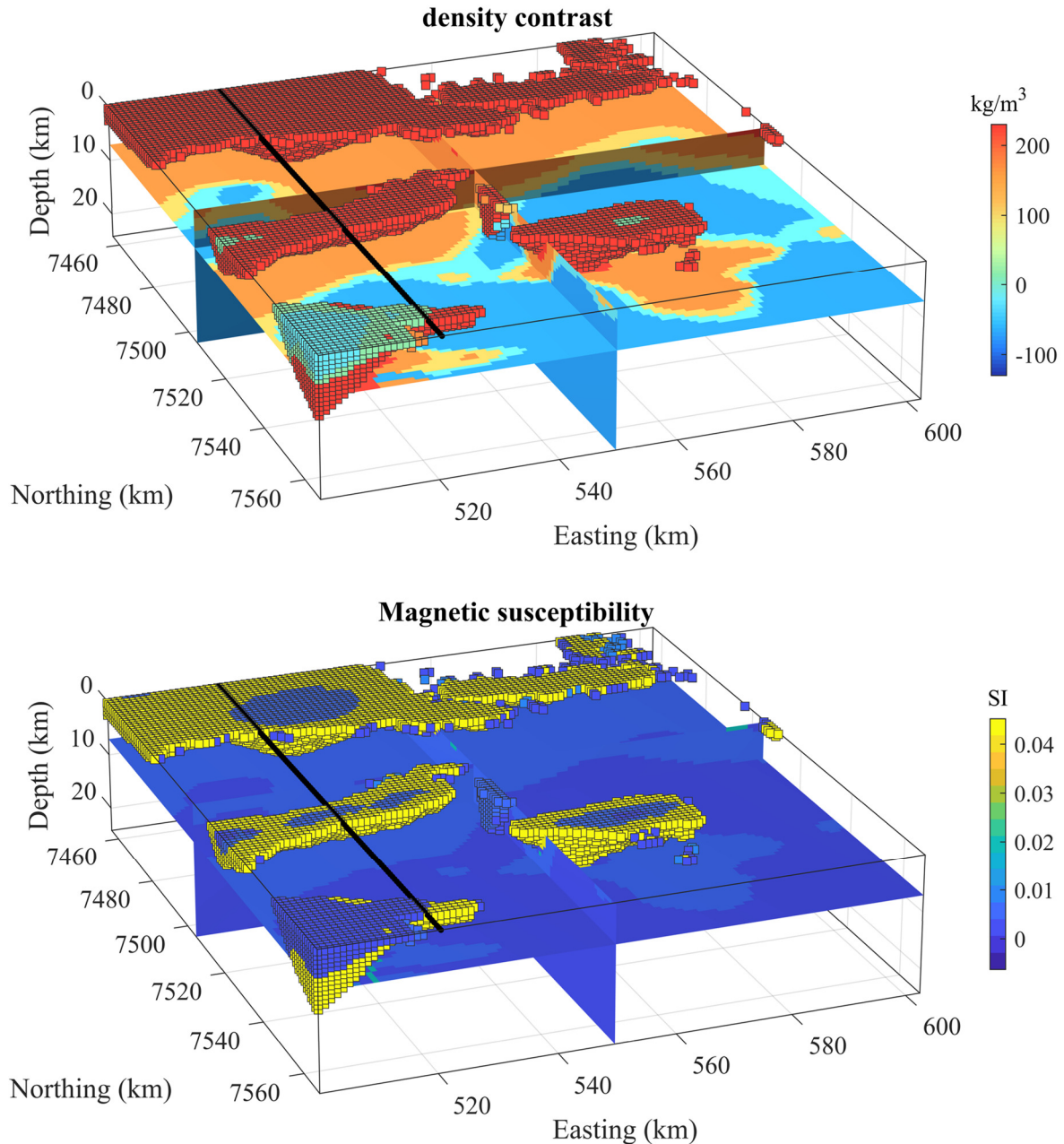
Figure 3. True synthetic density contrast (top) and magnetic susceptibility (bottom) model used for the simulation of geophysical data. The black line represents the surface coordinates of the 2D profile considered here. The voxels represent lithologies 10 through 15, color-coded with their respective density contrast and magnetic susceptibility values.
