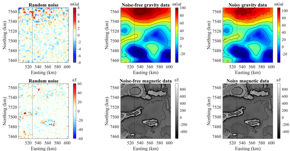
Figure 4. Noise (left hand side column) added to the data calculated from the true model (central column) and resulting noisy data (right hand side) for the gravity (top) and magnetic (bottom) datasets. The contour lines shown corresponding to the ticks shown in the palette's colour bar. The black line represents the location profile we use for the inversions performed here.
