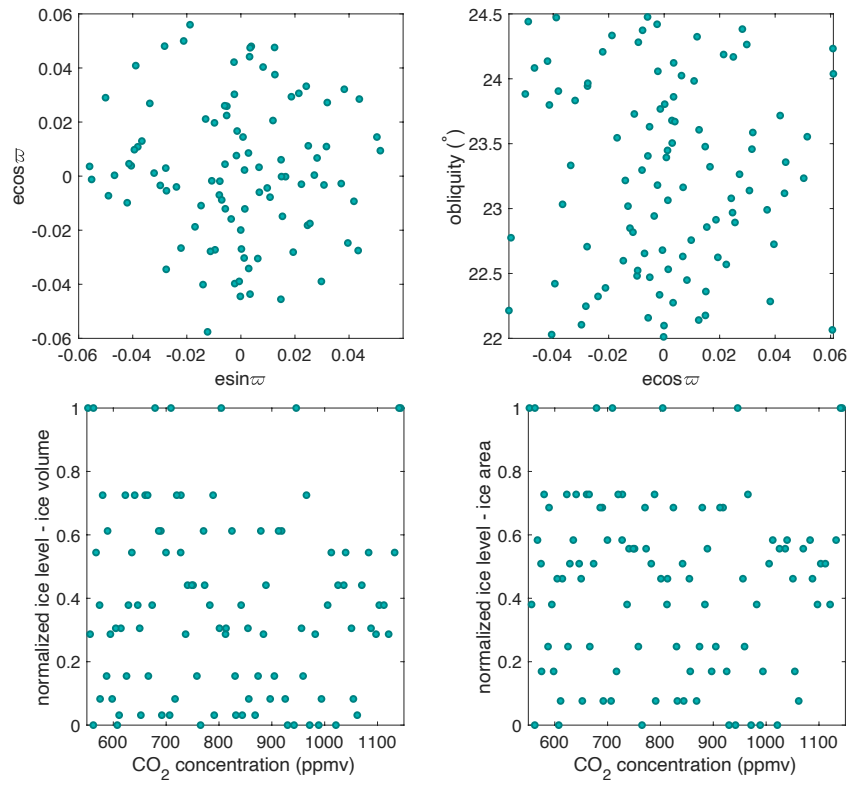
775 Figure 5: Latin hypercube model design of EMULATOR_12a showing the values for the orbital forcing, carbon dioxide forcing and ice sheet parameter forcing (defined by ice volume). Note that each dot represents one experiment from a total of 100 experiments.
