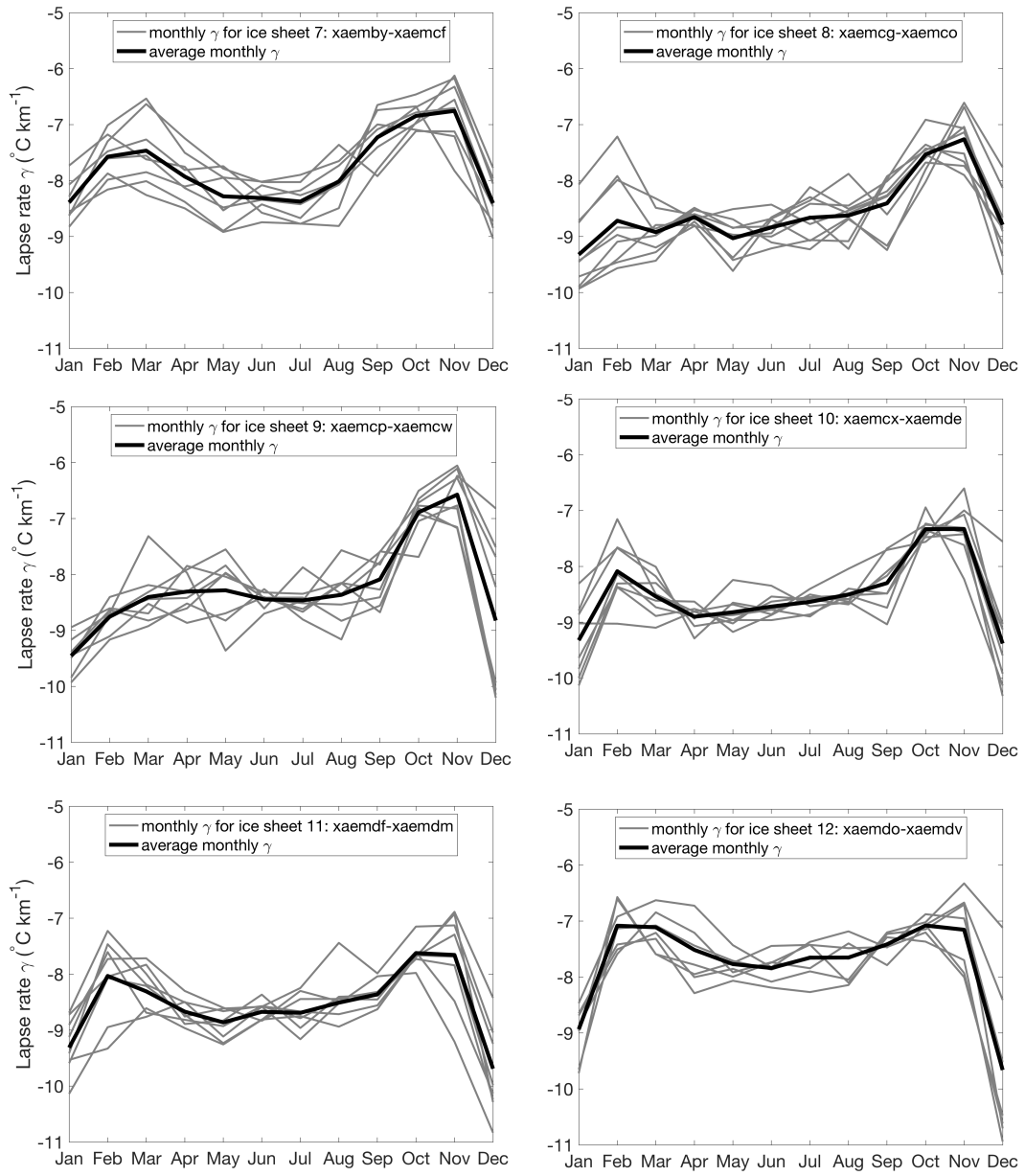
Figure A1: Monthly average lapse rate for the twelve different ice sheet geometries calculated from the 100 GCM runs for EMULATOR_12b.
