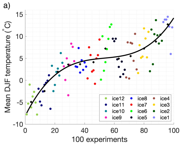
Figure 6: Mean austral summer temperature (December, January, February) for (a) EMULATOR_12a and (b) EMULATOR_20. Each dot represents the output from one GCM run. The output is grouped for each input ice sheet geometry. The mean austral summer for each input ice sheet geometry is given by the black cross and the best fit is given by the black line.
