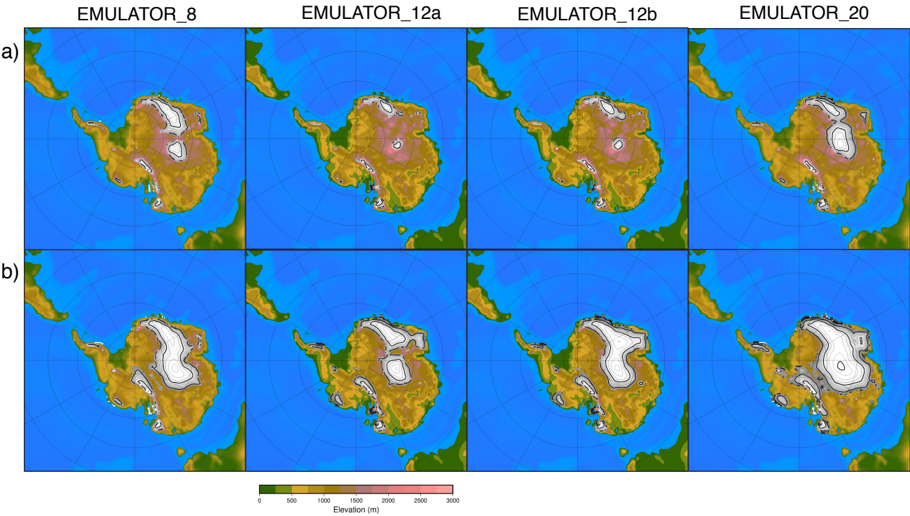
890 Figure A5: Snapshots of the ice sheet geometry after (a) 47,000 years and (b) 60,000 years (corresponding to the temperature fields in Fig. 10) for EMULATOR_8, EMULATOR_12a, EMULATOR_12b and EMULATOR_20 calibrated with ice volume.
