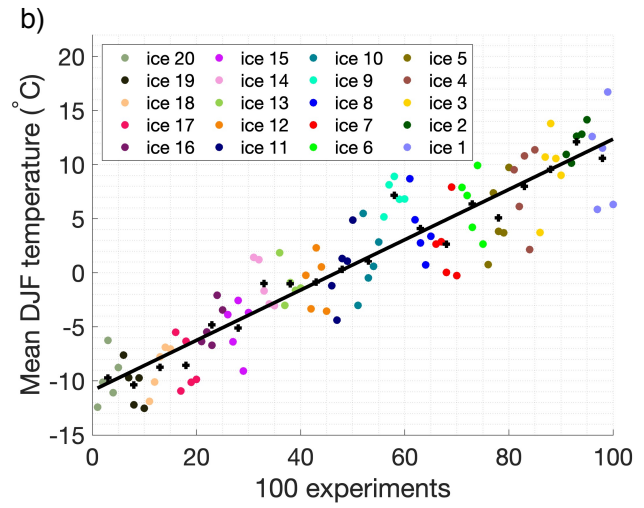
Figure 6: Mean austral summer temperature (December, January, February) for (a) EMULATOR_12a and (b) EMULATOR_20. Each dot represents the output from one GCM run. The output is grouped for each input ice sheet geometry. The mean austral summer for each input ice sheet geometry is given by the black cross and the best fit is given by the black line.
