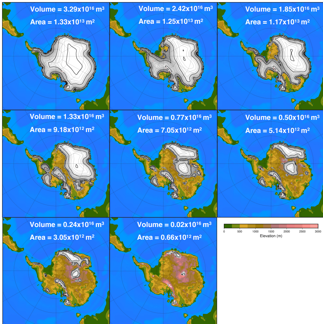
Figure 3: Eight different ice sheet geometries with their respective ice sheet volume and ice sheet area as input to 755 EMULATOR_8. Ice sheet contour lines are given each 250 m and thick contour lines each 1000 m.
