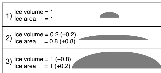
815 Figure 11: Three schematic ice sheet geometries with corresponding ice sheet volume and ice sheet area (normalized units).
