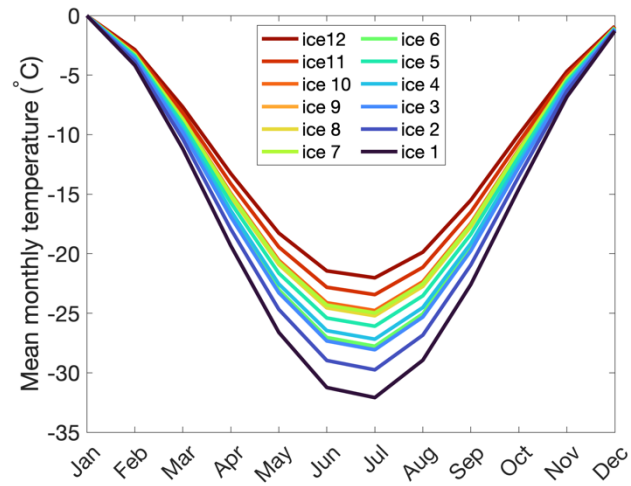
Figure 17: (a) Mean monthly temperature for each of the 12 input ice sheet geometries over the Antarctic continent.
