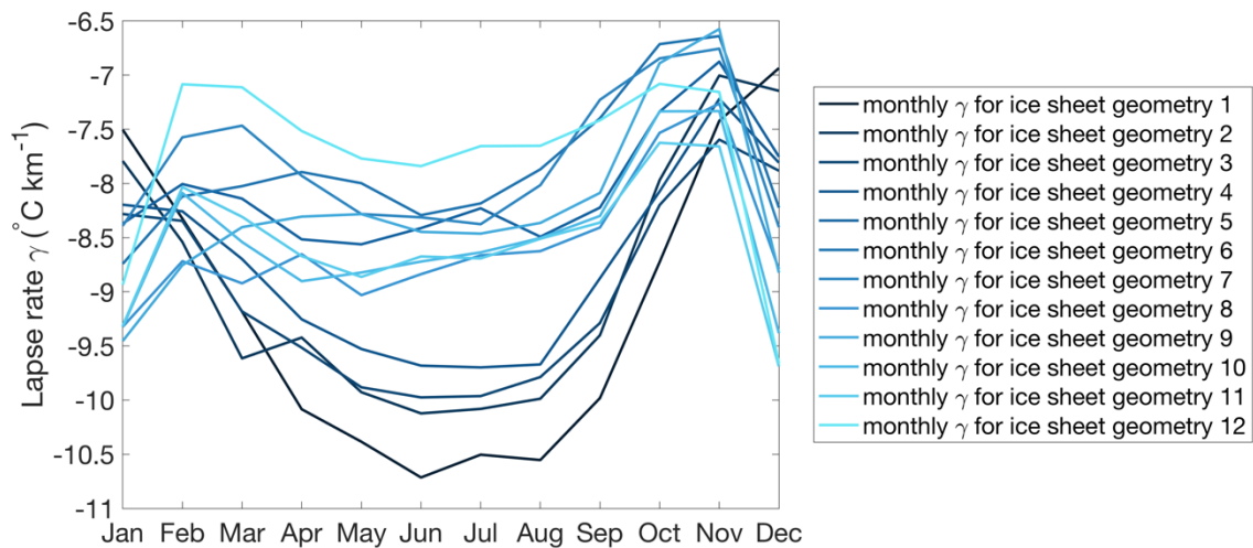
Figure 15: Average monthly near-surface lapse rate in HadSM3 over the Antarctic continent for each of the 12 ice sheet geometries. Ice sheet geometry 1 is the largest ice sheet and ice sheet geometry 12 is the smallest ice sheet geometry.
