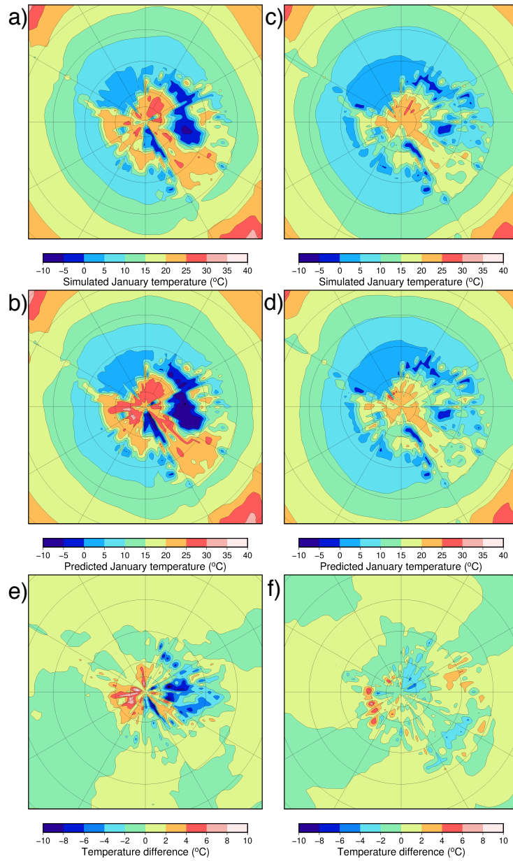
Figure 8: (a) Simulated and (b) predicted (with a leave-one-out experiment) January temperatures for the emulator showing a very poor- performing experiment ( xaemdk ) using EMULATOR_12b. (c) Simulated and (d) predicted January temperatures for a well-performing experiment ( xaemdv ) using EMULATOR_12b. Difference between the simulated and predicted temperature fields for (e) experiment xaemdk and (f) experiment xaemdv .
