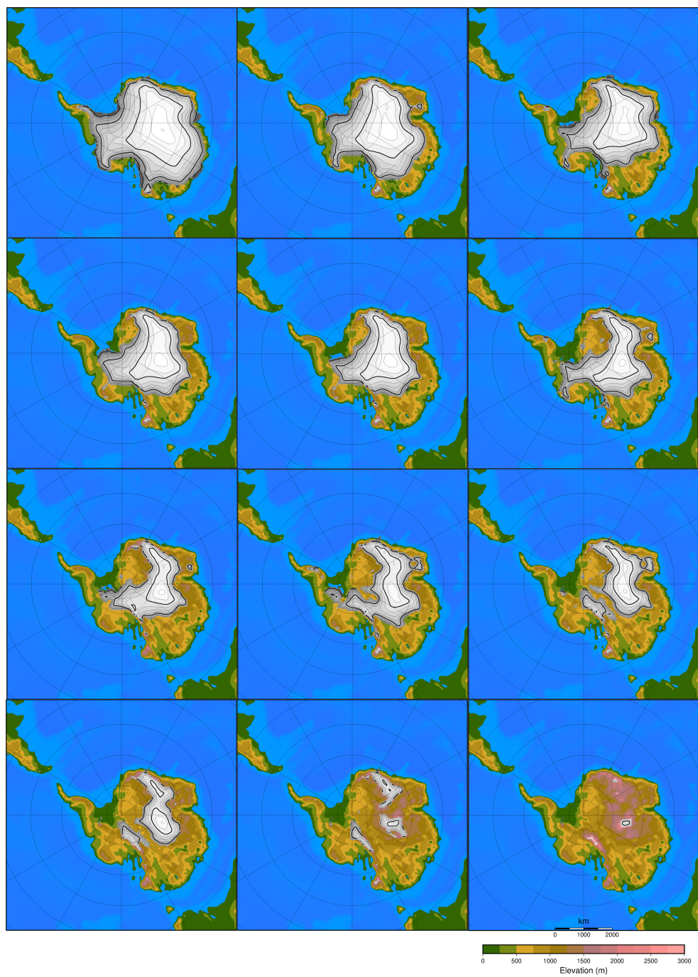
Figure A3: 12 ice sheet geometries as input to EMULATOR_12b.
