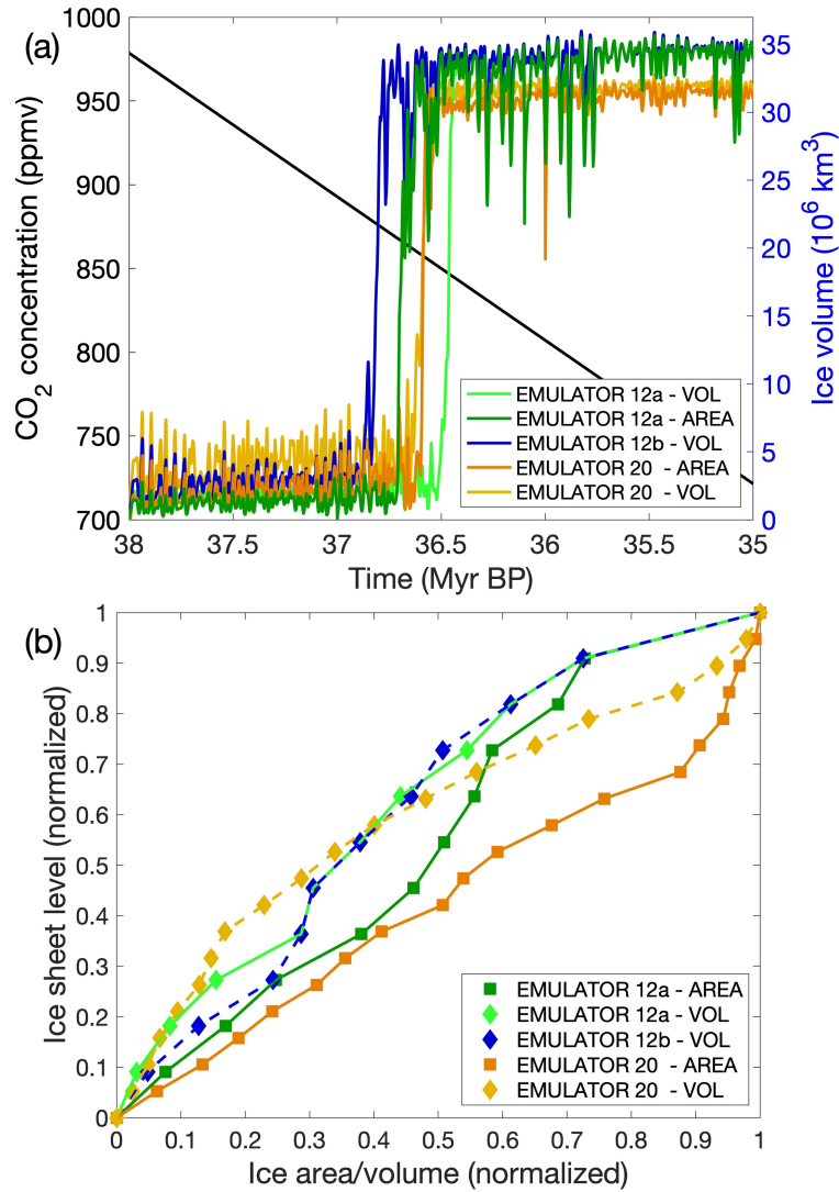
Figure 19: (a) Ice sheet evolution for EMULATOR_12a tuned on ice area, EMULATOR_12a tuned on ice volume and 865 EMULATOR_12b tuned on ice volume. (b) Comparison of the input ice sheet geometry spacing when looking at ice area and ice volume for EMULATOR_12a and EMULATOR_12b.
