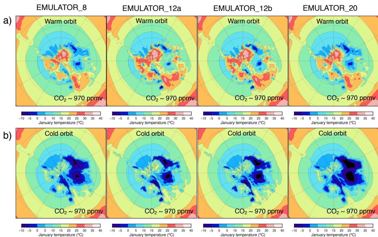
810 Figure 10: Simulated January temperature (°C) with the different emulators starting from an ice-free continent at 38 Ma after (a) 48,000 years (the first high insolation maximum) and after (b) 60,000 years (the first high insolation minimum) for the ice sheet parameter defined as ice volume.
