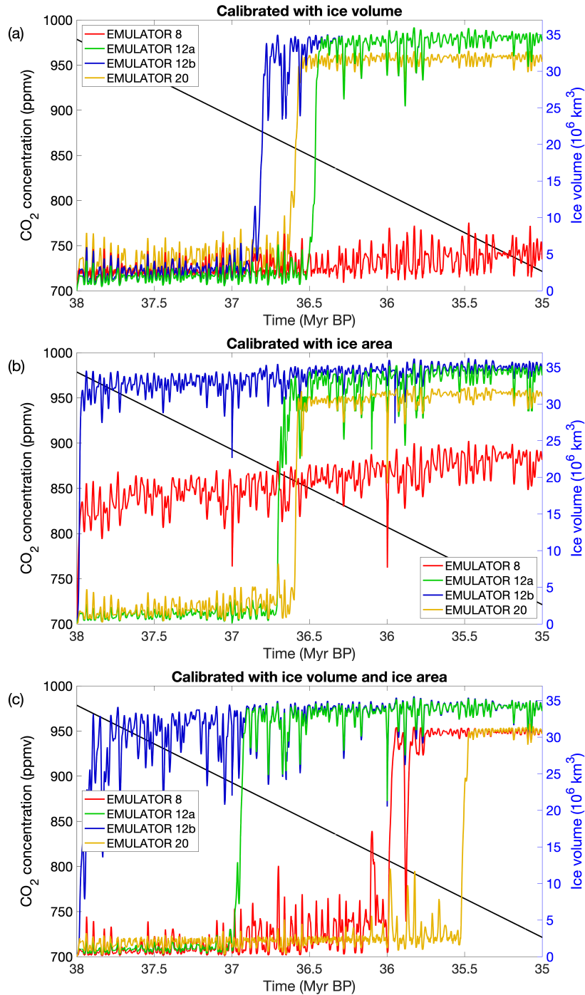
805 Figure 9: Ice sheet evolution during a 3 million year period forced by the orbital parameters from Laskar et al. (2004) and linearly declining \text{CO}_2 concentrations from \sim 980 ppm to \sim 720 ppm. Ice sheet evolution for the four different emulators calibrated based on (a) ice volume, (b) ice area and (c) both ice volume and ice area.
