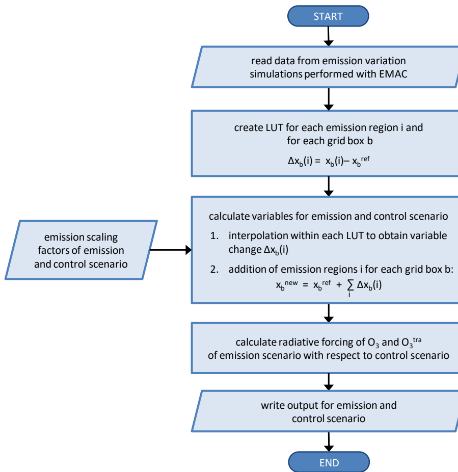
Figure 4. Workflow of TransClim showing the main calculation steps. For a defined emission and control scenario, TransClim computes the resulting climate effect such as the stratosphere-adjusted radiative forcing at top of the atmosphere.
