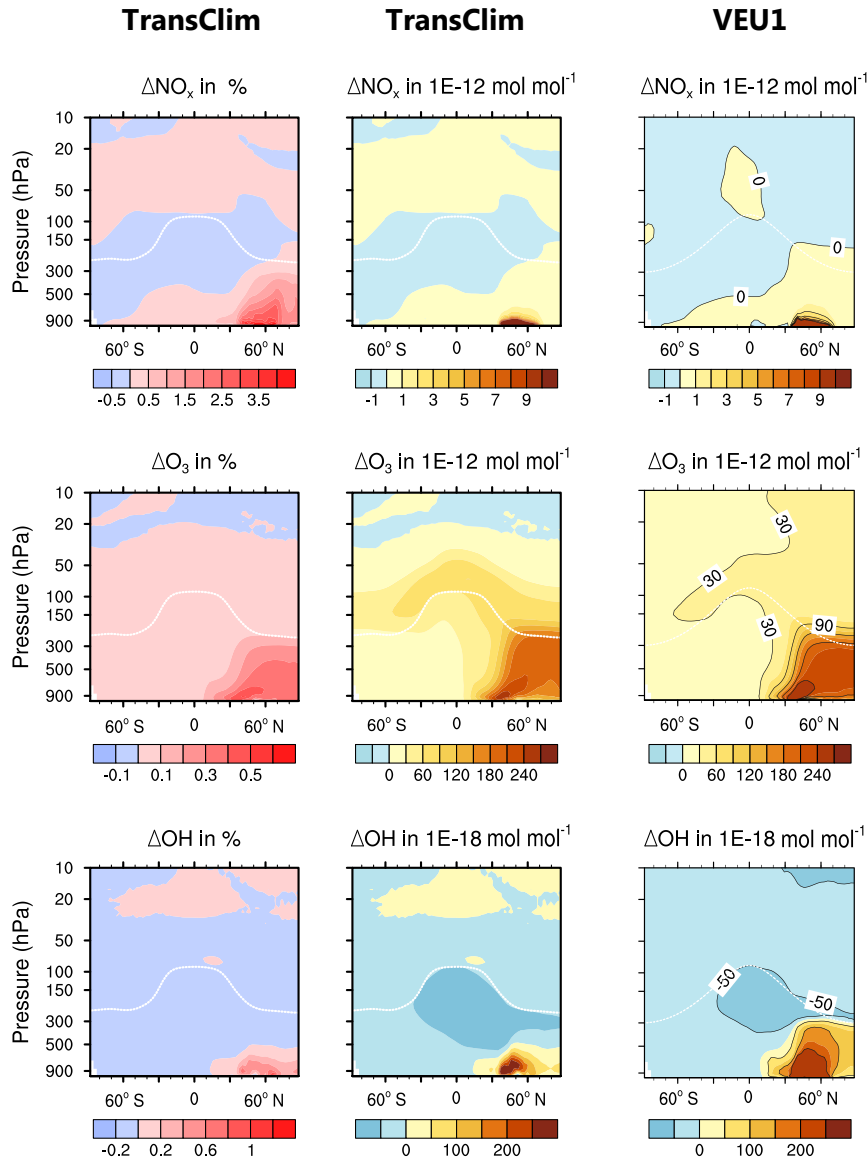
Figure 8. Zonal mean of relative and absolute NO x , O 3 and OH change caused by European road traffic emissions for the year 2030. Simulations performed with TransClim and EMAC (conducted within VEU1) are compared. The first and second columns show the relative and absolute changes simulated with TransClim. The third column shows the absolute changes simulated with EMAC (taken from fig. 6 in Hendricks et al. (2018)). The white line indicates the tropopause.
