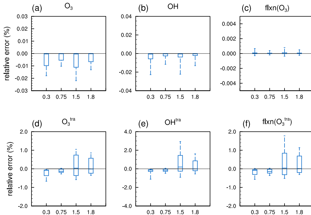
Figure 7. Box plot of the relative errors between the simulations performed with TransClim and EMAC for the different emission scaling. The road traffic emissions in North America are scaling with 0.3, 0.75, 1.5 and 1.8. The whiskers show the 5th and 95th percentiles. The relative errors for the variables O_3 (a), OH (b) and flxn(O_3) (c) as well as the contribution to O_3^{tra} (d), OH^{tra} (e) and flxn(O_3^{tra}) (f) are shown. For O_3 and O_3^{tra} , the relative errors of the tropospheric columns are shown. For OH and OH^{tra} , the deviations of the tropospheric means are displayed. For flxn(O_3) and flxn(O_3^{tra}) , the values at top of the atmosphere are taken into account.
