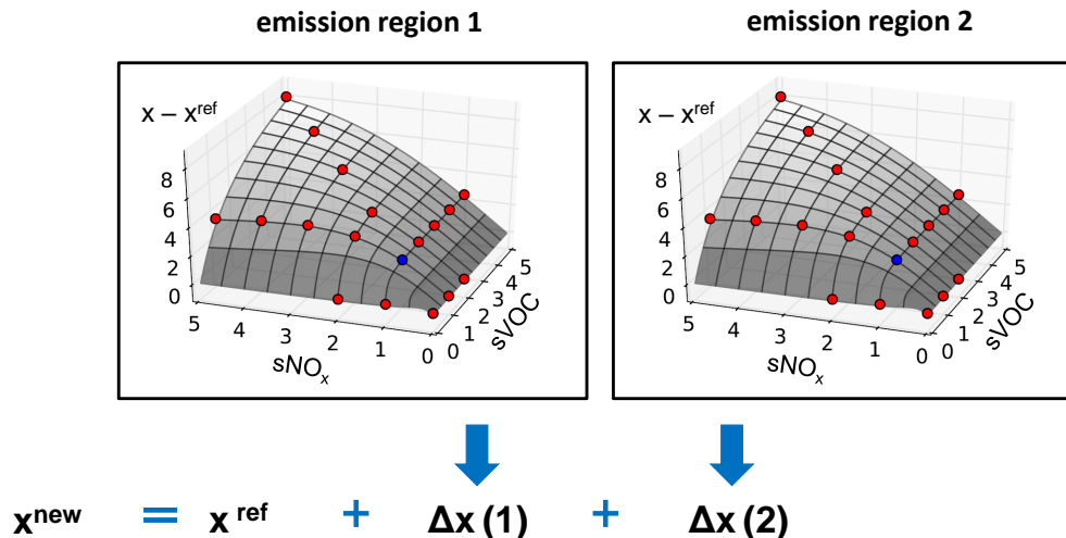
Figure 2. Sketch of interpolation algorithm used by TransClim. For each emission region, a LUT contains the change in variable x ( x - x^{ref} ) and the emission scaling factors for \text{NO}_x , VOC and CO emissions ( s\text{NO}_x , s\text{VOC} , s\text{CO} ). In the figure, only s\text{NO}_x and s\text{VOC} are displayed. The blue dot indicates the reference simulation ( s\text{NO}_x = 1 , s\text{VOC} = 1 ). The red dots indicate the emission variation simulations (note that the red dots are just a sketch and do not represent the actual emission scaling, see table 2). After linearly interpolating within the LUT for each emission region i , the resulting changes \Delta x(i) are added to reference x^{ref} . This procedure is performed for every grid box or for tropospheric or global means.
