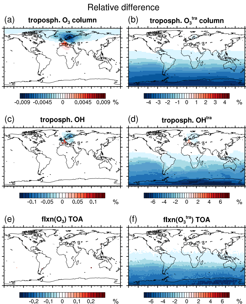
Figure 5. Relative difference between TransClim and EMAC simulation. Ozone ( O_3 ), hydroxyl radical (OH) and ozone net radiative fluxes ( flxn(O_3) ) as well as the contribution to ozone ( O_3^{tra} ), to hydroxyl radical ( OH^{tra} ) and to ozone net radiative fluxes ( flxn(O_3^{tra}) ) are shown. For O_3 and O_3^{tra} , the relative difference of the tropospheric columns are shown ((a) and (b)). For OH and OH^{tra} , the deviations of the tropospheric means are displayed ((c) and (d)). The values at top of the atmosphere (TOA) are shown for flxn(O_3) and flxn(O_3^{tra}) ((e) and (f)).
