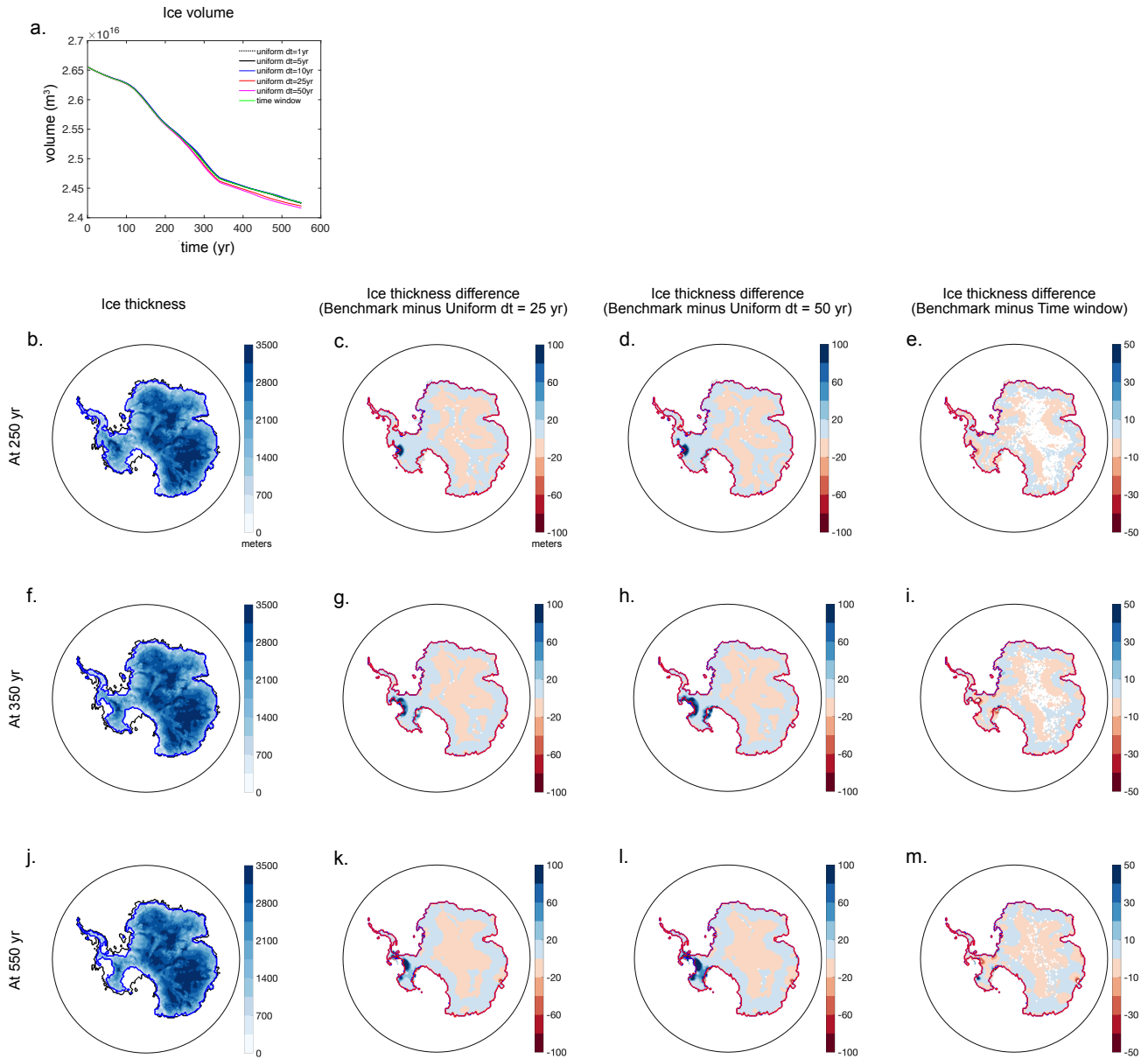
Figure 9. Changes in Antarctic Ice Sheet volume and thickness from coupled ice-sheet – sea-level simulations over 550 years adopting a RCP 8.5 scenario from DeConto et al. (2021). (a) AIS volume variations through 550 yr from simulations that incorporate uniform (standard) coupling interval of 1 yr (benchmark), 5, 10, 25 and 50 yr and that incorporate the time window profile derived in Fig. 7. (first column) ice thickness modelled in the benchmark simulation, differences in ice thickness between the benchmark and the standard simulations that incorporate coupling interval of (second column) 25 yr and (third column) 50 yr and that incorporates (fourth column) the time
