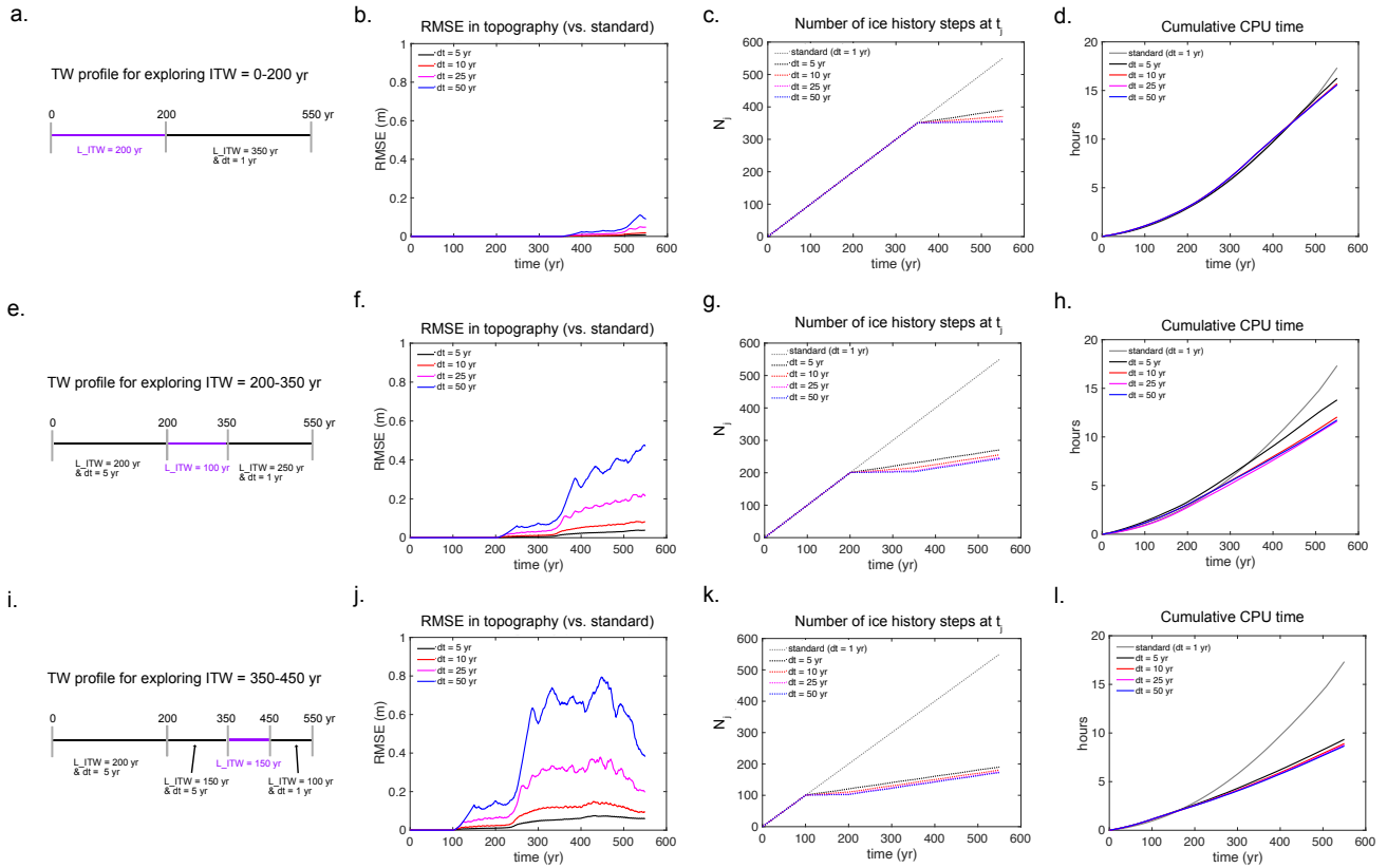
Figure 7: Time window profiles, RMSE in predicted topography, the number of loading events considered at t_j (nsteps, N_j ) and the total CPU times it has taken for the sea-level model to perform calculations at time step t_j in the 550 yr-long future AIS-scenario simulations. Results from the simulations in which we explore the internal time windows that cover the periods between (a-d) 0-200 yr, (e-j) 200-350 yr and (i-l) 350-450 yr. Note that the standard simulation for the AIS scenario assigns a uniform time step size of 1 yr throughout the simulation.
