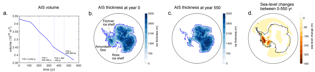
Figure 6. Changes in Antarctic Ice Sheet volume and thickness over 550 years from DeConto et al. (2021) and associated total sea-level changes predicted in a standalone (uncoupled) sea-level simulation. (a) AIS volume variations through 550 yr. Vertical dashed lines mark the internal time windows. (b, c) Snapshots of ice thickness (blue) and grounding lines (blue contour lines) at (b) 0 yr and (c) 550 yr. (d) Total sea-level changes between 0-550 yr associated with the ice loading changes between 0-550 yr. Note that the regions (in yellow and red) that show negative sea-level changes are where sea level has fallen because of solid Earth uplift and the drawdown of sea surface height associated with ice mass loss. Red line represents a cross section perpendicular to a grounding line in the West Antarctic region where the most intense sea-level change (fall) happens (see also Fig. 8).
