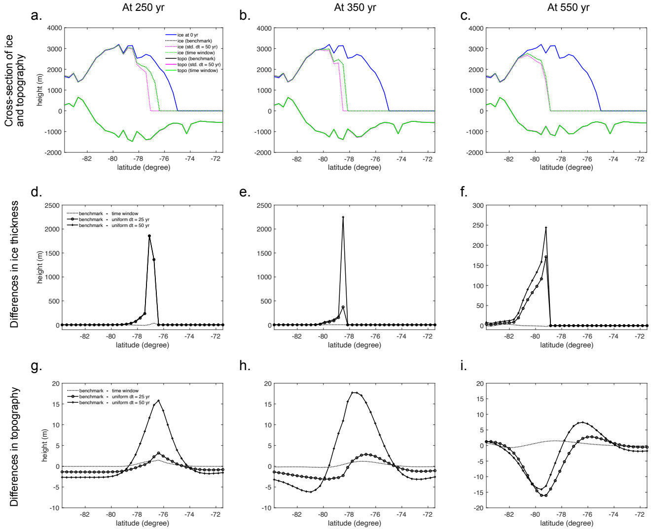
815 Figure 10. Predicted elevations of ice sheet and topography across the grounding line in the West Antarctic region (red line shown in Fig. 6g) in coupled ice-sheet – sea-level simulations with and without the time window algorithm and the differences in the predicted ice thickness and topography. (a-c) Cross-section of ice thickness and topography at (a) 250 yr, (b) 350 yr and (c) 550 yr. Blue lines indicate ice profile at the beginning of the simulation. Black lines show results from the benchmark standard coupled simulation that incorporates temporal resolution of 1 yr, magenta lines show results from the standard simulation with dt = 50 yr and green lines show results from 820
