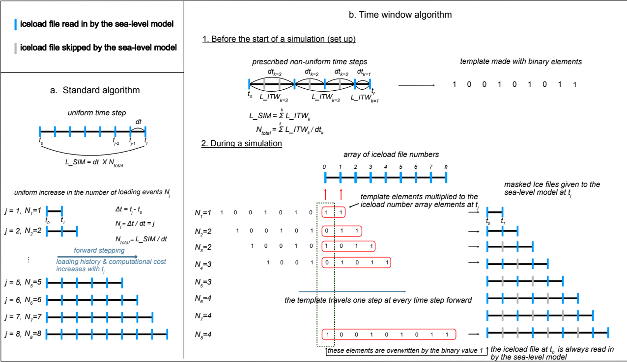
Schematic representation of forward sea-level model algorithms
