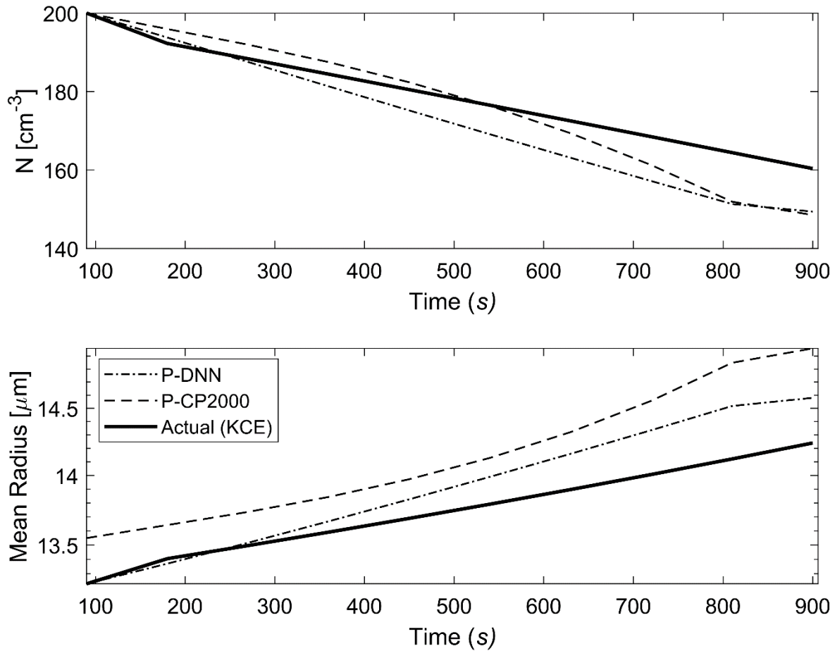
435 Figure 9: Drop number concentration (top) and mean radius (bottom) comparison with KCE. The concentration and mean radius of KCE were obtained by integrating the drop number concentration spectra for the corresponding moment order (0 and 1 respectively). The data points are plotted every 60 s.
