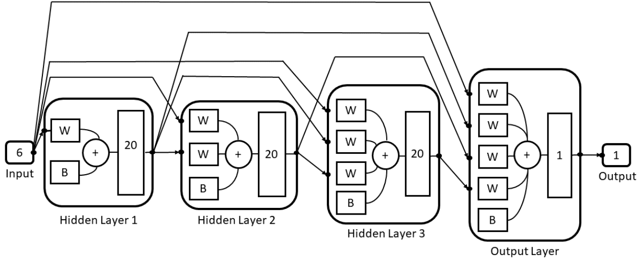
215 Figure 2: Schematic representation of the architecture of the trained neural network used to calculate the total moment tendencies. The neural network receives six inputs and then processes them by means of three hidden layers of 20 neurons each, and an output layer with a single neuron and one output value.
