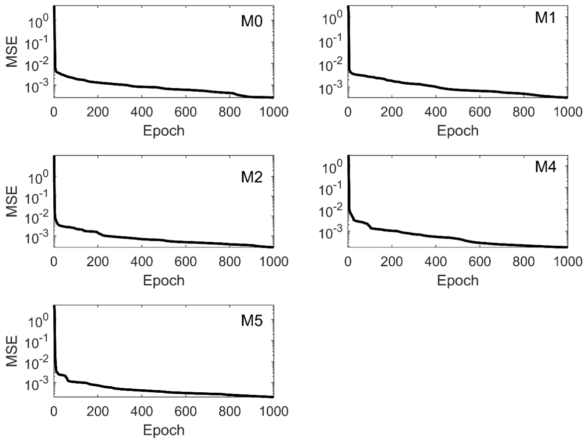
Figure 5: Performance training records of total moment tendencies for the moments from order 0 to 5 (3 rd order is excluded). The shown data corresponds to the total moment tendencies obtained from the trained neural networks, with input values and reference targets taken from the validation data set. The performance measure is the Mean Square Error (MSE).
