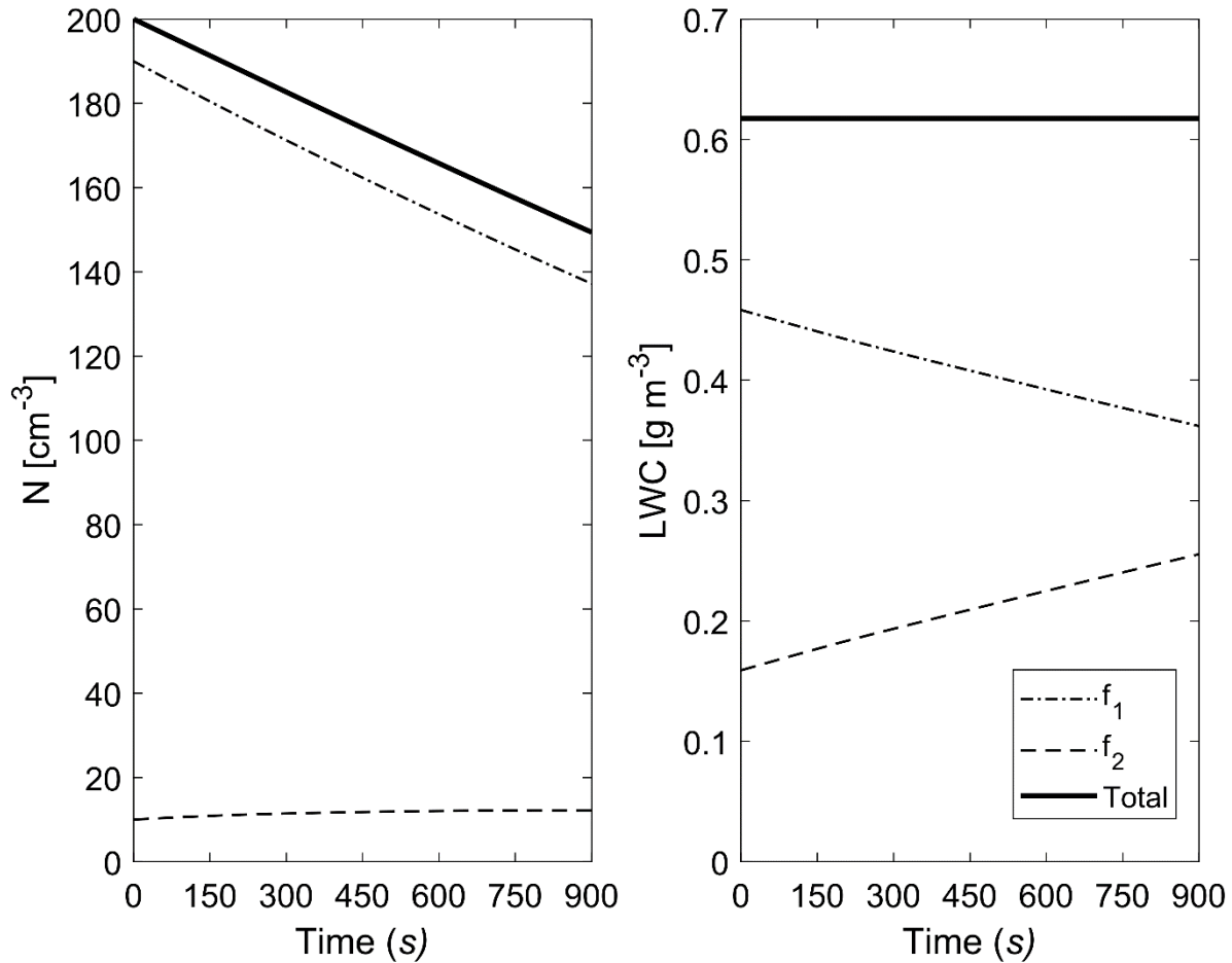
455 Figure 10: Evolution of drop number concentration N (left) and liquid water content LWC (right) of the individual distributions that conform P-DNN. The liquid water content of each of the distribution functions ( f_1 and f_2 ) were obtained from the corresponding moment (order 3) calculated from eq. (4). The combined (total) values of the variables are also shown and were calculated from eq. (5).
