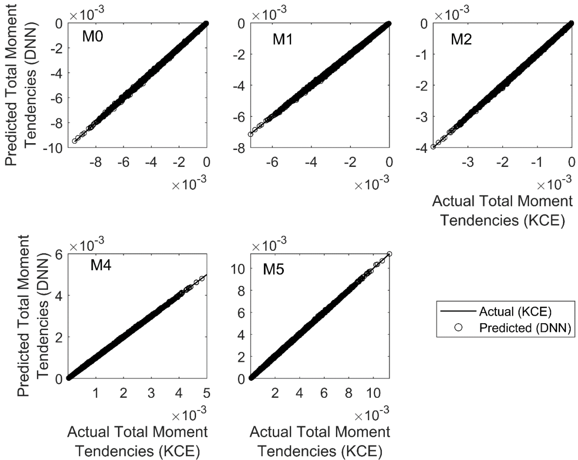
305 Figure 6: Regression plots for the five DNN trained. It is a comparison between the outputs obtained from evaluating the trained neural networks using the test inputs and the targets from the validation data set corresponding to each of the total moment tendencies obtained from eq. (13). The y axis varies for each subplot because the plotted data is non-normalized.
