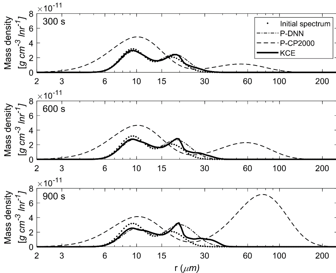
380 Figure 7: Mass density functions from P-DNN, P-CP2000 and KCE. The represented times are 300 s, 600 s and 900 s, from top to bottom. Equation (16) was used to transform the drop number concentration spectra from P-DNN to the mass density spectra.
