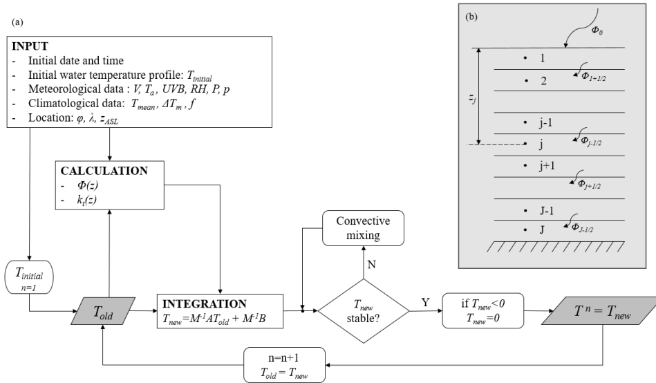
375 Figure 4 Model configuration. Panel (a) shows a schematic overview of the model workflow. The input consists of the initial time and date, the initial water temperature profile T_{initial} , meteorological data (wind speed, air temperature, UVB radiation, relative humidity, precipitation, and atmospheric pressure), climatological data (mean annual air temperature, mean annual temperature range between the daily air temperature maximum and minimum, and mean monthly cloud cover), and location data (location latitude, longitude, and altitude above sea level). Panel (b) shows the layer setup. Points from 1 to J indicate the integration points where water temperatures are calculated, and z_j is the depth of the j-th point. The horizontal lines indicate boundaries between layers, \Phi_{j+1/2} are the heat fluxes across the layer boundaries, and \Phi_0 is the net surface heat flux. 380
