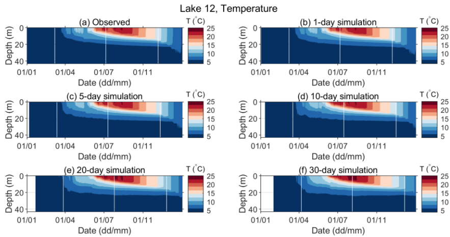
515 Figure 7 Observed (a) and predicted (b-f) water temperatures of Lake 12 for different simulation lengths for 2019. Periods with missing data are seen as white vertical stripes.
