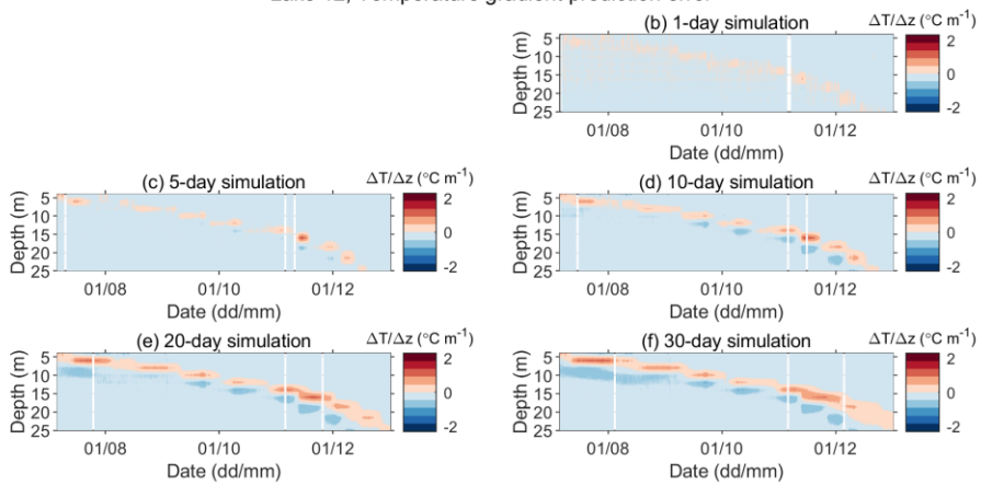
Figure A6 Error in the predicted vertical gradient of water temperature ( P_i - O_i ) in Lake 12 for different simulation lengths in the period between 06 July 2019 and 31 December 2019. Panel (a) is omitted so that the panels' positions for different simulation lengths correspond to those in Fig. 5.
