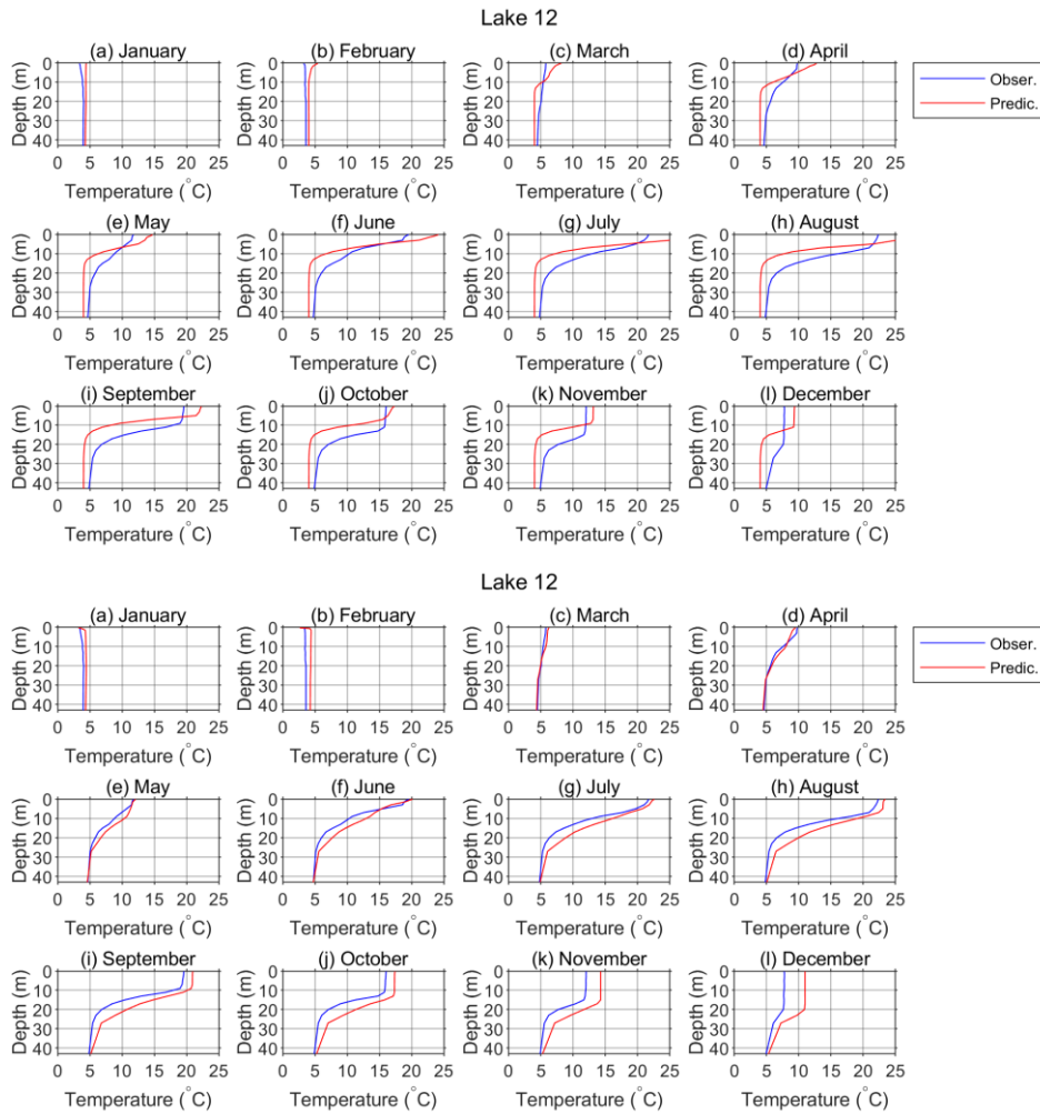
Figure 1413 Monthly means of the observed (blue) and predicted (red) water temperature vertical profiles for Lake 12 in 2019. Predicted temperatures are obtained by a single yearlong simulation run initiated on 1 January 2019.
