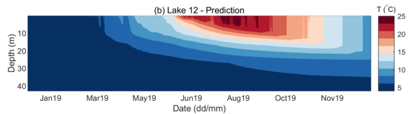
Figure 12 Observed (a) and predicted (b) water temperature for Lake 12 in 2019. The predicted temperature is obtained by a single yearlong simulation run initiated on 1 January 2019.
