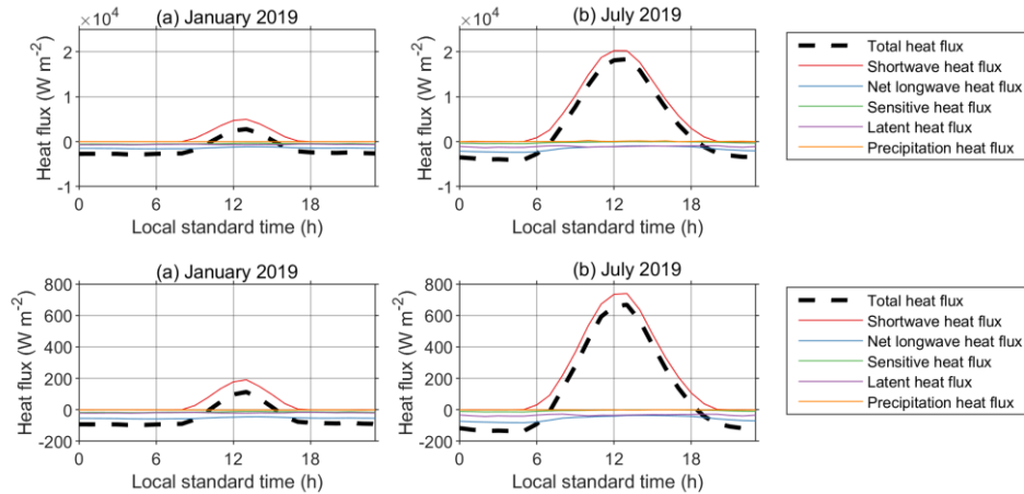
Figure 5 Modeled mean diurnal variations in the heat flux at the surface of Lake 12 for January (a) and July 2019 (b).
