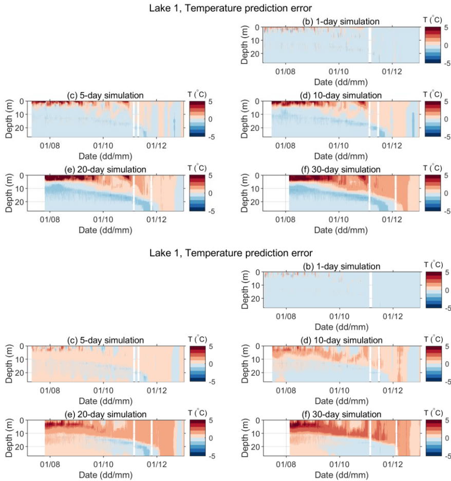
Figure A1 Error in the predicted water temperature ( P-O_i ) for Lake 1 for different simulation lengths for the period between 06 July 2019 and 04 November 31 December 2019. Panel (a) is omitted so that the panels' positions for different simulation lengths correspond to those in Fig. 6.
