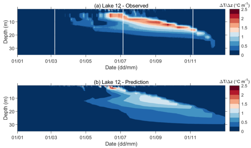
575 Figure 13 Observed (a) and predicted (b) water temperature gradient for Lake 12 in 2019. The predicted temperature gradient is obtained by a single yearlong simulation run initiated on 1 January 2019.
