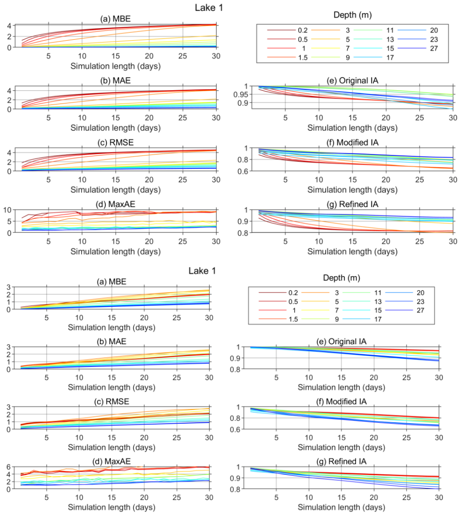
540 Figure 9 Model performance parameters for Lake 1. (calculated for all the periods with necessary data available: 6.7.-31.12.2019. and 2.7.-30.9.2020.)
