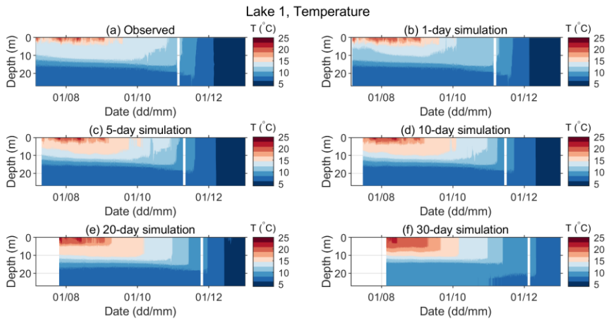
Figure 6 Observed (a) and predicted (b-f) water temperatures of Lake 1 for different simulation lengths in the period between 06 July 2019 and 04-31 November-December 2019. Periods with missing data are seen as white vertical stripes.
