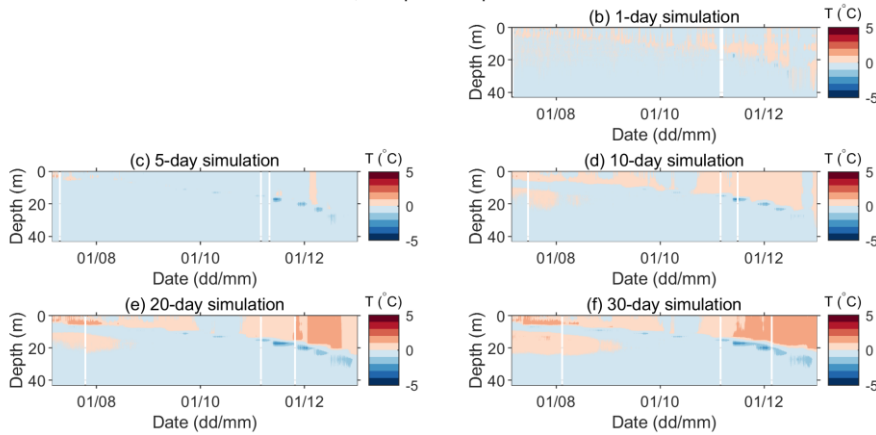
Figure A2 Error in the predicted water temperature ( P-O ) for Lake 12 for different simulation lengths in the period between 06 July 2019 and 31 December 2019. Panel (a) is omitted so that the panels' positions for different simulation lengths correspond to those in Fig. 7.
