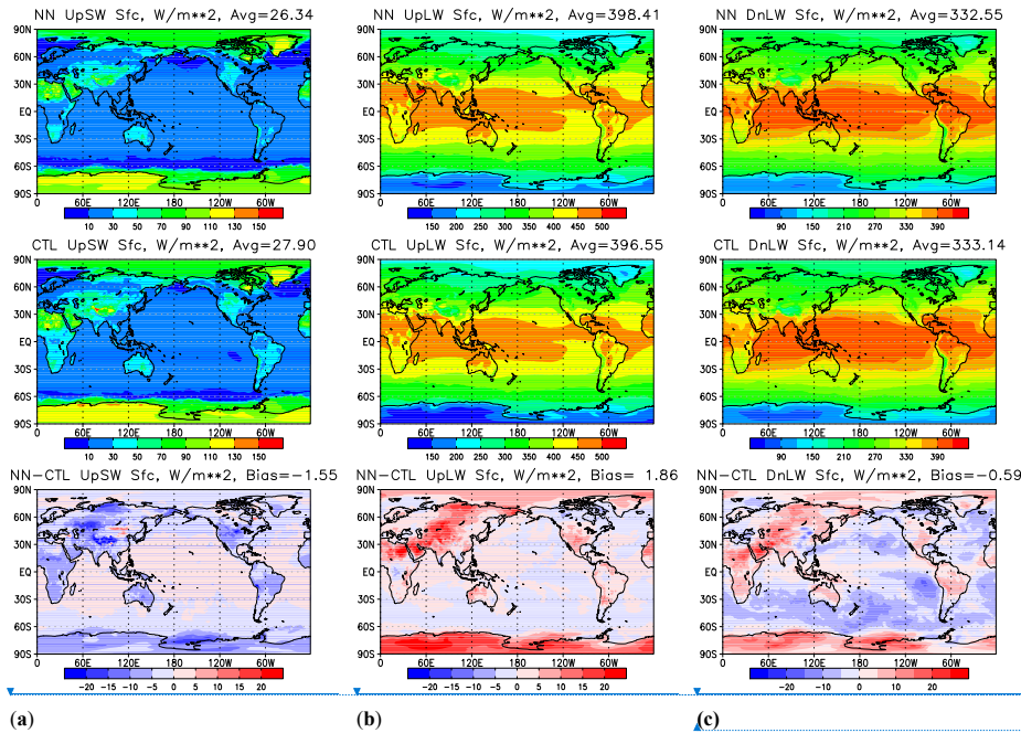
375 Figure 3. Time means over 12-month worth of model output covering 2/1/2018-2/1/2019 for: (a) Upwelling SW radiation at the surface; (b) Upwelling LW radiation at the surface; (c) Downwelling LW radiation at the surface. Upper row – results produced by HGFS, middle – by GFS, and the lower row the difference (HGFS – GFS).
