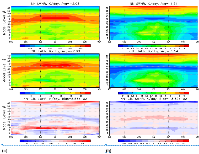
Figure 1. Zonal and time mean over 12-month worth of model output covering 2/1/2018-2/1/2019 for: (a) Long-wave heating rate, K/day; (b) Short-wave heating rate, K/day. Upper row – results produced by HGFS, middle – by GFS, and the lower row the difference (HGFS – GFS). Vertical coordinate shows model level number.
