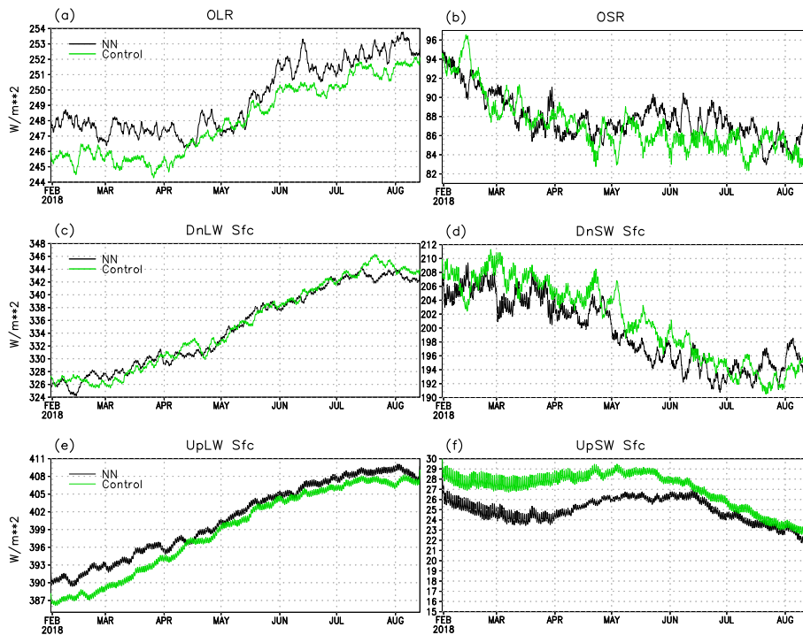
510 Figure 4. Time series of a running 10-day mean covering 2/1/2018-8/1/2018 for: (a) Outgoing LW at TOA; (b) Outgoing SW at TOA; (c) Downwelling LW radiation at the surface; (d) Downwelling SW radiation at the surface; (e) Upwelling LW radiation at the surface; (f) Upwelling SW radiation at the surface. Black curves – results produced by HGFS, green – by GFS.
