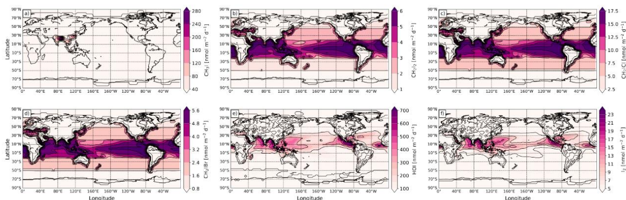
Figure 2 - Annual-mean emission fluxes of organic [ \text{CH}_3\text{I} (a), \text{CH}_2\text{I}_2 (b), \text{CH}_2\text{ICl} (c), and \text{CH}_2\text{IBr} (d)] and inorganic [ \text{HOI} (e) and \text{I}_2 (f)] iodine source gases [in \text{nmol m}^{-2} \text{d}^{-1} ] used in SOCOL-AERv2-I.
