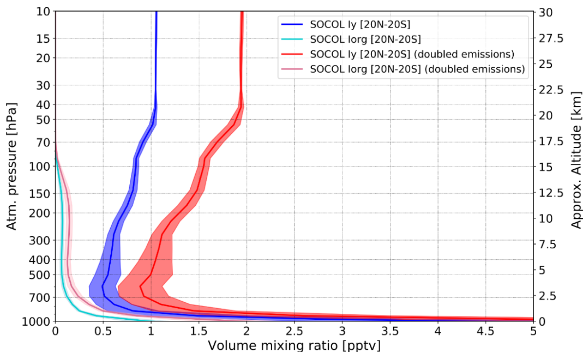
Figure 3. Modeled vertical distribution of total organic ( I_{org} ) and inorganic ( I_y ) gas-phase iodine simulated with SOCOL-AERv2-I averaged over tropics [20°N - 20°S], for 2000-2009 period and 10 ensemble members. Red curve: I_y from the experiment 2 x iodine. Blue curve: I_y from the experiment 1 x iodine. Light red and blue curves: I_{org} from 2 x iodine and 1 x iodine experiments, correspondingly. Shadings represent a standard deviation of tropical iodine [20°N - 20°S].
