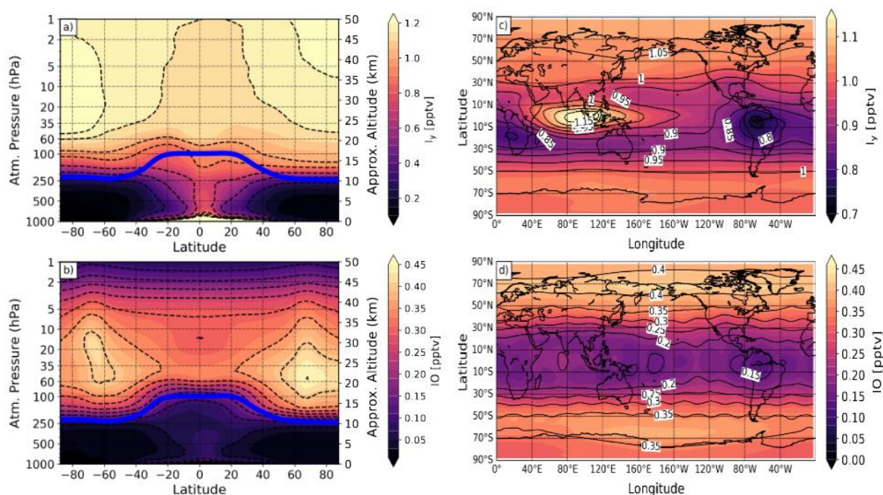
Figure 1. - Modeled vertical distribution and global map of total inorganic gas-phase iodine ( I_y ) and iodine monoxide (IO) simulated with SOCOL-AERv2-I from the experiment with present-day iodine emissions ( 1 \times iodine), averaged for 2000-2009 period and 10 ensemble members. (a+b) zonal-mean vertical distributions of I_y and IO. (c+d) global maps of I_y and IO averaged for 100-70 hPa region. Blue solid line in (a) and (b): annual mean tropopause height.
