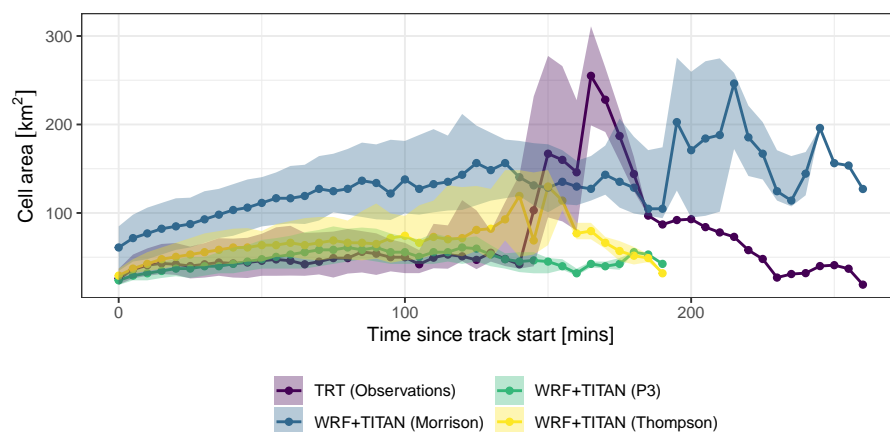
Figure 13. Area development over cell lifecycles for observations and simulation outputs. For each time since the track start, the coloured band shows the inter-quartile range of area and the joined points show the median area.
