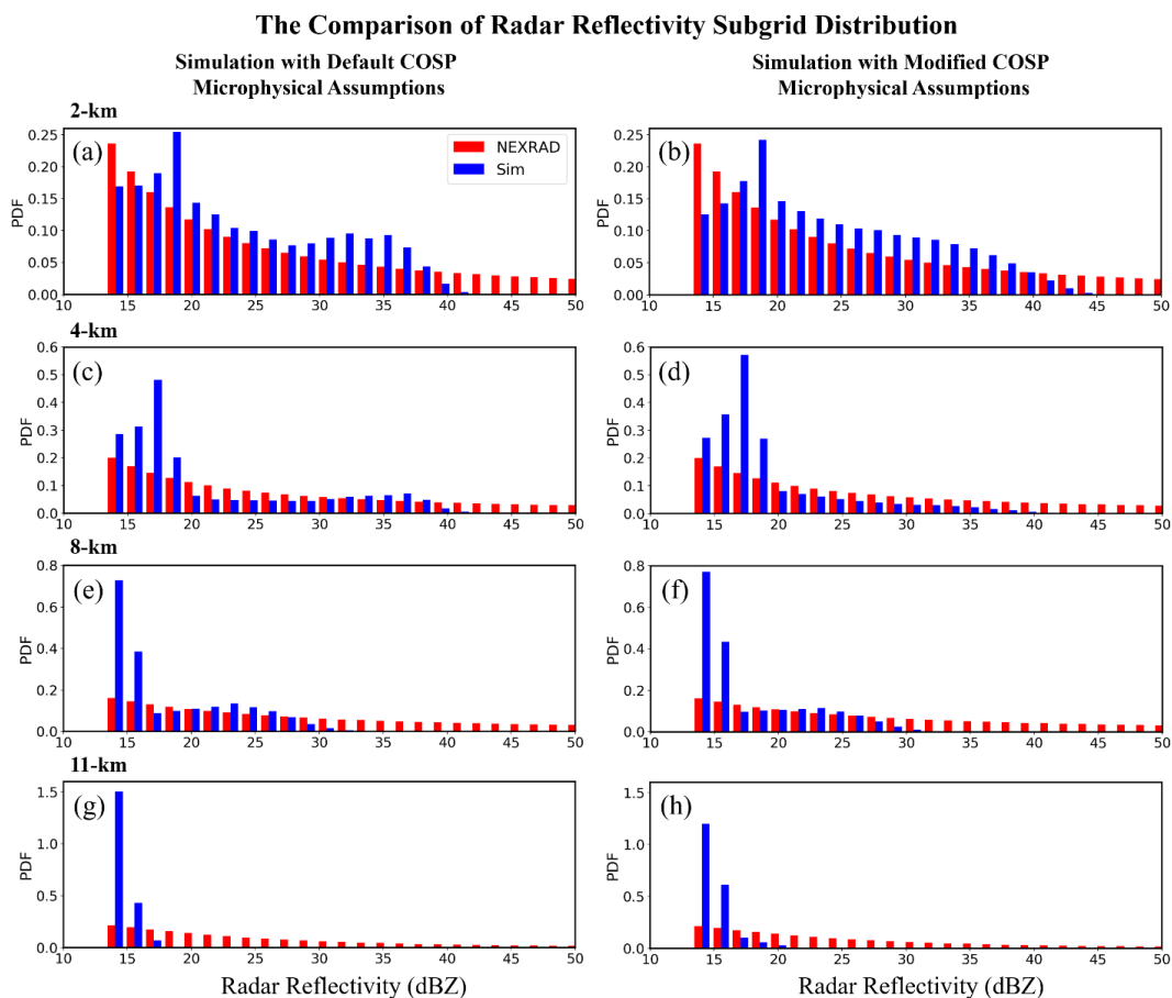
Figure 4: Comparison of radar reflectivity subgrid distribution between NEXRAD observations (red bars) and the simulations (blue bars) at the vertical levels of 2 km, 4 km, 8 km, and 11 km. Simulation results in the left and right columns are from the default microphysics assumptions in COSP and modified COSP microphysics assumptions, respectively.
