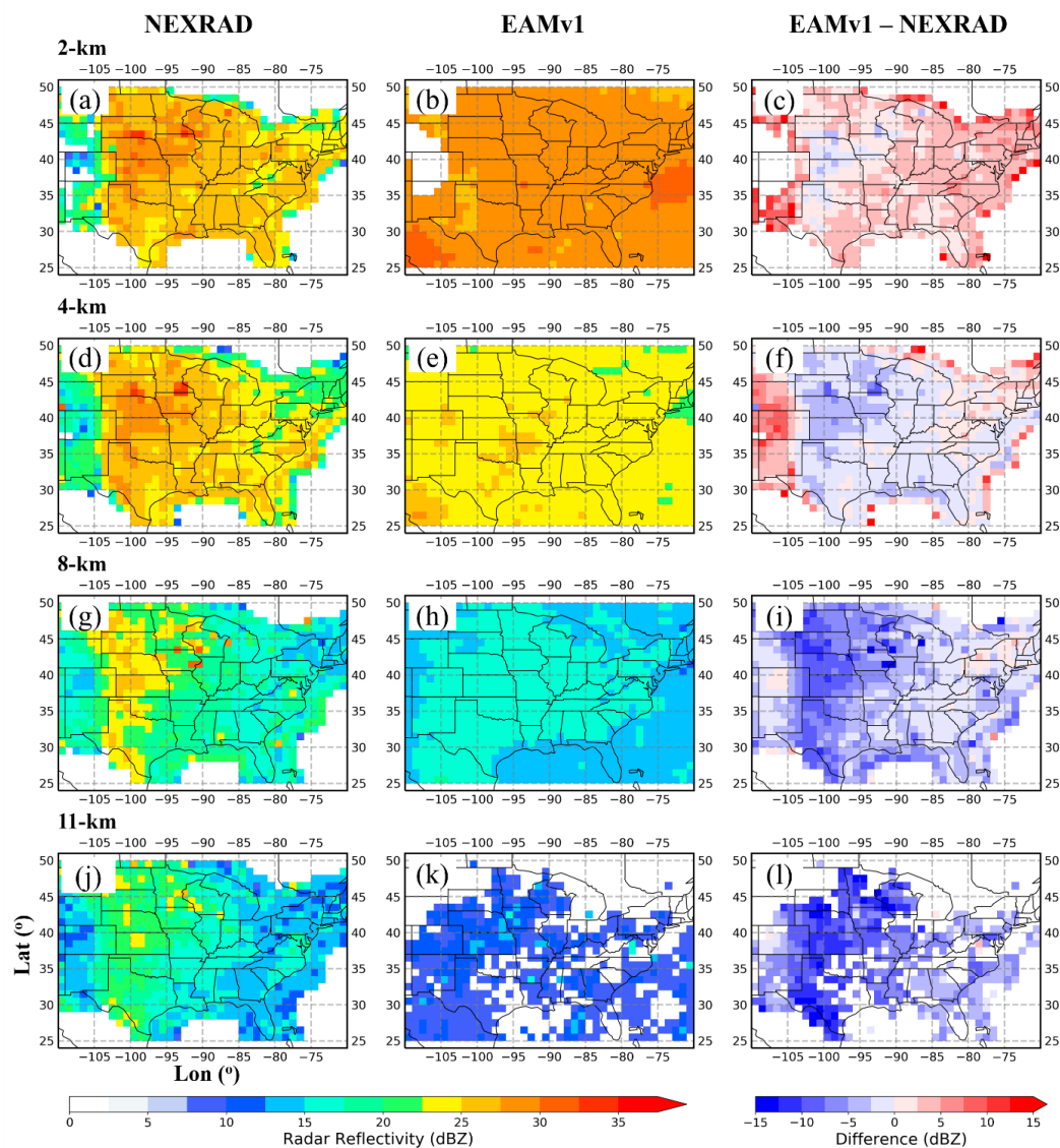
580 Figure 2: Plan view of radar reflectivity averaged from NEXRAD observations (a, d, g, j), EAMv1 simulations (b, e, h, k), as well as their absolute differences (c, f, i, l) at the level of 2-km, 4-km, 8-km, and 11-km altitude. The NEXRAD data are spatially averaged from native resolution to the model grid over 2014-2016 April-September period, and the simulation are vertically interpolated to the NEXRAD levels.
