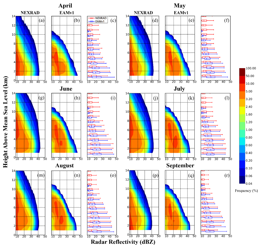
585 Figure 3: Contoured-Frequency-by-Altitude-Diagrams (CFADs) normalized by the total number of samples at all altitude levels for NEXRAD (a, d, g, j, m, p) and EAMv1 simulation (b, e, h, k, n, q) for the months from April to September averaged over 2014-2016 period. The box-whisker plots (c, f, i, l, o, r) for NEXRAD (red) and EAMv1 (blue) are calculated using 590 normalization at each individual level, where the center of the box represents the 50th percentile value, and the 25th and 75th percentiles are represented by the left and right boundary of the box, respectively. Whiskers correspond to the 5% and 95% values.
