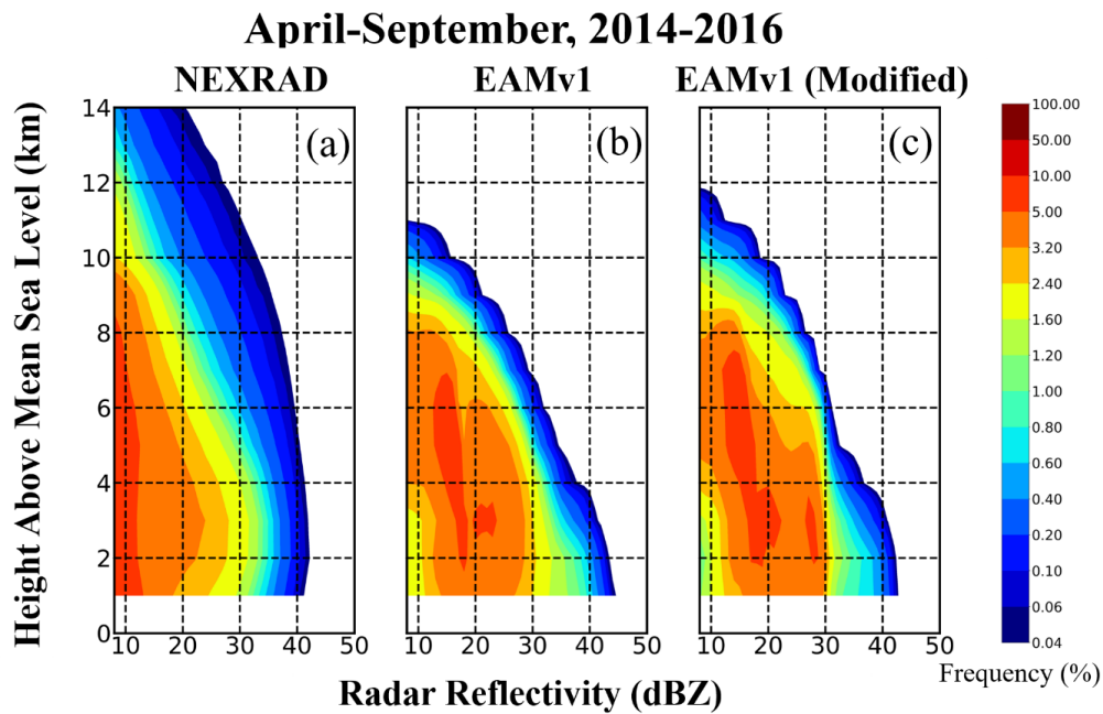
Figure 6: Comparison of Contoured-Frequency-by-Altitude-Diagrams (CFADs) for the warm seasons over 2014-2016 between (a) NEXRAD, (b) EAMv1 simulation, and (c) the EAMv1 simulation with reduced convective entrainment rate.
