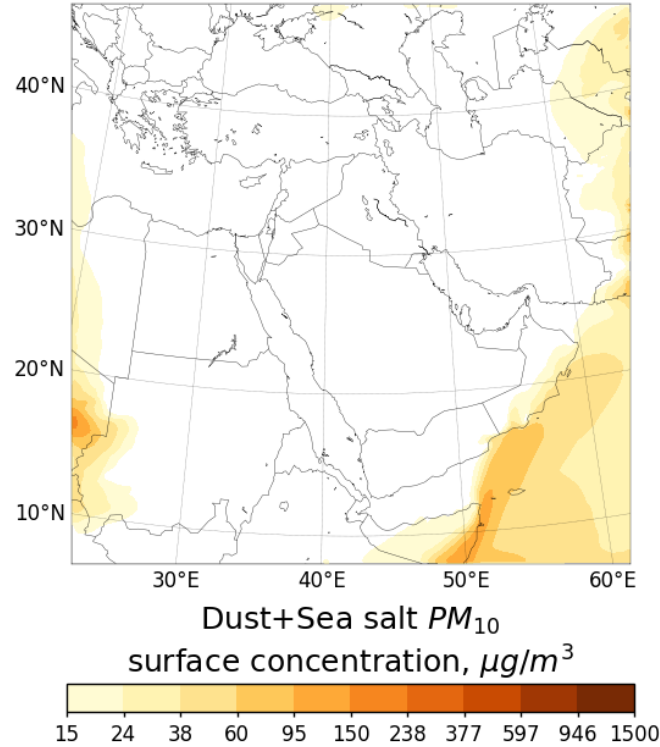
Figure 10. Effect of trans-boundary transport. Averaged dust and sea salt PM_{10} surface concentrations ( \mu g/m^3 ) obtained from WRF-Chem simulation without emission of sea salt and dust.
