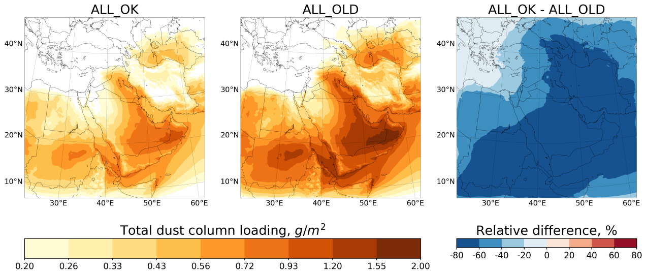
Figure 9. Averaged over the summer of 2016 total dust column loadings ( \text{g}/\text{m}^2 ) from ALL_OK and ALL_OLD runs and relative difference (%).
