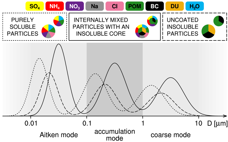
Figure 1. Schematic representation of the MADE3 submodel, as shown in Kaiser et al. (2019). The colors represent the different chemical components. The dotted, solid, and dashed lines correspond to the different mixing states (soluble, mixed, and insoluble, respectively). Grey shadings are to visually separate typical Aitken, accumulation and coarse mode sizes.
